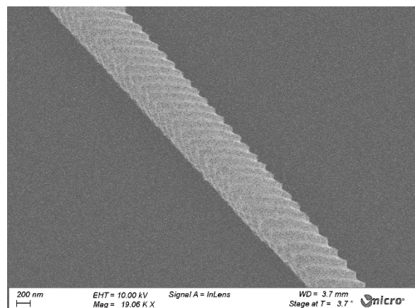
Figure: III.14 :The SEM images for VPC with triangular holes and the fabricated devices in TopoRun 2
