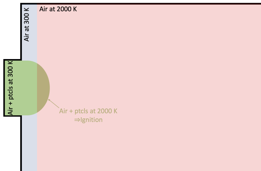
Figure 6.2 – Schematization of the ignition process used in the domain.
