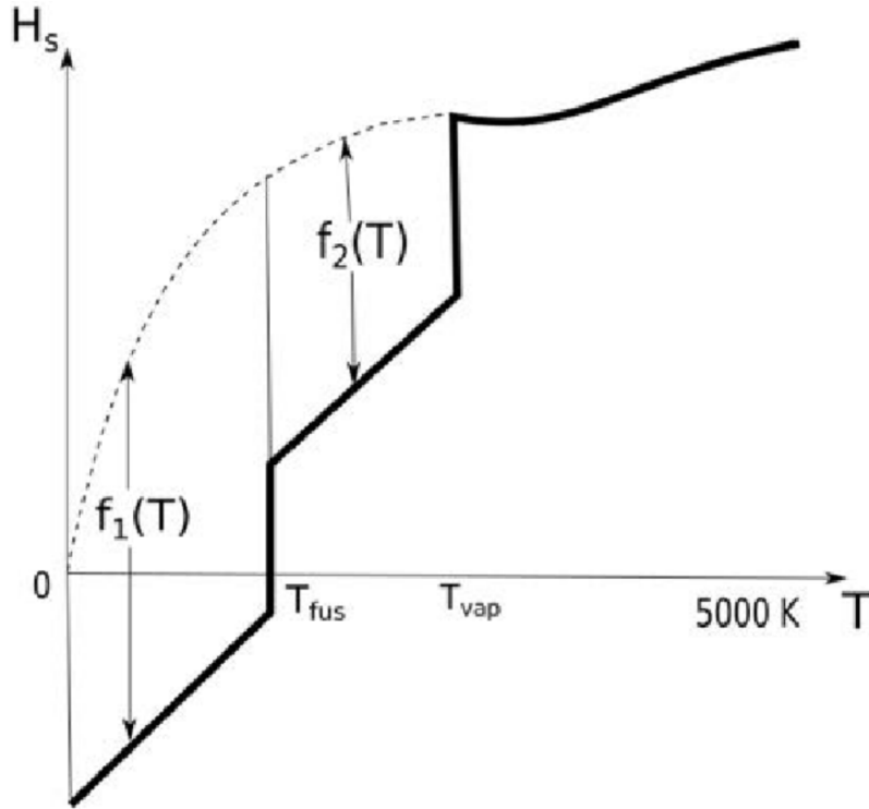
Figure 3.6 – Evolution of the sensible enthalpy with temperature for different phases (in solid line) superimposed with the sensible enthalpy for the gaseous phase (dashed line). Figure extracted [105].
