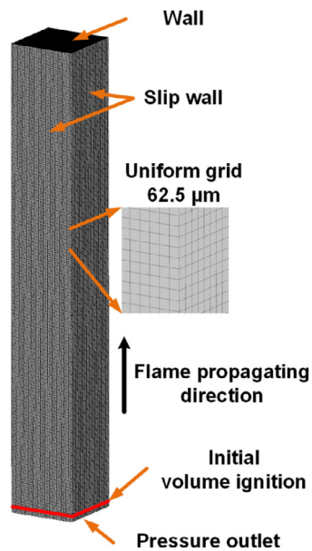
Figure 1.21 – Computational domain and boundary conditions for Al dust combustion. Figure extracted from Han et al. [54].
