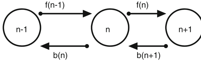
Figure 3.18 – Schematic representation of the kinetics of homogeneous nucleation; f(n) is the forward rate which corresponds to condensation while b(n) is the backward rate which corresponds to evaporation. Figure extracted from [66].
