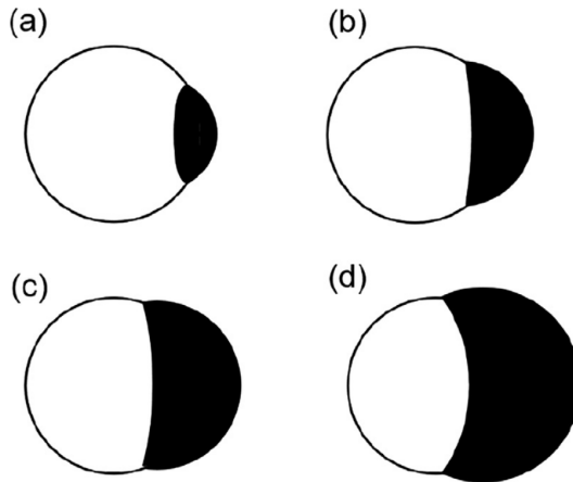
Figure 3.10 – Aluminum (white)/alumina (black) droplet geometry for four alumina mass fractions Y_{Al_2O_3} = 0.1(a), 0.3(b), 0.5(c) , and 0.7(d) . Figure extracted from [41].
