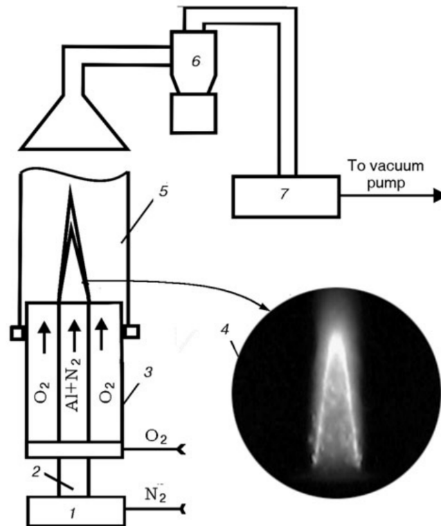
Figure 5.19 – Diagram of the dust burner used by Poletaev et al. [92]: 1) dispersion unit; 2) inner burner tube; 3) outer burner tube; 4) flame; 5) protective quartz tube; 6) trapping system; 7) fabric filter. Figure extracted from Poletaev et al. [92].
