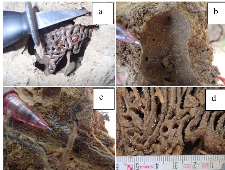
Figure 21. Soil features next to the fourth soil profile (CB4) with (a) comb chamber in a termite nest, (b) evidences of fungi mycelium in a comb chamber, (c) mycelium in the soil material of the termite mound, and (d) detail of exosymbiotic fungus Termitomyces .
