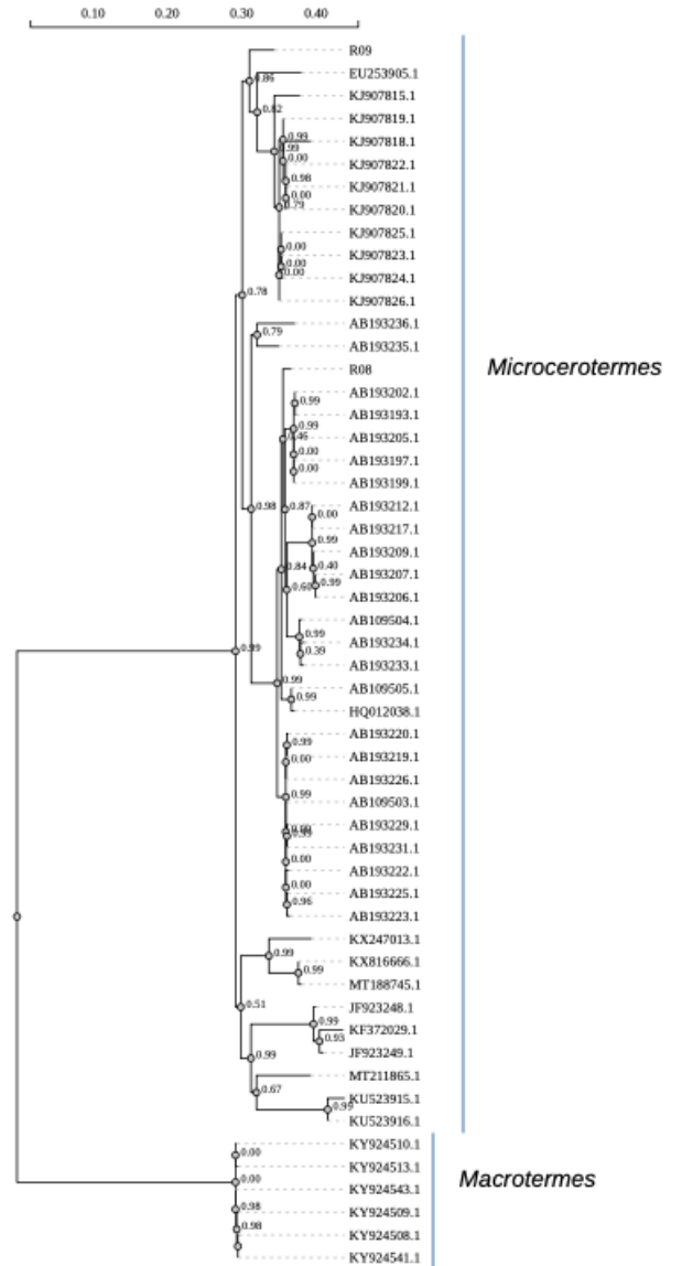
Phylogenetic tree of Microcerotermes with Macrotermes as an outgroup
