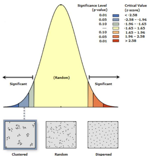
A6. Example of theoretical Average Nearest Neighbor results calculated using ArcMap 10.7. Both z-scores and p-values are associated with the standard normal distribution. At P < 0.10 , very low (negative) z-scores indicate significantly clustered distributions, while dispersed distributions correspond to very high z-scores. Random distributions are given for P > 0.10 .
