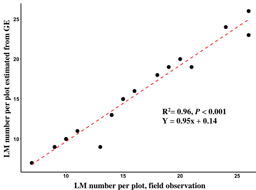
A5. Number of lenticular mounds (LMs) with trees nearby inventories in the field in 2019 and estimated using Google Earth images (n =19 plots)
