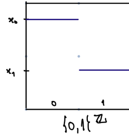
Figure 5.1 A representation of x(\omega) = x_{\pi_0(\omega)}
