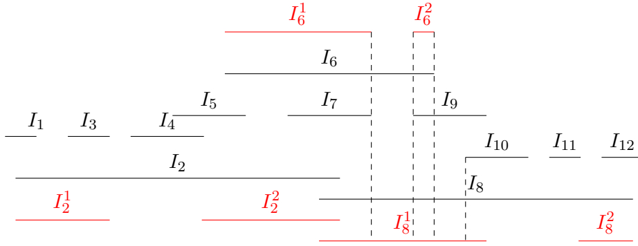
Figure 5.4.: Interval representation of the graph G with the 2-intervals representing non-original intervals in red. No way of “cutting” I_6 leads to a disjoint unit 2-interval representation.
