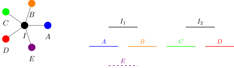
Figure 4.2.: A (disjoint) unit 2-interval graph cannot contain an induced K_{1,5} .
