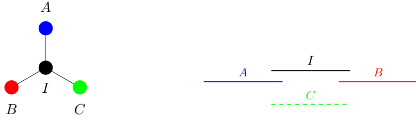
Figure 4.1.: A unit interval graph cannot contain an induced K_{1,3} .
