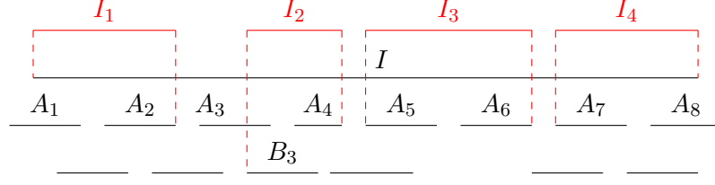
Figure 5.2.: Interval I intersects 8 disjoint intervals. In red, the 4-interval returned by the algorithm. Note that if l(I_2) were defined as l(A_3) instead of l(B_3) , it would intersect three pairwise disjoint original intervals.
