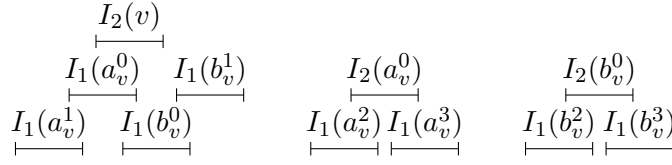
Figure 6.12.: A unit 2-interval representation of B_v (Figure 6.11), i.e., \mathbf{D}_{B_v} for an arbitrary v \in V_{\text{black}} . Note that only one interval of v is used ( I_2(v) ), while the other one remains free to display the rest of the neighborhood of v (and is not represented here).
