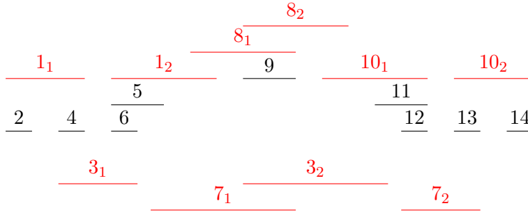
Figure 5.15.: Unit 2-interval representation of the graph in Figure 5.7.
