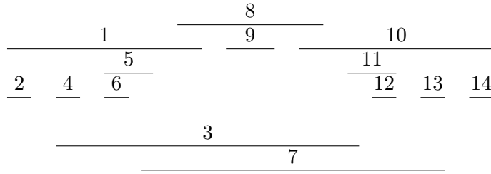
Figure 5.8.: An interval representation of the graph in Figure 5.7.
