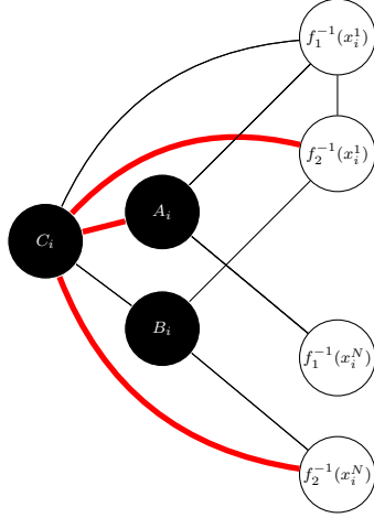
Figure 6.15.: Two representatives of the same literal vertex cannot be adjacent. In this case, there is an induced K_{1,3} caused by the fact that f_1^{-1}(x_i^1) and f_2^{-1}(x_i^1) are adjacent. The representatives of literal vertex x_i^2 are omitted for clarity.
