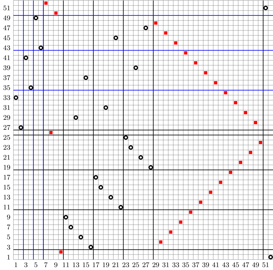
Figure A.1.: Illustration of the construction introduced in the proof of Theorem A.1.
