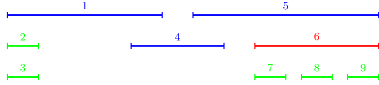
Figure 3.4.: Interval representation of the graph associated to the PQ-tree in Figure 3.3.
