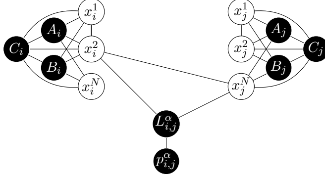
Figure 6.3.: Gadget for a 2-clause \hat{C}_\alpha of the form C_\alpha = (x_i \vee \bar{x}_j) .
