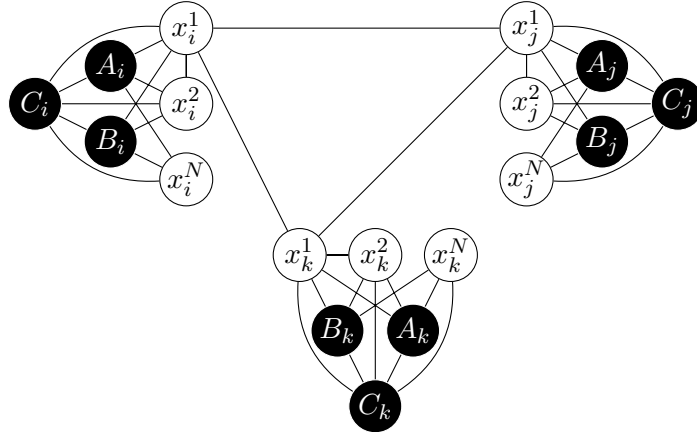
Figure 6.2.: Clause gadget \hat{C}_\alpha associated to a 3-clause C_\alpha = (x_i \vee x_j \vee x_k) . Note that in the final graph, each vertex x_i^m, x_j^m, x_k^m , for every m \in \{1, 2, N\} , will be incident to exactly 2 edges linking them to vertices outside their variable gadget.
