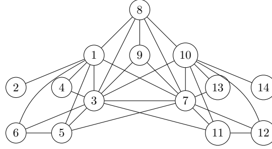
Figure 5.7.: One of the 6 graphs with 14 vertices (the one with the fewest edges) which is an interval graph (see Figure 5.8) and K_{1,5} -free, but not disjoint unit 2-interval.
