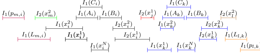
Figure 6.9.: Representation of a longest contiguous block of intervals, where each color represents the intervals associated to a different variable. A longest contiguous block occurs when there is a clause (x_i \vee x_j \vee x_k) , where x_i and x_k are set to false and both of them also appear as positive literals in a 2-clause.
