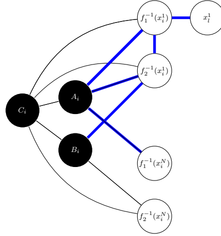
Figure 6.14.: If a black vertex is adjacent to two representatives of a same literal vertex (in this case, A_i is adjacent to f_1^{-1}(x_i^1) and f_2^{-1}(x_i^1) ), then S is not a unit interval graph (there is an induced net, highlighted in blue). The representatives of literal vertex x_i^2 are omitted for clarity.
