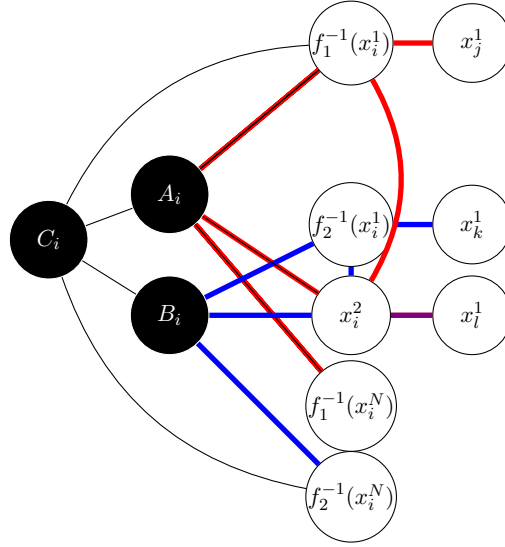
Figure 6.5.: Configuration of S[\hat{V}_i] described in Case 4 of Lemma 6.5. In red, the net created if f_1^{-1}(x_i^1) has an external neighbor, and in blue, the net created if f_2^{-1}(x_i^1) has an external neighbor (edge (x_i^2, x_l^1) is part of both nets and is depicted in purple).
