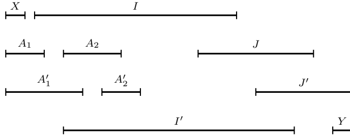
Figure 5.12.: Interval representation of a graph with two vertices that are centers of an E -claw, represented by intervals I and I' .
