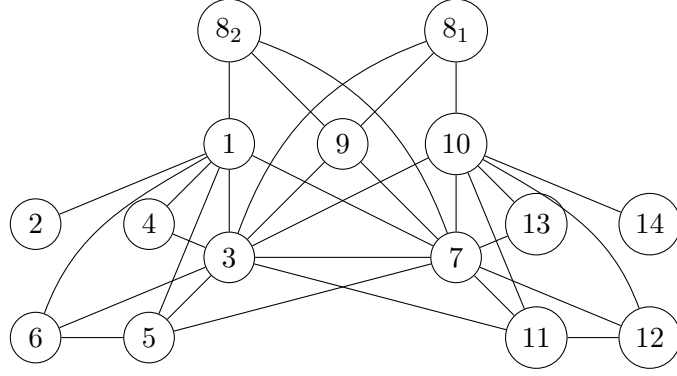
Figure 5.10.: The graph G after the split of vertex 8
