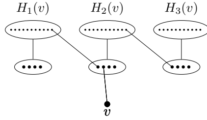
Figure 6.16.: Illustration of the gadget added to every vertex v of the original graph for the case d = 3 . K_{11,4} 's are represented schematically: an edge stopping at the border of an ellipse indicates that it is incident to every vertex within the ellipse.
