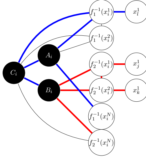
Figure 6.4.: Configuration of S[\hat{V}_i] described in Case 3 of Lemma 6.5. In red, the net created if both f_2^{-1}(x_i^1) and f_2^{-1}(x_i^2) have an external neighbor. In blue, the net created if f_1^{-1}(x_i^1) has an external neighbor.
