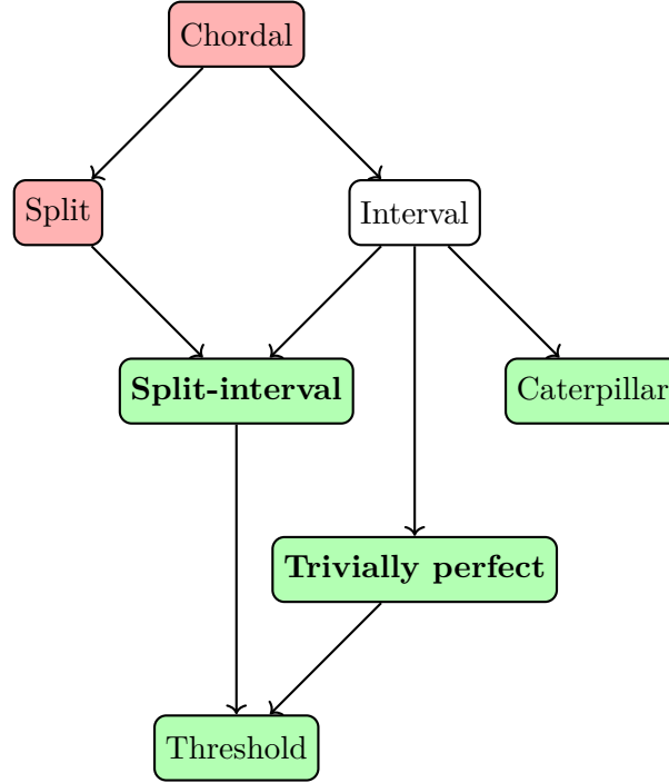
Figure 7.1.: Summary of the complexity of proper interval completion on different subclasses of chordal graphs. A rectangle in red indicates that the problem is NP-hard in this class, while a green rectangle means that it is polynomial. A white rectangle indicates that the complexity is unknown. In bold, the results proven here.
