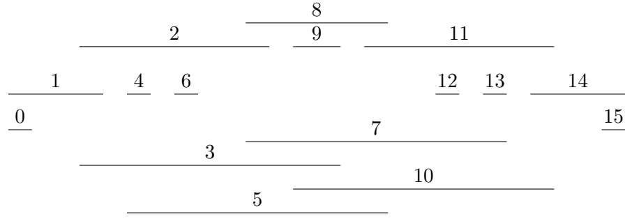
Figure 5.5.: Interval representation of a K_{1,5} -free interval graph for which the algorithm does not return a disjoint unit 2-interval representation. In this particular case, it is not straightforward to find such a representation, even though it exists.
