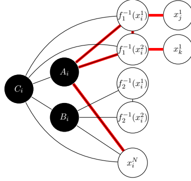
Figure 6.10.: In red, the net created if both representatives of x_i^1 are incident to the clause gadget in S and f_1^{-1}(x_i^2) is incident to an external edge.
