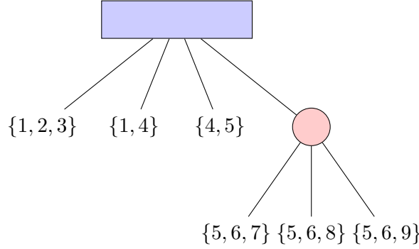
Figure 3.3.: PQ-tree of an interval graph. Q-nodes are represented by blue rectangles, and P-nodes are represented by red circles. Each maximal clique is contained in a leaf and represented by the set of vertices it contains.
