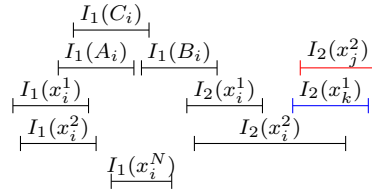
Figure 6.7.: Representation of a 3-clause (x_i \vee x_j \vee x_k) , where x_i is set to false while x_j, x_k are set to true.
