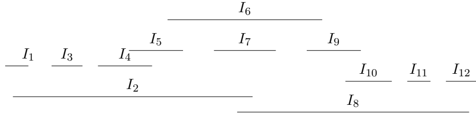
Figure 5.3.: Interval representation of the graph G for which the algorithm does not return a disjoint unit 2-interval representation.
