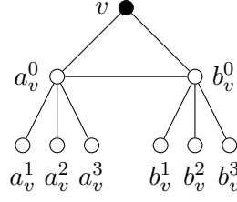
Figure 6.11.: Gadget B_v used to replace every black vertex v of G in the construction of G' . Vertex v is a public vertex, as it is adjacent to vertices of the gadget ( a_v^0 and b_v^0 ) and vertices outside the gadget (namely, its neighbors in the original graph G ), whereas the rest of the vertices are private , as their only neighbors are vertices from the gadget (the ones shown in the figure).
