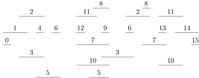
Figure 5.6.: Disjoint 2-interval representation of the graph in Figure 5.5. The fact that no interval intersects three pairwise disjoint intervals implies that the input graph is disjoint unit 2-interval.
