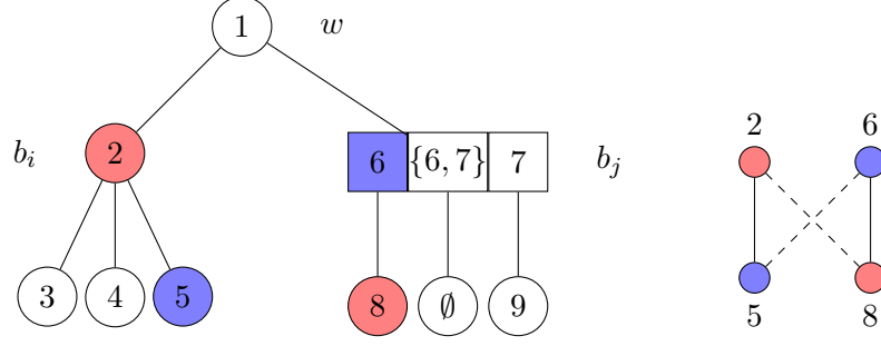
Figure 7.2.: If a node w has two children b_i and b_j such that T_{b_i} and T_{b_j} both contain a pair of vertices with one vertex in C_1 and the other in C_2 , the partition yields a completion with an induced C_4 . A node in red indicates that the vertex contained inside belongs to C_1 , while a node in blue indicates that it belongs to C_2 . To the right of the MPQ-tree we depict the induced C_4 in the completion: full edges represent edges already present in G while dashed edges represent fill edges.
