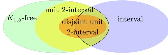
Figure 5.1.: K_{1,5} -free interval graphs are not contained in the class of disjoint unit 2-interval graphs. The class of unit 2-interval graphs is a superclass of disjoint unit 2-interval graphs, and spans the whole intersection of K_{1,5} -free and interval graphs.
