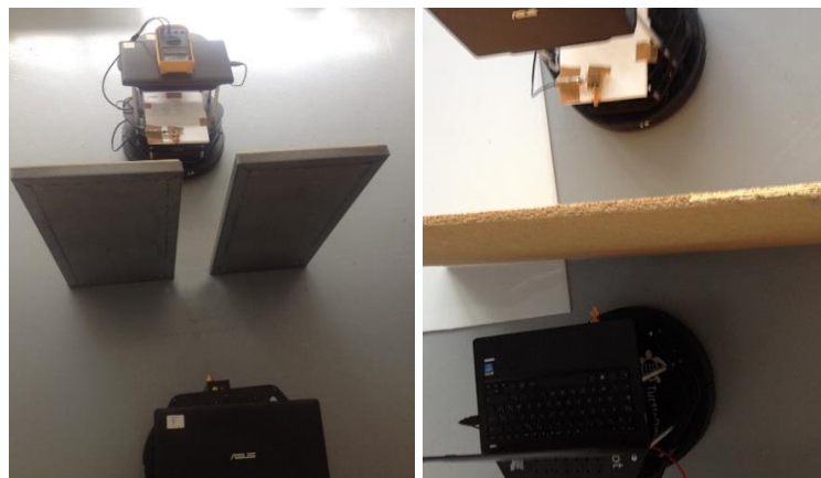
Figure 1.1 Microwave on-destructive testing platform.
