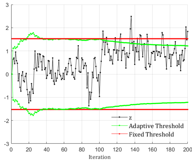
Figure 2.12 EWMA – results with fixed/adaptive thresholds.
