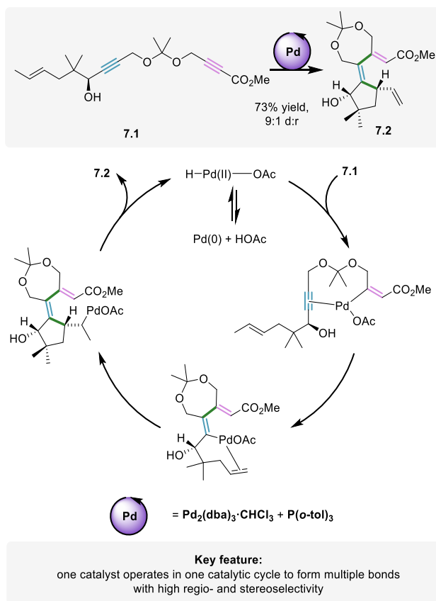
Scheme 5.7. Pd-catalyzed intramolecular domino polyenyne cycloisomerization for the synthesis of terpene derivatives.
