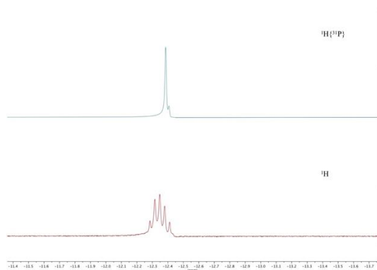
Figure 2.28: Formation of Rh-H as detected by ^{31}\text{P} -decoupled ^1\text{H} NMR spectroscopy in the reaction with styrene.
