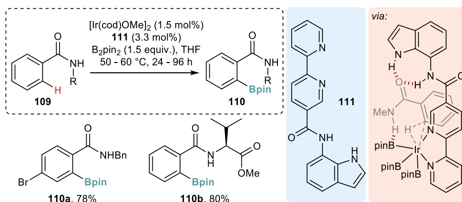
Scheme 1.30. ortho -Selective C–H borylation of aromatic amides enabled by hydrogen bonding by Reek.
