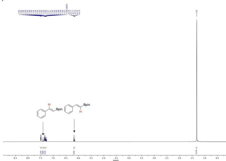
Figure 2.9: Partial deuterium retaining in 3\text{a} in the reaction of (E)\text{-1a-}\beta\text{-d} detected by ^1\text{H-NMR} spectroscopy. Isotomeric cluster of product 3\text{a-d}_n derived by GC-MS analysis:
