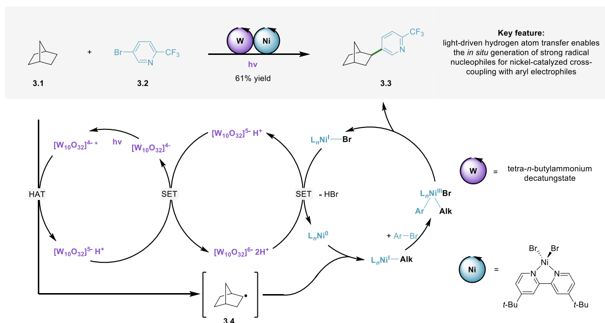
Scheme 5.3. W-/Ni-catalyzed arylation of strong sp^3 -C-H bonds with aryl bromides enabled by light-driven hydrogen atom transfer (HAT).
