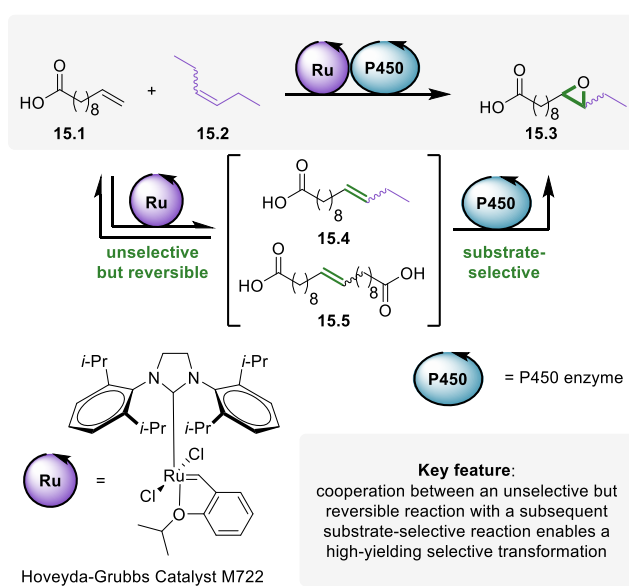
Scheme 5.15. Ru-/P450-catalyzed orthogonal relay of reversible olefin cross-metathesis and substrate-selective epoxidation of alkenes.
