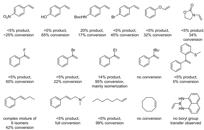
Figure 2.47: Overview of unsuccessful substrates.
