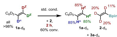
Figure 2.14: Partial deuterium retaining in 3a in the reaction of 1a-d 8 detected by GC-MS analysis.
