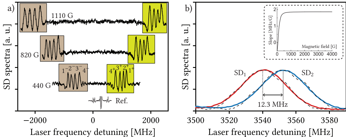
Figure 4.7 – ^{39}\text{K} D_1 line spectra recorded for L = 120 \pm 5 nm. a) SD absorption spectra for B_z increasing from 440 to 1110 G. Lower curve: SD of a saturated absorption spectrum for reference. Transition labeling is consistent with fig. 4.2, \sigma^- and \sigma^+ are shown in the brown and green regions respectively. b) The red curve has been calculated for B_1 = 2000 G and the blue curve for B_2 = 2007 G. Black curves depict experimental SD absorption spectra for B_1 and B_2 , used to measure 3.3 G/ \mu\text{m} gradient when the NC ( L = 120 \pm 5 nm) is placed on a micrometer stage at B_1 = 2000 G and shifted by 2 \mu\text{m} relative to the initial position when B_2 becomes 2007 G. As can be seen, when moving the NC by 2 \mu\text{m} , the frequency shift is 12.3 MHz, which can be measured well. The inset shows the slope [MHz/G] of the F = 1, 2 \rightarrow F' = 1, 2 transitions.
