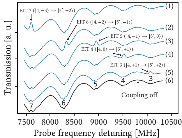
Figure 5.5 – Probe transmission spectra of the Cs nanocell ( L = \lambda = 852 nm). The probe frequency is scanned so that it is successively resonant with transitions 3 to 7, following the labeling presented in fig. 5.1). Each spectrum (from 1 to 5) exhibits an EIT resonance. These EIT resonances are labeled EIT 3 to EIT 7, and the transition to which the coupling laser is tuned is specified. As an example, for EIT 3, the two lasers form a \Lambda -system with the probe laser resonant with transition 3 ( |3, -1\rangle \rightarrow |5', -2\rangle ) and the coupling laser \nu_{c_3} tuned to transition |4, +1\rangle \rightarrow |5', +2\rangle . The bottom black line (spectrum 6) corresponds to the case where the probe is scanned but the coupling is turned off. The coupling powers are respectively 10 and 0.05 mW and the external magnetic field is B = 1400 G. Small VSOP peaks are visible on each atomic resonance. Zero frequency corresponds to the transition frequency of Cs D_2 line.
