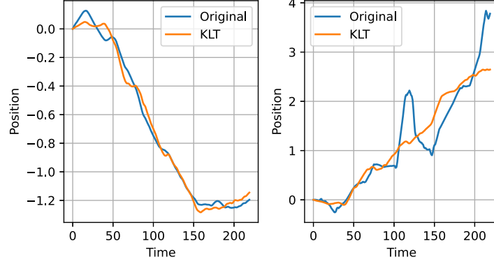
Figure 3.18: Approximation with 9 components of the lateral component of two sample trajectories.
