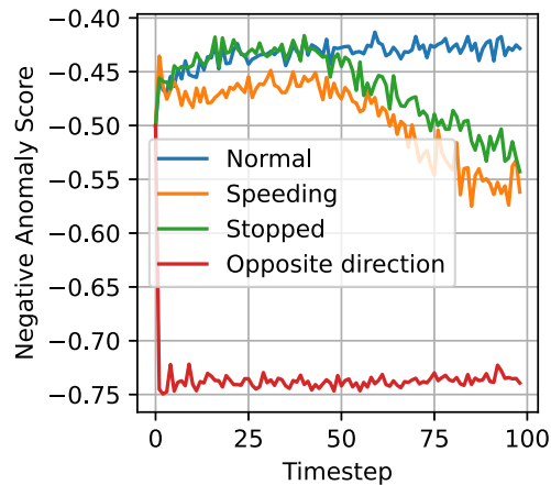
Figure 4.12: Anomaly scores computed in real-time with Isolation Forest
