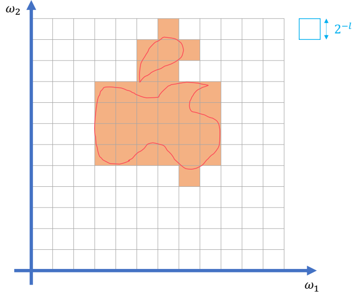
Figure 6.4: Discretization \pi of the exemplary 2D sample space \Omega and the identity mapping \mathbf{1}_\pi that maps B onto the cells whose size is 2^{-l} .
