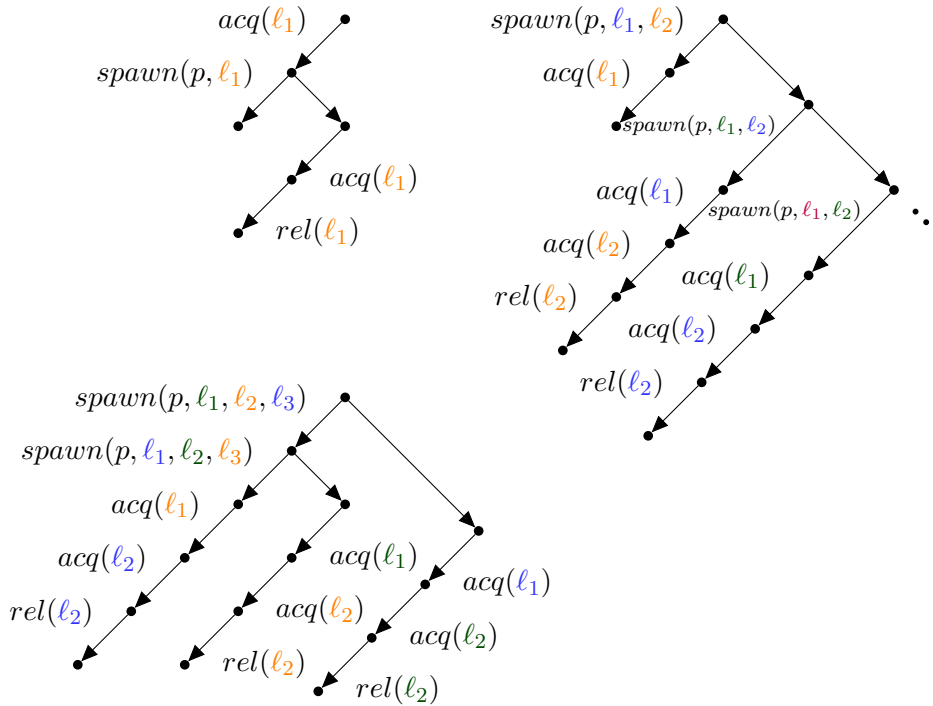
Figure 5.2: Some trees that cannot be obtained as the limit of a run.
