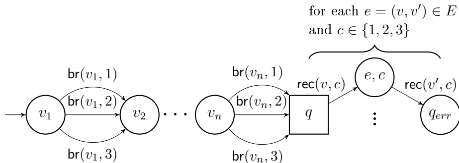
Figure 3.4: Illustration of the lower bound proof from Theorem 3.15.
