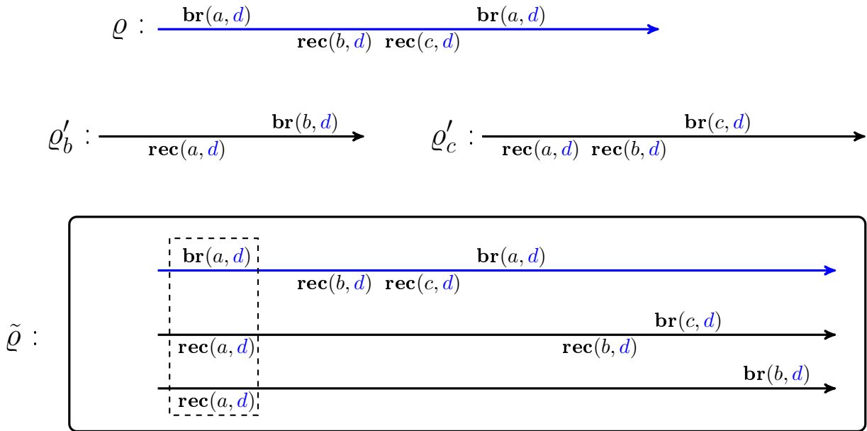
Figure 3.7: An illustration of the proof of Lemma 3.34. The partial run \varrho is compatible with decomposition (a, b, a, c, \varepsilon) . We have \mathbf{In}_d(\varrho_b) = a \in \mathcal{L}_{(a)} and \mathbf{In}_d(\varrho_b) = ab \in \mathcal{L}_{(a,b,a)} . We build a partial run \tilde{\varrho} such that aacb \sqsubseteq \mathbf{Out}_d(\tilde{\varrho}) . Note that \tilde{\varrho} is also compatible with decomposition (a, b, a, c, \varepsilon) . We ignore data other than d in this picture.
