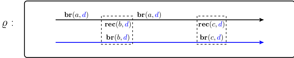
Figure 3.9: An illustration of the proof of Lemma 3.36. Datum d is initial in \varrho' and not \varrho . We ignore data other than d in this picture.
