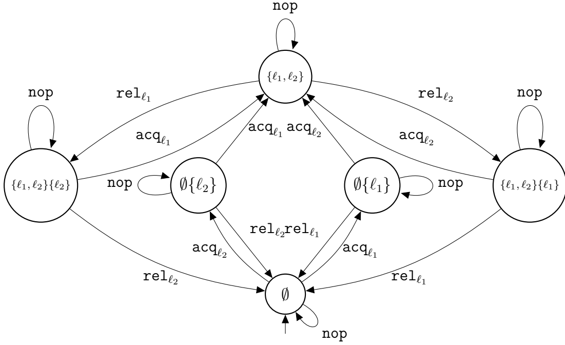
Figure 4.6: The automaton structure for pattern recognition.
