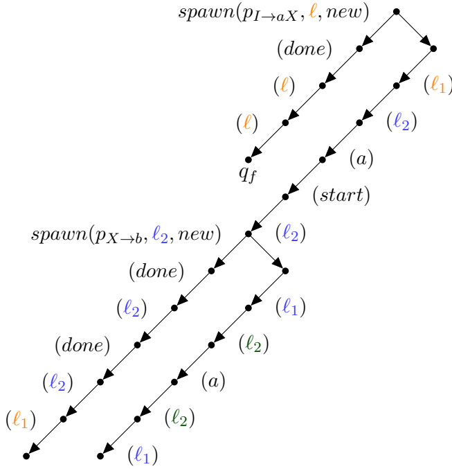
Figure 5.3: A run of a DLSSV \mathcal{S} as in the proof of Theorem 5.33, simulating the rules I \rightarrow aX , X \rightarrow b .
