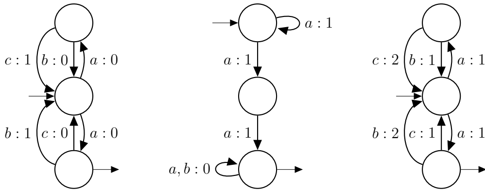
Figure B.5: The left automaton is 2-explorable, the middle one is not explorable but is \omega -explorable, the third one is not \omega -explorable. These examples are taken from [HK23].
