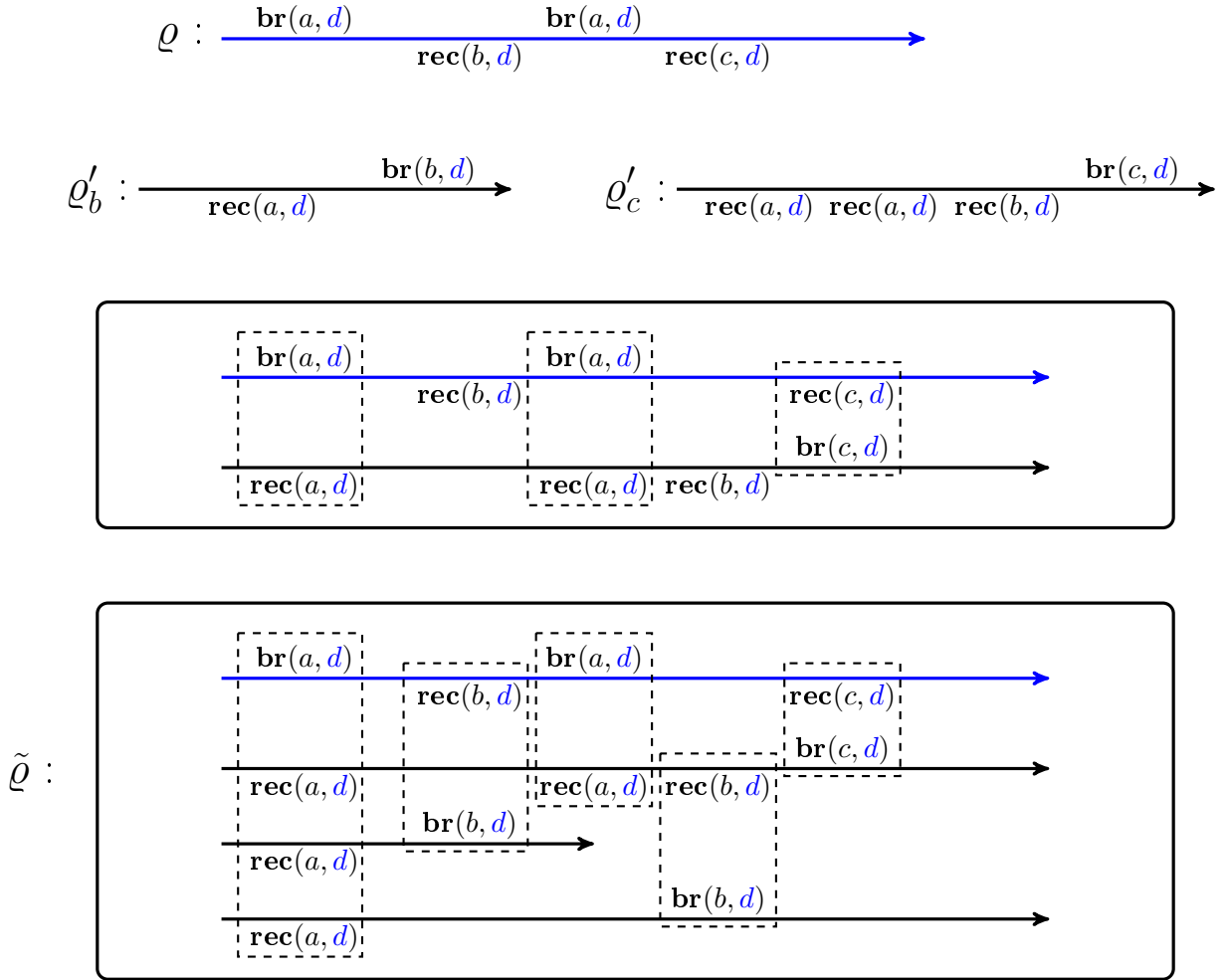
Figure 3.8: An illustration of the proof of Lemma 3.35. The partial run \varrho is compatible with decomposition (a, b, a, c, \varepsilon) . We have \mathbf{In}_d(\varrho_b) = a \in \mathcal{L}_{(a)} and \mathbf{In}_d(\varrho_b) = aab \in \mathcal{L}_{(a,b,a)} . We build \tilde{\varrho} such that \mathbf{In}_d(\tilde{\varrho}) = \varepsilon . We start by using \varrho'_c to eliminate the unmatched receptions of c (while adding some unmatched receptions of b ), then we use \varrho'_b to eliminate the unmatched receptions of b . We ignore data other than d in this picture.
