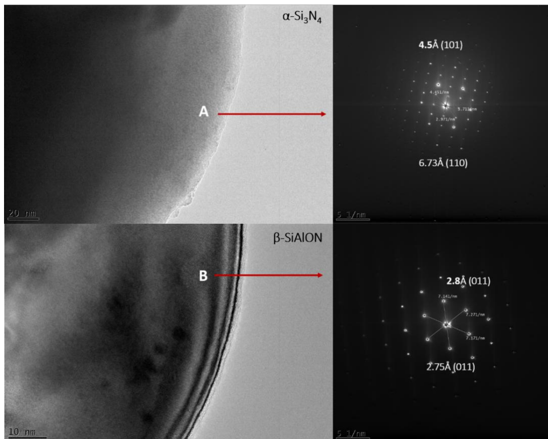
Figure V.14. TEM analysis of PAICe0.05SZ3_16 .
