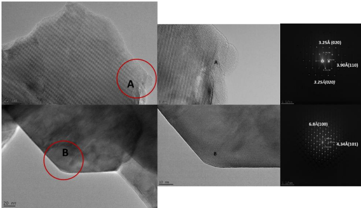
Figure V.12. TEM observations of PAICe0.01SZ3_16 .
