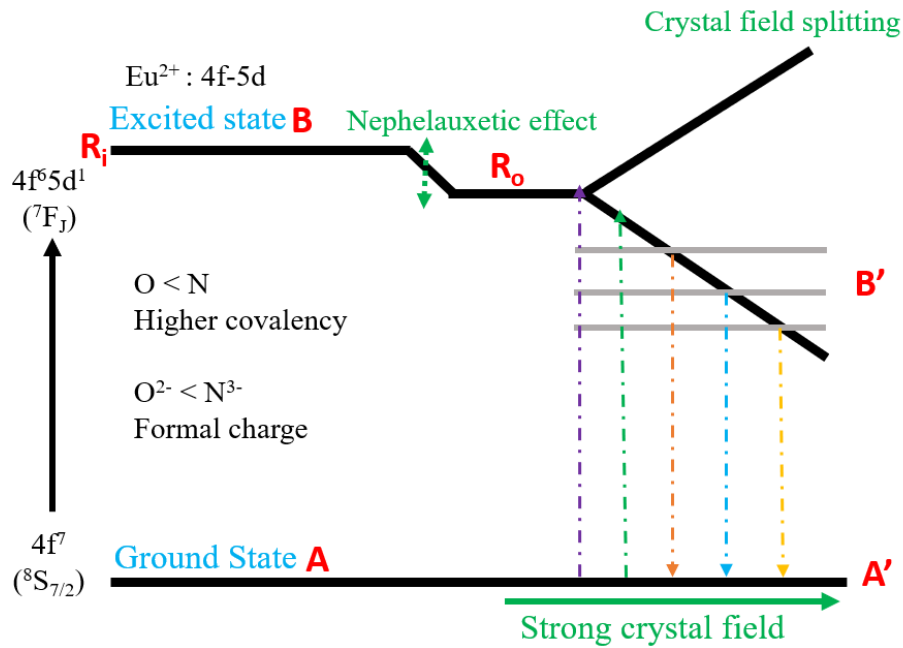
Figure I.5. Crystal field splitting and nephelauxetic effect of Eu 2+ -doped SiAlON 48 .
