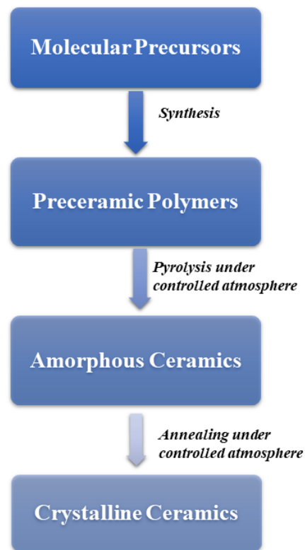
Figure I.9. Flow chart for the formation ceramics by using polymer derived ceramic route.
