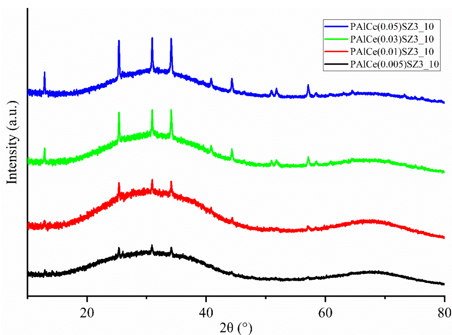
Figure V.4. XRD patterns of PAICeYSZ3_10 (0.005 ≤ Y ≤ 0.05).
