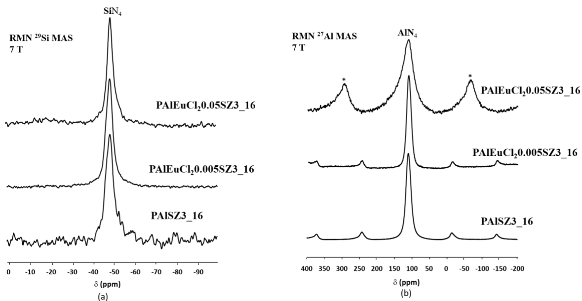
Figure IV.5. Solid-state NMR spectra of PAISZ3_16 , PAIEuCl 2 0.005SZ3_16 and PAIEuCl 2 0.05SZ3_16 samples: (a) 29 Si MAS NMR and (b) 27 Al (b) MAS NMR (* indicate spinning sidebands).
