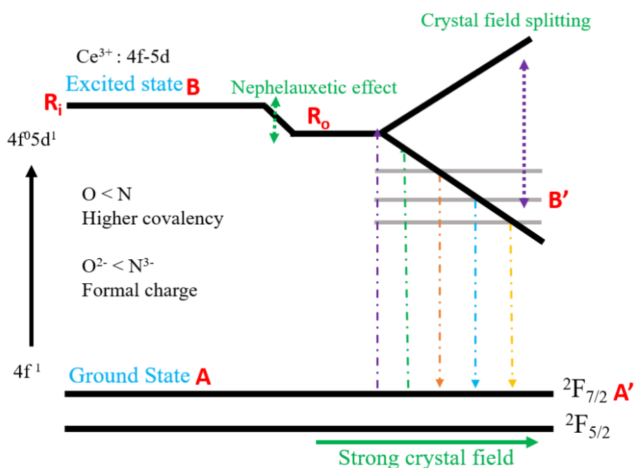
Figure I.6. Crystal field splitting and nephelauxetic effect of Ce 3+ -doped SiAlON 52 .
