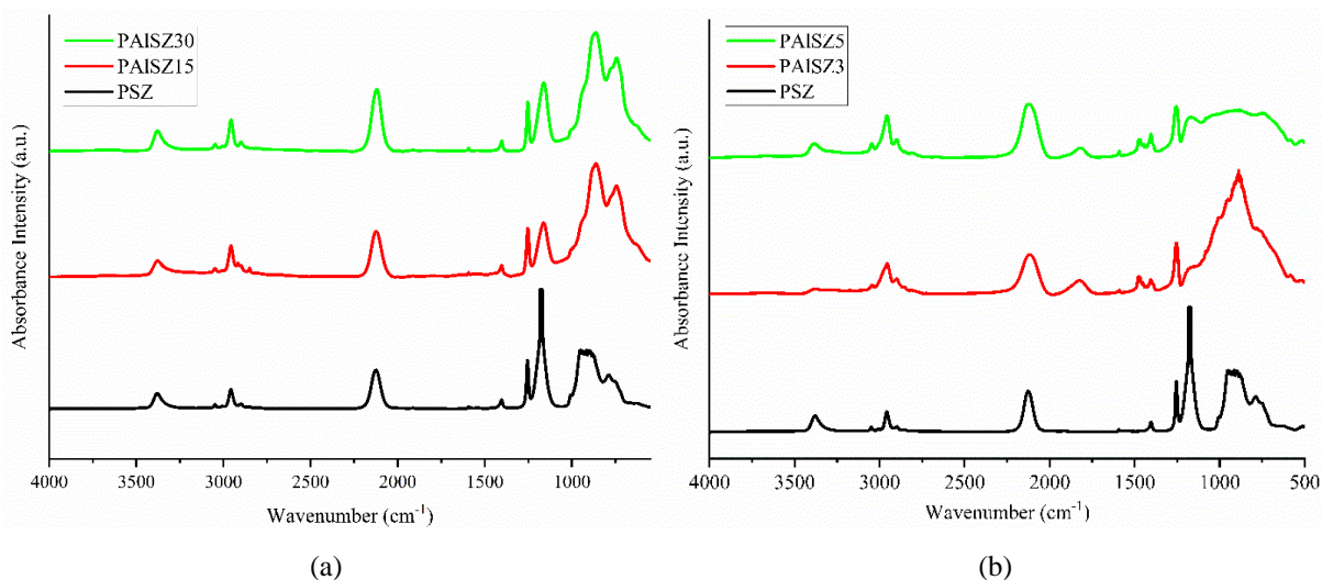
Figure III.3. FTIR-ATR spectra of (a) liquid PAISZX ( 30 \leq X \leq 15 ) and (b) of solid PAISZX ( 5 \leq X \leq 3 ).
