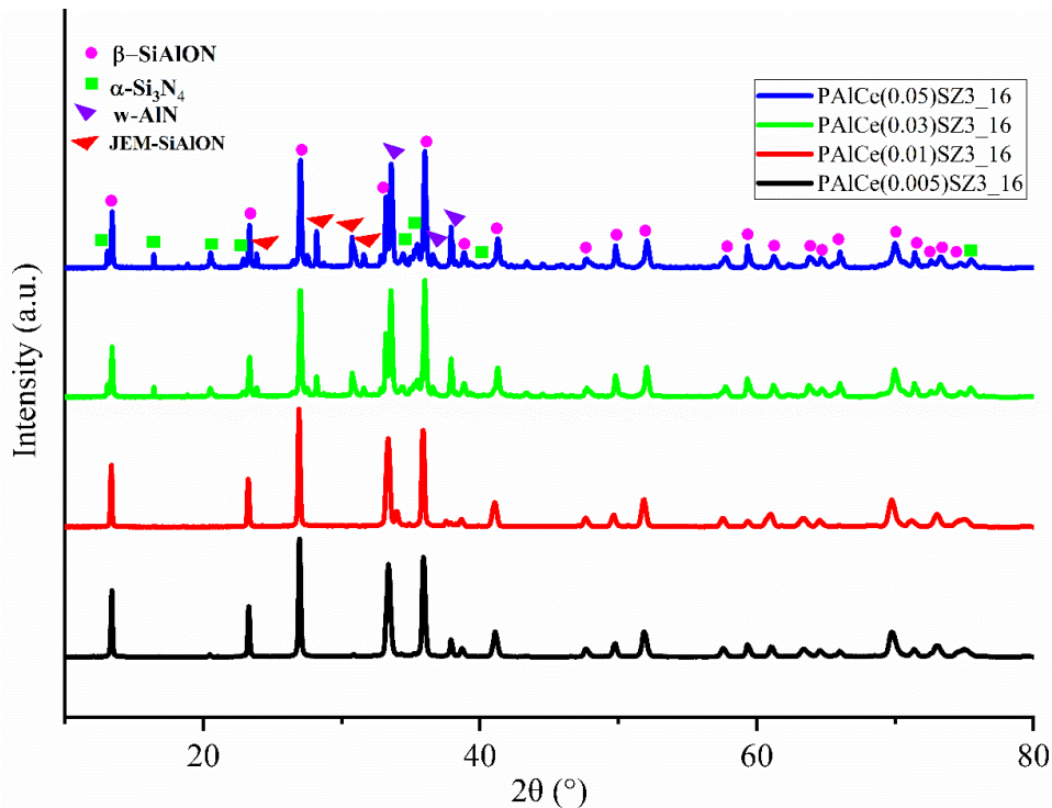
Figure V.7. XRD patterns of PA1CeYSZ3_16 ( 0.005 \leq Y \leq 0.05 ).
