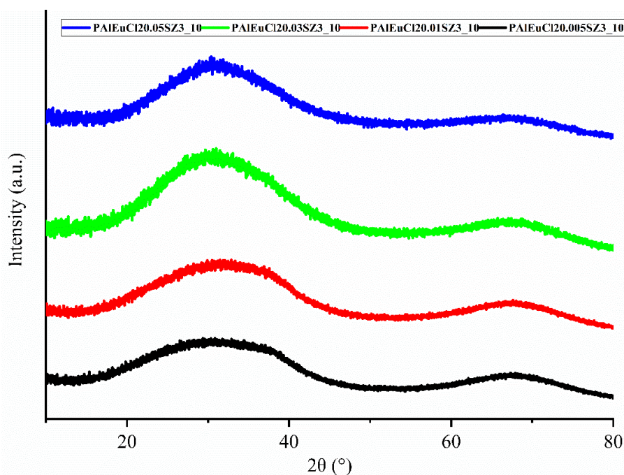
Figure IV.4. X-ray diffraction (XRD) patterns of PAIEuCl 2 YSZ 3 _10 (0.005 ≤ Y ≤ 0.05).
