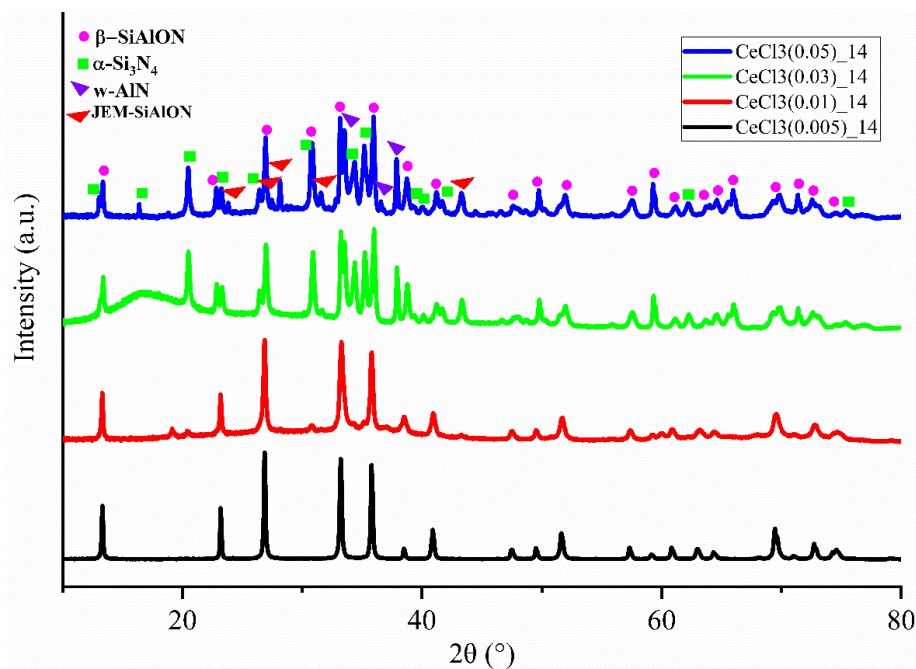
Figure V.6. XRD patterns of PAICeYSZ3_14 ( 0.005 \leq Y \leq 0.05 ). The halo shape around ( 10-20^\circ ) for PAICe0.03SZ3_14 sample comes from sample holder.
