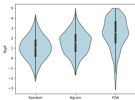
(c) logP
