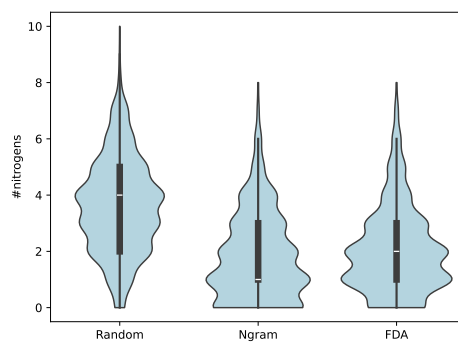
(n) #nitrogens
