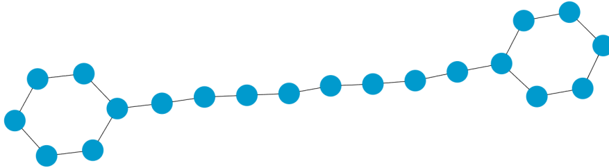
Fig. 1. A counter-example of Graffiti 289 of size 20 (second largest eigenvalue \leq mean of the mean of all adjacent vertex degree for all nodes)
