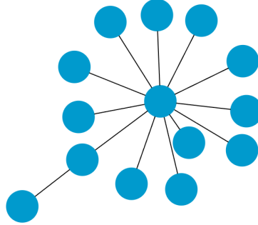
Fig. 2. A counter-example of Graffiti 301 of size 14 (scope of positive eigenvalues \leq harmonic) Edges: 0-1, 0-2, 1-3, 1-4, 1-5, 1-6, 1-7, 1-8, 1-9, 1-10, 1-11, 1-12, 1-13
