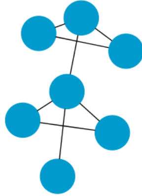
Fig. 5. Counter example of conjecture 4
