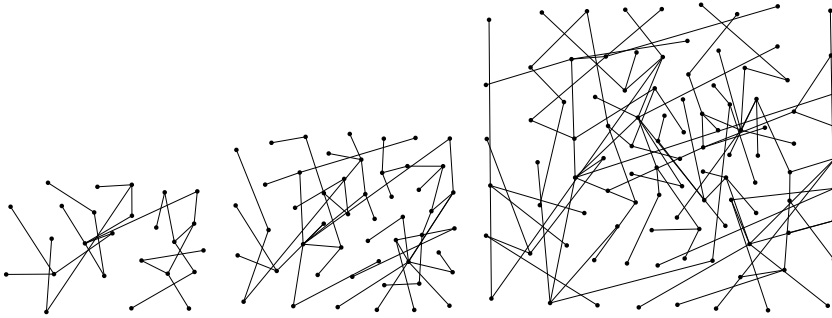
Fig. 1: Graphs of size 25, 50, 100 generated by seed 0
