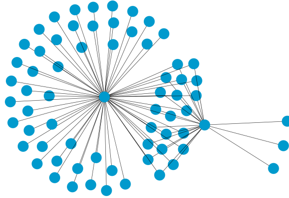
Fig. 5. A counter-example of Graffiti 137 of size 67 (second largest eigenvalue \leq harmonic)
