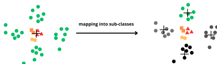
Figure 1: Schematic diagram of the subclass mapping process. Although the green points are locally clustered, their centroid is close to samples from minor classes, which makes distinguishing between classes less effective. We use the subclass mapping to address this issue.
