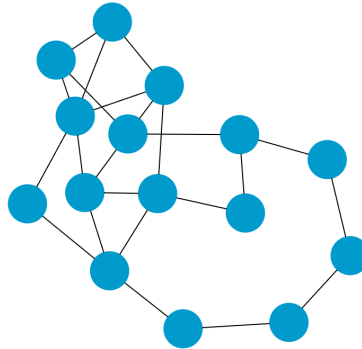
Fig. 3. A counter-example of Graffiti 30 of size 15 (# positive distance eigenvalues \leq sum of temperatures) Edges: 0-1, 0-3, 0-12, 1-2, 1-3, 2-3, 2-7, 2-12, 3-4, 3-5, 4-6, 5-6, 5-7, 5-12, 6-7, 6-8, 7-9, 8-10, 9-11, 10-14, 11-12, 11-13, 13-14
