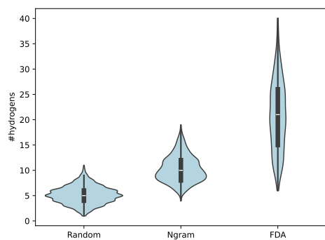
(m) #hydrogens
