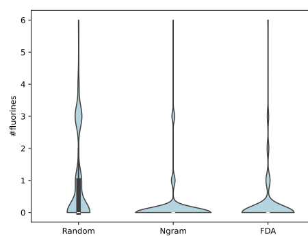
(l) #fluorines
