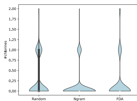
(h) #chlorines
