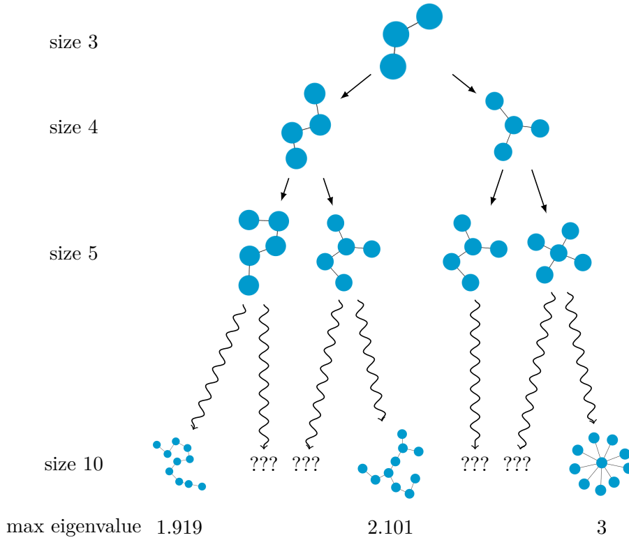
Figure 1.1: Search tree of the tree generation problem. The ondulated arrows represent playouts from size 5 graphs to terminal size 10 graphs. MCTS algorithm should direct themselves toward the right size of the search space tree during their search.
