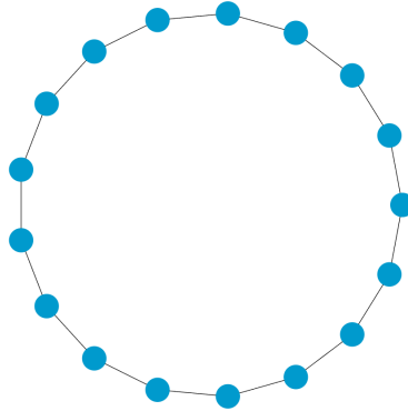
Fig. 7. A counter-example of Graffiti 197 of size 17
