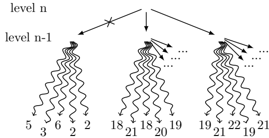
Fig. 2: Level n LNMCS pruning a search subtree and launching n-1 LNMCS on surviving search subtrees.
