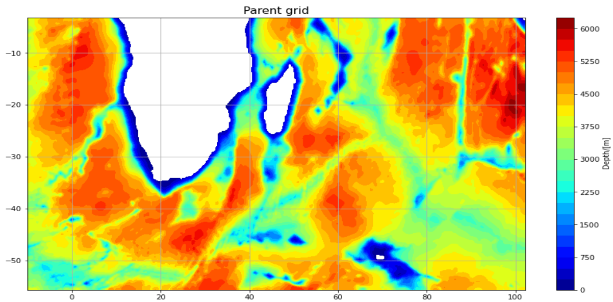
Parent grid ( Dx \sim 22.5\text{km} )
