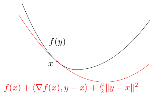
Figure 2.3: Illustration of the strong convexity of a function. The function is lower bounded by the quadratic function y \mapsto f(x) + \langle \nabla f(x), y - x \rangle + \frac{\mu}{2} \|y - x\|^2 for a given x \in \mathbb{R}^p .
