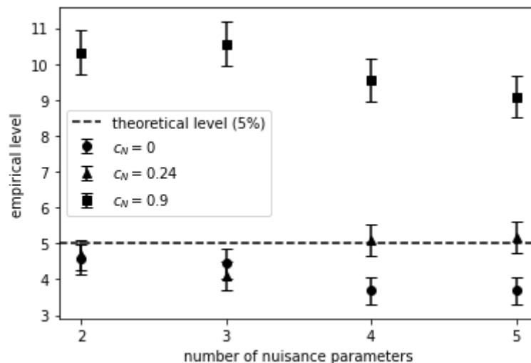
Figure 2.2 – Comparison of the parametric Bootstrap procedure and the shrunked parametric Bootstrap procedure in m_3 , using K = 2500 datasets of size N = 30 and B = 300 Bootstrap replicates for varying numbers of nuisance parameters, and different shrinkage parameters c_N .
