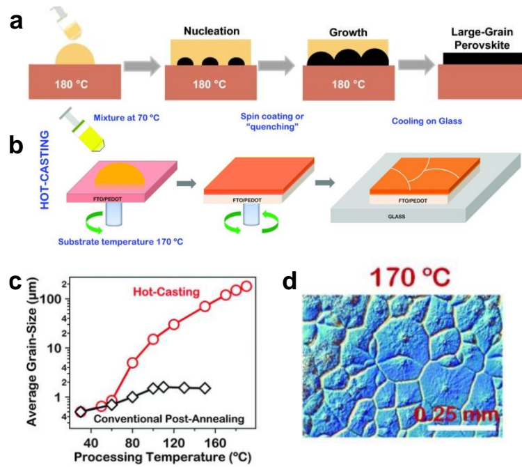
Figure 23: Hot-casting method to crystallize spin-coated perovskite precursors films. a) With substrate heating at 180 °C [130,131]. b) With heated solution and heated substrate at 170 °C [132].
