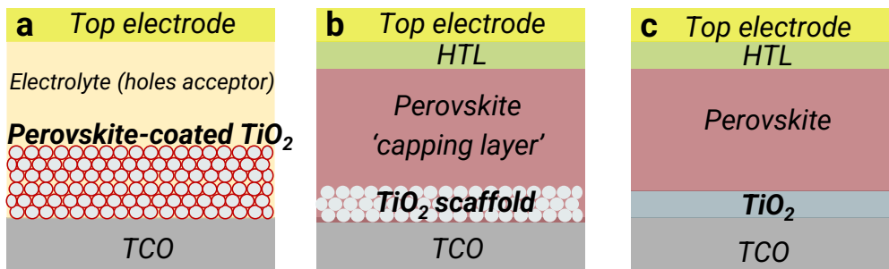
Figure 25: Schematics of devices using \text{TiO}_2 as electron extractor: a) Dye Sensitized Solar cell. b) Mesoporous perovskite solar cell (n-i-p configuration) c) Planar perovskite solar cell.
