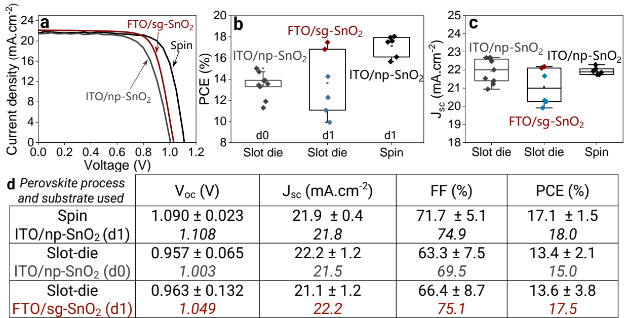
Figure 11: a) J - V curves of the best device per batch (measured at d0 or d1). b) Statistics of power conversion efficiencies. c) Statistics of short-circuit current densities. d) Summary of J - V parameters for the three conditions. The parameters of the champion devices plotted on panel b are in italic.
