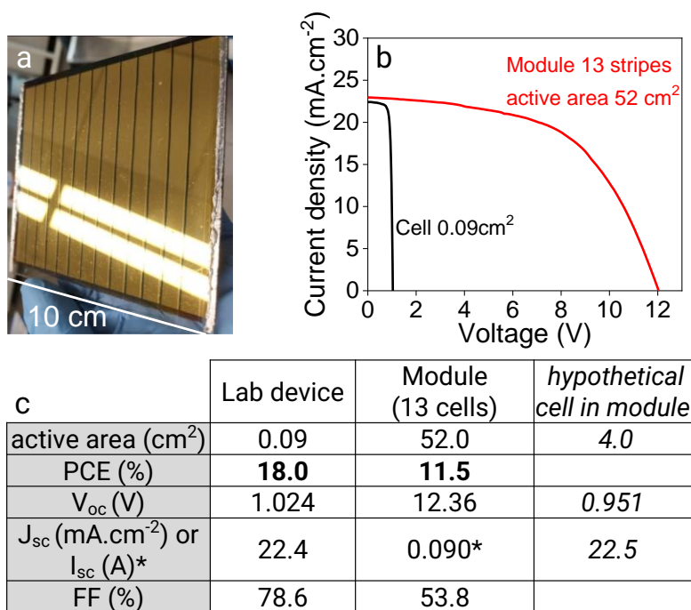
Figure 30: a) Picture of the photovoltaic module fabricated over 52 cm 2 active area with 13 stripes with the FTO/sg-SnO 2 /CBD-SnO 2 /Perovskite (slot-die)/Spiro-OMeTAD/Au device structure. b) J-V curves of a 0.09 cm 2 device and of the module (measured in reverse bias). c) Comparison of the device electrical parameters and extraction of an hypothetical stripe electrical parameters from the module.
