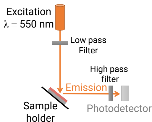
Figure 15: Configuration used for the photoluminescence measurement.
