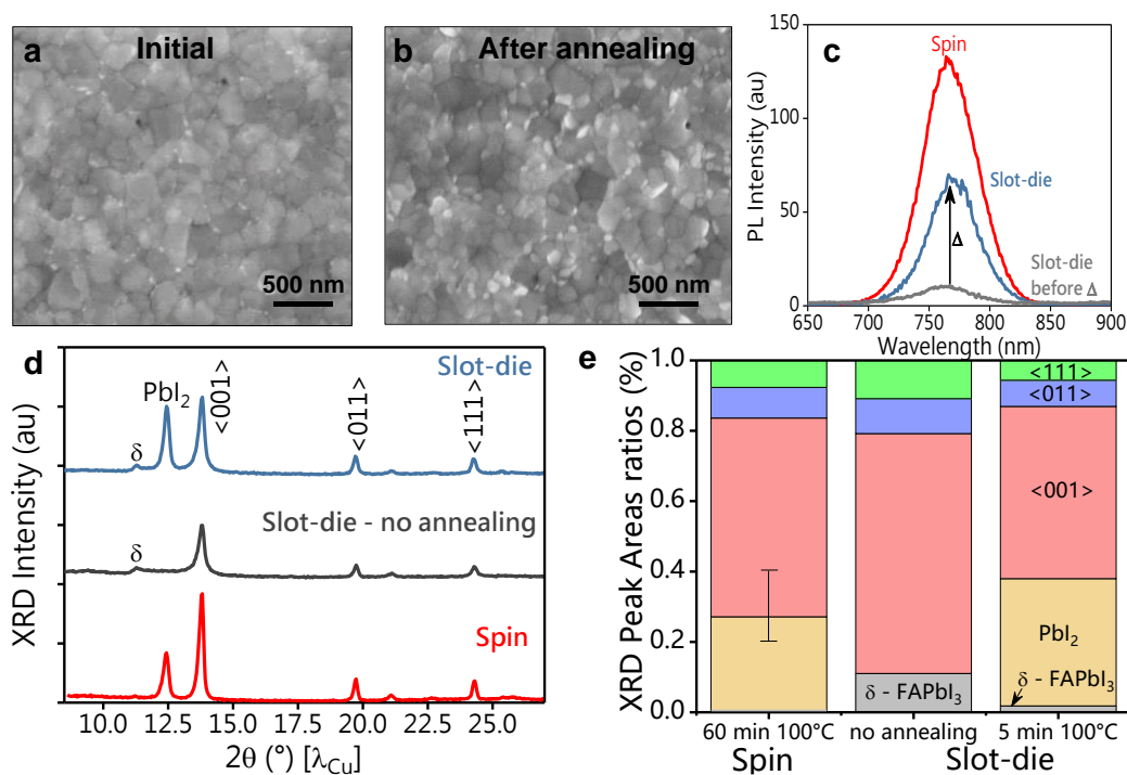
Figure 20: a-b) SEM top images of slot-die coated layers “as-quenched” and after 5 min at 100 °C. c) Photoluminescence spectra, d) X-Ray diffraction patterns, and e) Corresponding XRD peak area ratio extraction of the layers shown in a) and b). The reference spin-coated layer is added for comparison.
