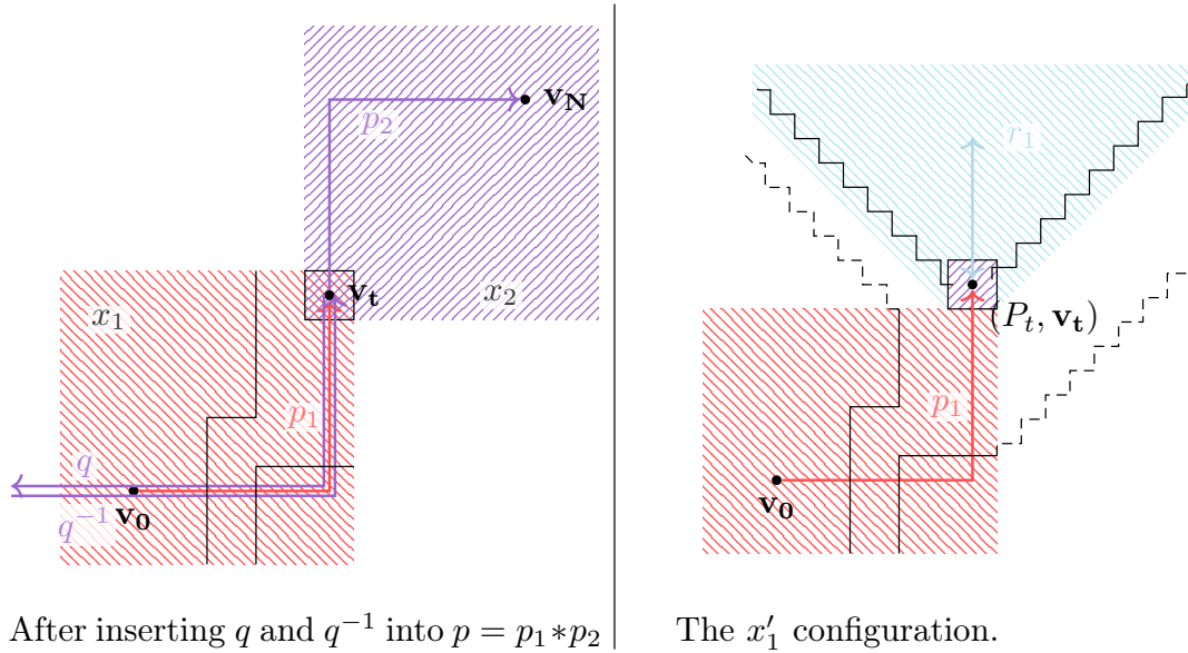
Figure 3.22: Red paths are traced in x_1 , purple ones in x_2 . Wires are drawn in black.
