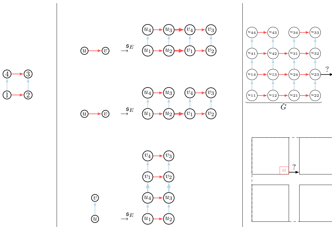
Figure 4.12: An example of non-deterministic substitution, whose iterates are subgraphs of \mathbb{Z}^2 . The presence of the edge marked by a ? depends on information not directly available in G , and might depend on choices made arbitrarily far in the derivation sequence.
