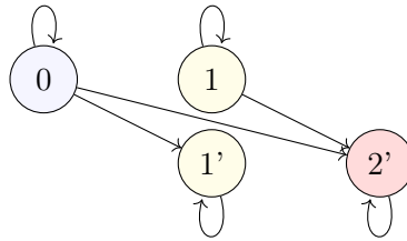
Figure 3.8: Graph giving the horizontal adjacency rules for X . An edge (u, v) indicates that the colour v can be placed to the right of u .
