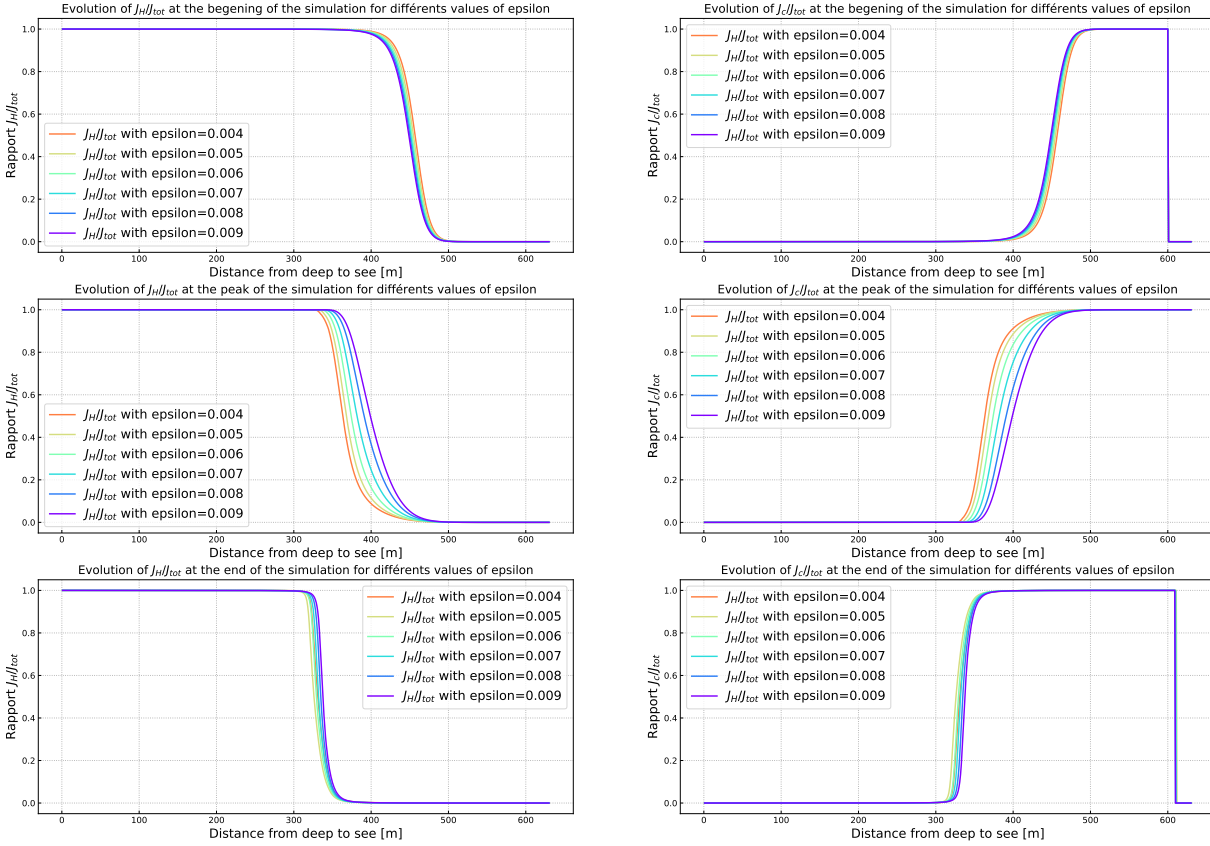
Figure B.5 – Rappports \frac{J_{\mathcal{C}}}{J_{tot}} and \frac{J_{\mathcal{H}}}{J_{tot}} at different times of the simulation: at the beginning, at the peak and at the end: according to different values of \epsilon .
