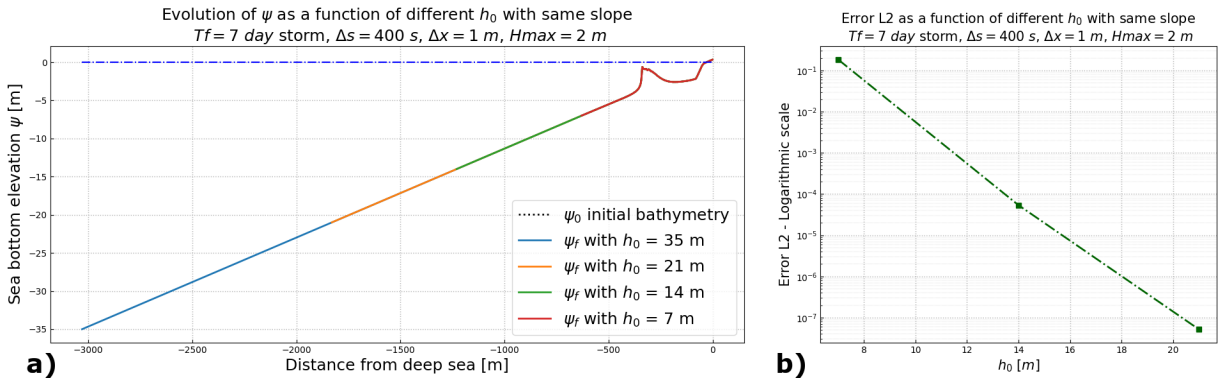
Figure 1.14 – a) Different final bottom profiles for domains of sizes [600, 1200, 1800, 3000] m corresponding to offshore wave heights of h = [7, 14, 21, 35] \text{ m} . The representation is truncated at 7 m depth. b) L^2 error comparing each simulation to the reference solution corresponding to the 3000 m domain (the longest, represents deep-water conditions).
