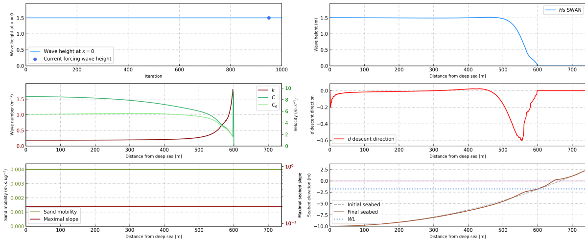
Example Simulation 1D of storm in convex bathymetry with tide Parameters: H_0 = 1.5 \text{ m} - T_0 = 6 \text{ s} - h_0 = 10 \text{ m} Iteration = 950 / 999
