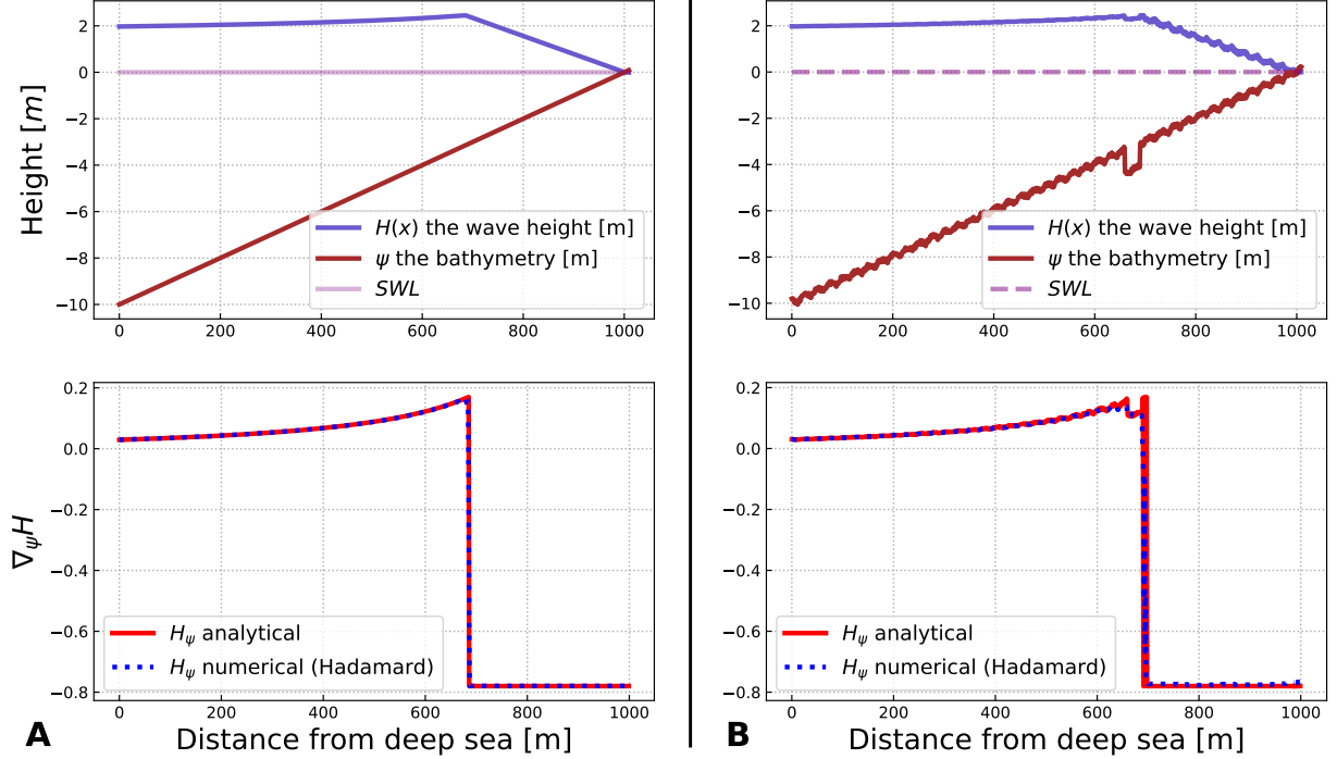
Figure 3.4 – Comparison of numerical and analytical solution of \nabla_{\psi}H using OptiMorph model. Configuration without (A) / with (B) perturbations, H_0 = 2 m, h_0 = 10 m and the wave period T_0 = 10 s. In dodgerblue, the wave height H , in brown the bottom profile \psi , in red \nabla_{\psi}H calculated analytically, in blue \nabla_{\psi}H calculated by Hadamard strategy.
