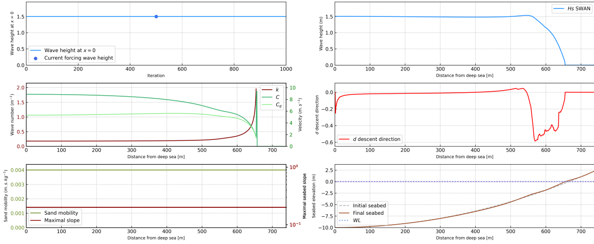
Example Simulation 1D of storm in convex bathymetry with tide Parameters: H_0 = 1.5 \text{ m} - T_0 = 6 \text{ s} - h_0 = 10 \text{ m} Iteration = 500 / 999
