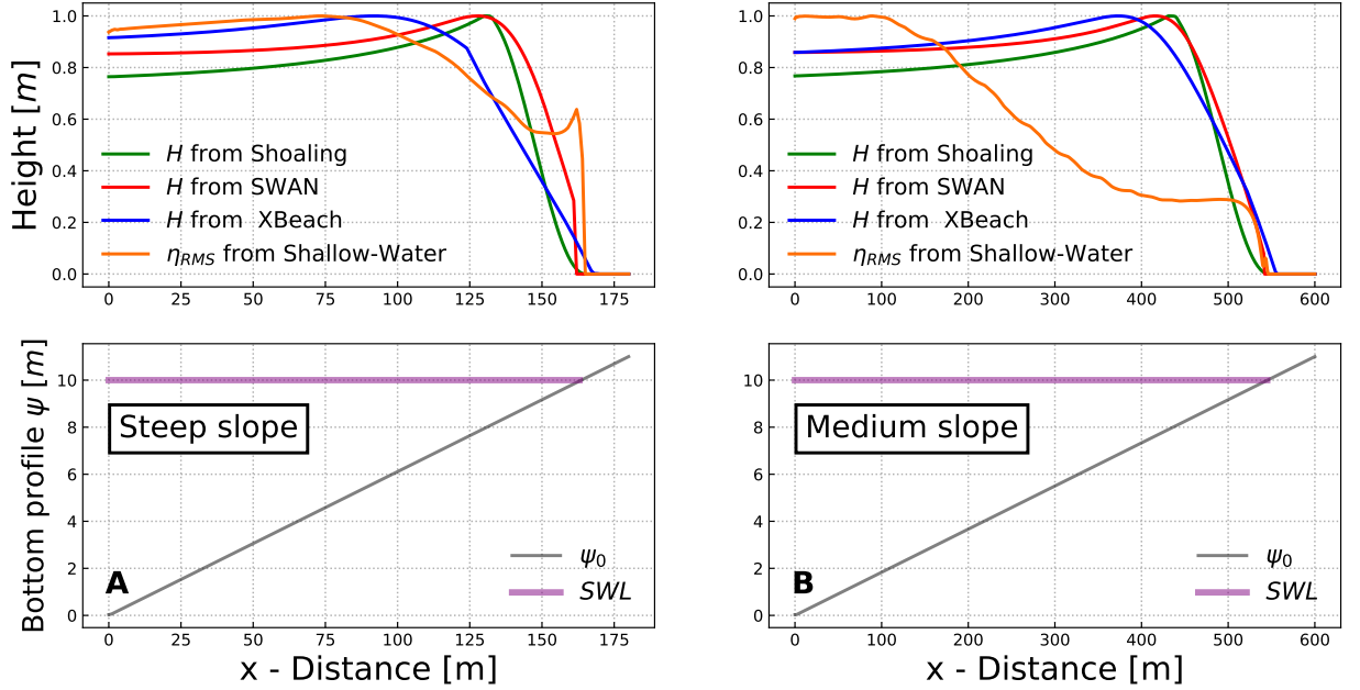
Figure 3.12 – Comparison between H from models Shoaling (green), SWAN (red) XBeach (blue) and \eta_{RMS} from Shallow-Water (orange) models. H and \eta_{RMS} are on the same scale. A) Simulation parameters of H_0 = 1.5 m, T_0 = 8 s, h_0 = 20 m, \Omega = 180 m. B) Simulation parameters of H_0 = 1.5 m, T_0 = 8 s, h_0 = 20 m, \Omega = 600 m.
