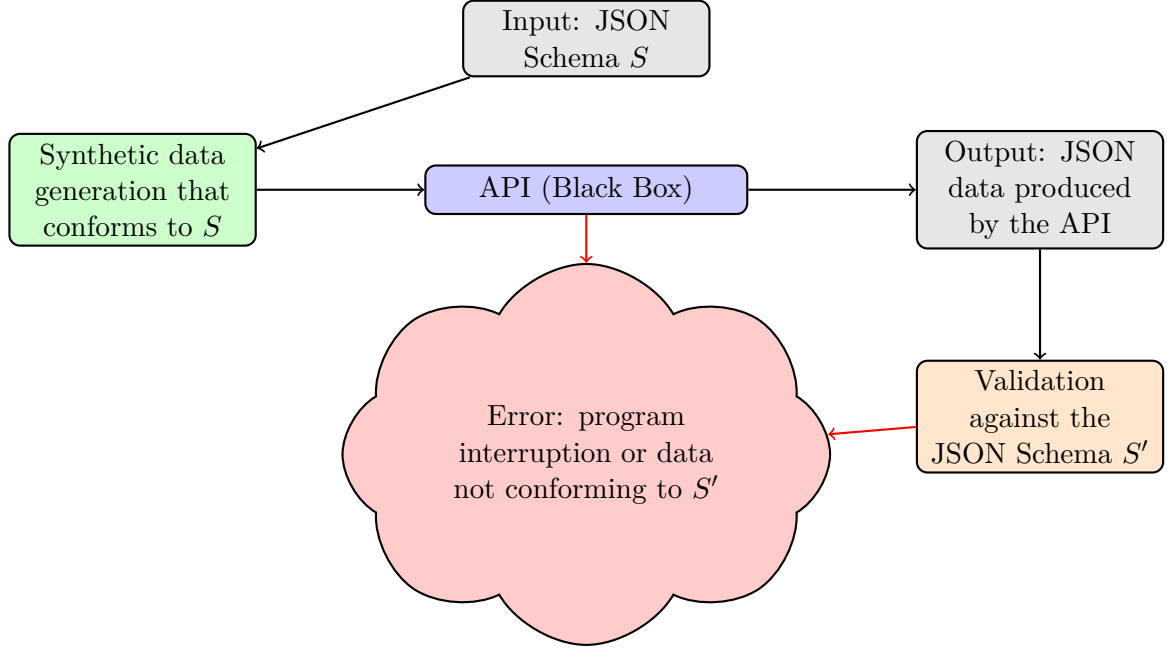
Figure 1.1: Black box testing of JSON-based web APIs
