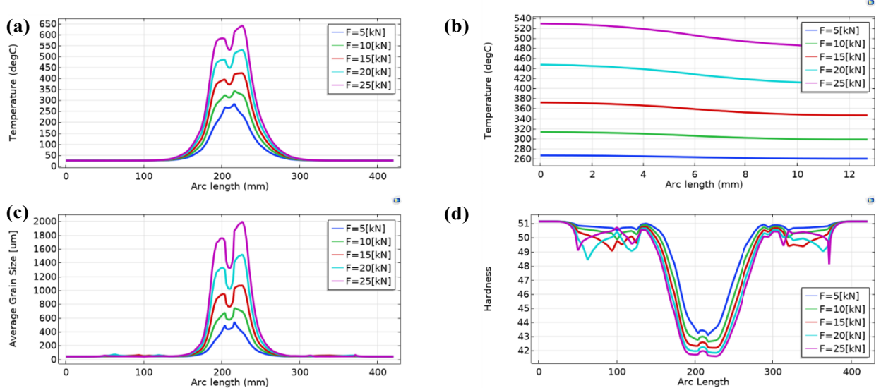
Figure 3-3: Al Workpiece, parametric analysis on normal force. a) temperature in x-direction, b) temperature in z-direction, c) average grain size, and d) hardness
