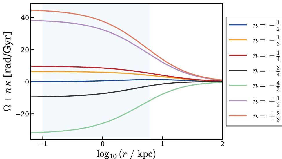
Figure 4.13: Behavior of \Omega + n\kappa for our background potential.
