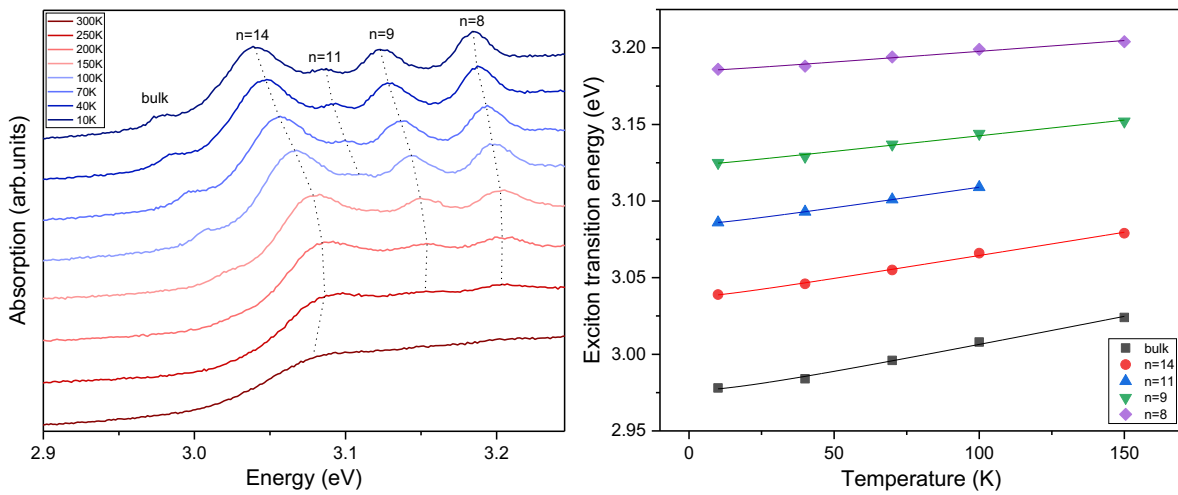
Figure 3.4: Left side: Absorption spectra of a CsPbCl 3 nanocubes ensembles taken at temperatures ranging from 300 to 10 K. The closest number of monolayer matching their energy at 10 K is provided according to the simulations presented in Fig. 3.5. Right side: The energy of each absorption transition is followed with temperature. The experimental points are fitted with a Varshni law presented in the text.
