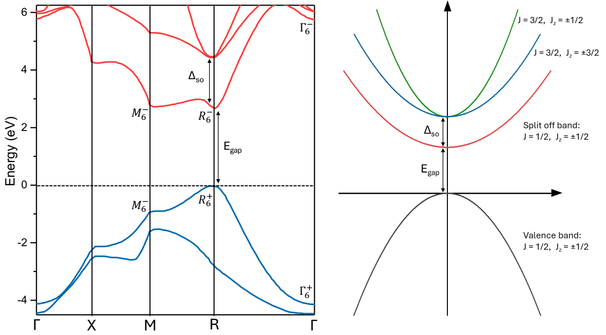
Figure 1.4: Left: Energy band structure of bulk \text{CsPbCl}_3 obtained from a 40-band \mathbf{k} \cdot \mathbf{p} model, adapted from Steinmetz et al. [53]. The authors found here a bulk band gap energy of E_g = 2.7 eV and a spin orbit coupling parameter value of \Delta_{SO} = 1.6 eV. Right: illustration of the simplified band structure around the R point of the first Brillouin zone.
