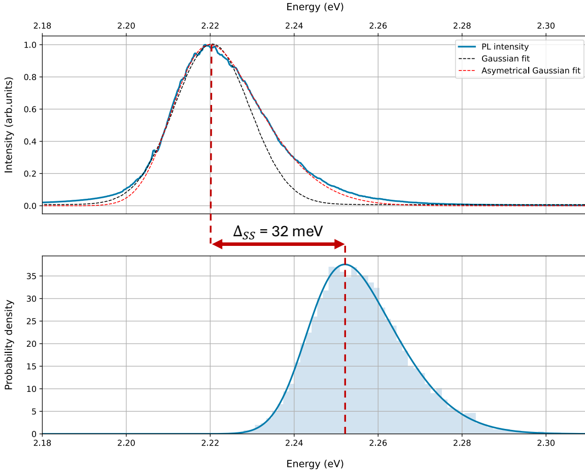
Figure 5.10: Top: The experimental PL spectrum of an ensemble of FAPbBr 3 NCs captured at T = 7 K (blue solid line). The best Gaussian (black dashed line) and asymmetrically stretched Gaussian (dashed red line) adjustments are also provided on the same graph. Bottom: The skew normal distribution (given by the red curve of the graph on the top) is translated of \Delta_{SS} = 32 meV, (Stokes-shift) and is used to generate an histogram of the absorption transition energies of the simulated NCs on the grid.
