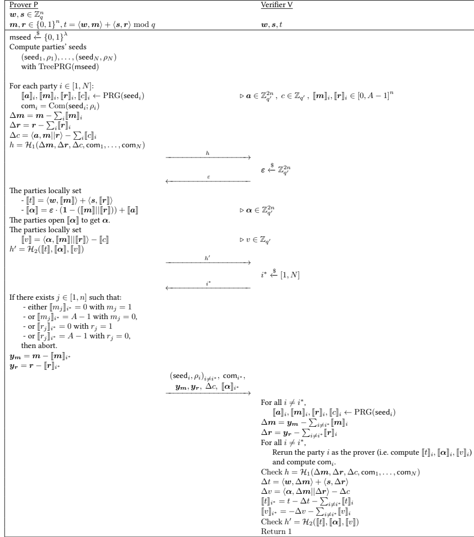
Protocol 7: Zero-knowledge argument for string-commitment using batch product verification to prove binarity.
