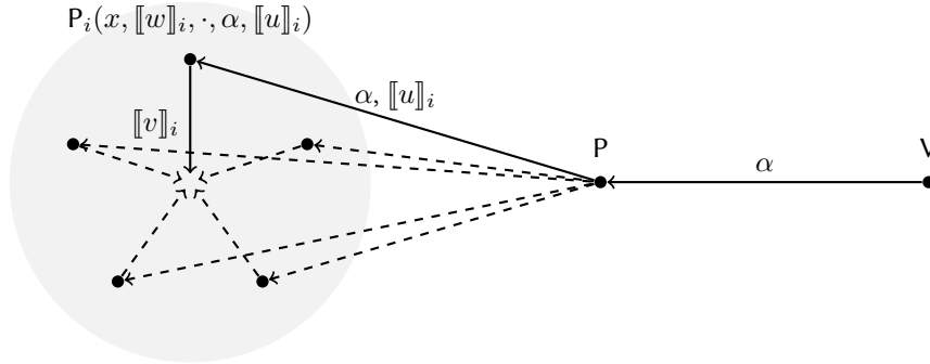
Fig. 3.1: Informal overview of party P_i computation during one round: the challenge \alpha corresponds to type (i) action, the new sharing [[u]] to (ii), and [[v]]_i = g(\cdot, \alpha, [[u]]_i) to (iii), where g is a linear function. The \cdot may be substituted by previous broadcasts, and challenges.
