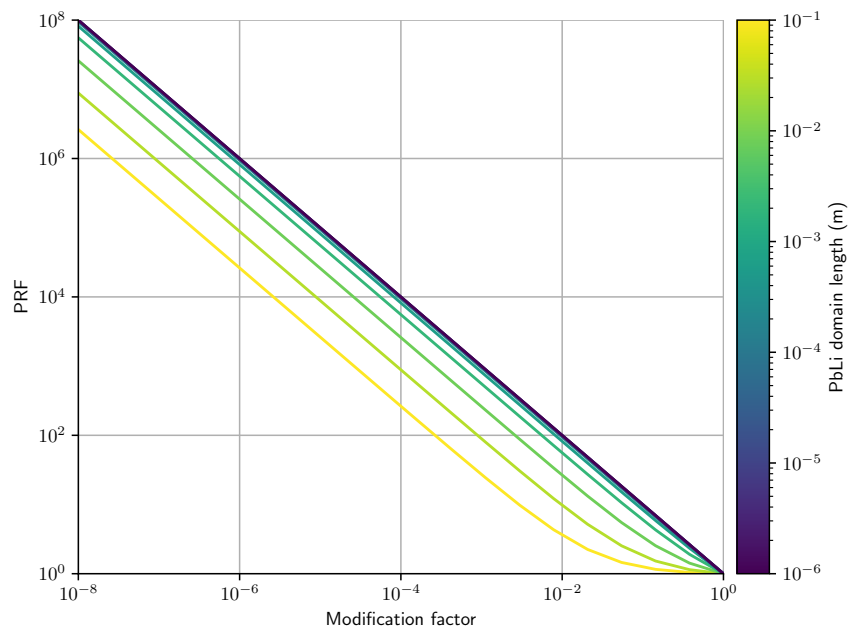
Figure 5.10: Measured PRF compared to a standard material interface condition against modification factor for Eurofer solubility, varying the length of the PbLi
