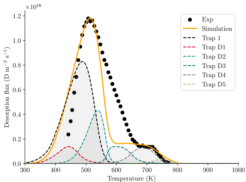
Figure D.2: TDS data for tungsten sample damaged to 0.001 dpa, fitted using one intrinsic trap and five extrinsic traps
