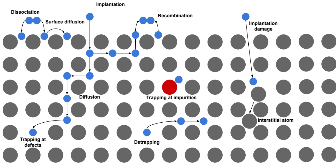
Figure 1.9: Interactions of solute hydrogen isotopes in metals [44]
