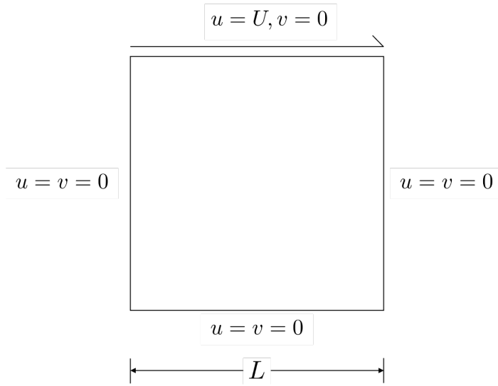
Figure A.1: Lid driven cavity problem
