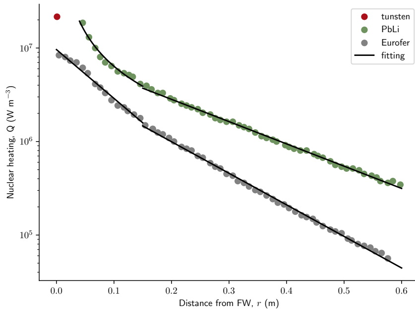
Figure 3.6: Nuclear heating in the PbLi and Eurofer by radial length, r [106]
