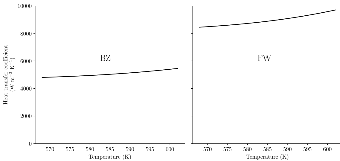
Figure 3.19: Heat transfer coefficient values across the WCLL unit in the BZ pipes (left) and the FW channels (right)
