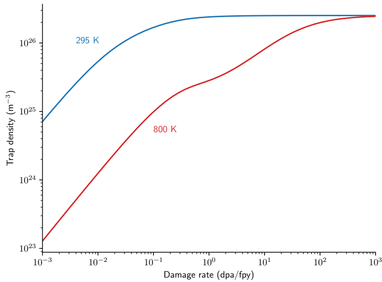
Figure 4.7: Total trap densities at 295 K and 800 K with variation in the damage rate after one FPY.
