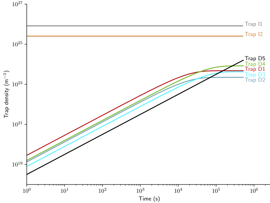
Figure 4.13: Temporal evolution of trap concentration of damaged induced traps D1-D5 as a result of a damage at 5 dpa/fpy, using an average temperature of 684 K, compared to intrinsic traps concentrations
