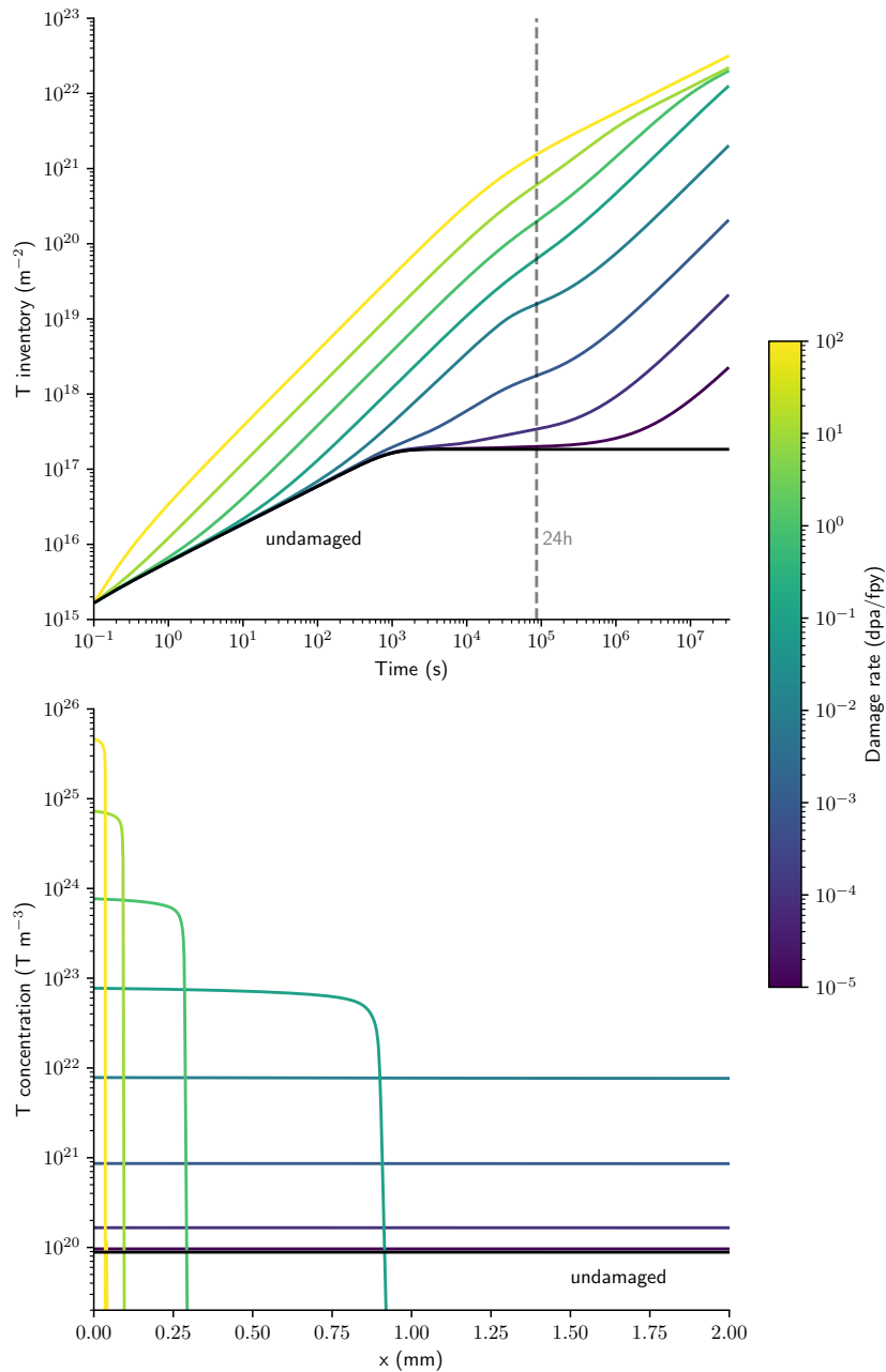
Figure 4.8: Tritium inventory over 1 FPY (top) and the retention distribution after 24 h (bottom) from simultaneous damage exposure and tritium implantation, at 700 K varying the damage rate.
