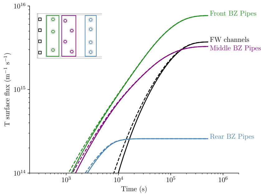
Figure 4.11: Temporal evolution of the tritium fluxes at the cooling surfaces for the first wall cooling channels and breeding zone pipes at the front, middle and rear position relative to the plasma facing surface. Dashed lines correspond to the standard case without trapping effects
