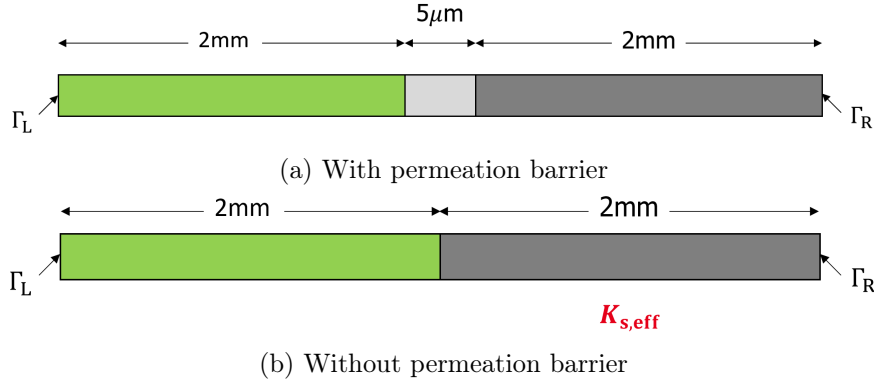
Figure 5.7: Cartesian 1D model of a domain of 2 mm PbLi ■ and 2 mm Eurofer ■ with and without a 5 \mu\text{m} \text{Al}_2\text{O}_3 ■ permeation barrier
