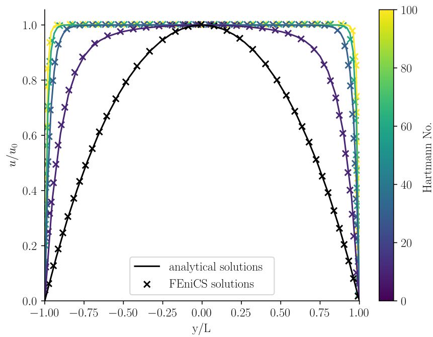
Figure C.3: Fully insulated case ( \frac{\partial \Phi}{\partial x} = 0 on \Gamma_{HW} ) compared to analytical solutions [246]
