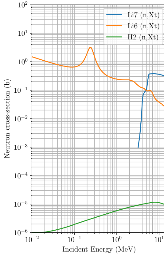
Figure 1.7: Cross-section of neutron capture reactions in barns with Li-7 Li-6 and H2 producing tritium [40]
