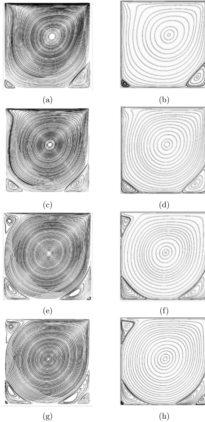
Figure A.2: Re = 400 (a), Re = 1000 (c), Re = 5000 (e), Re = 10000 (g), compared to its respective counterpart reference solution (b), (d), (f) and (h) [164]
