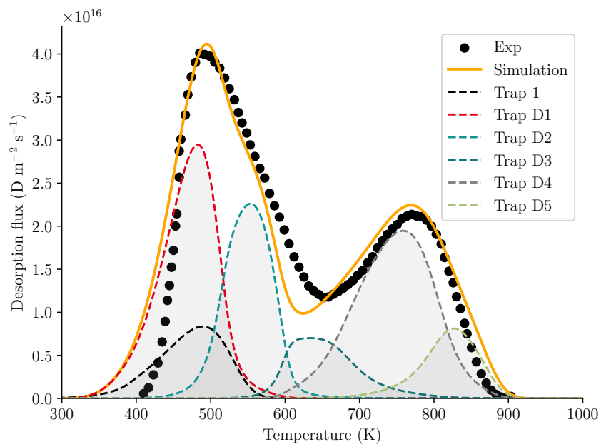
Figure D.4: TDS data for tungsten sample damaged to 0.023 dpa, fitted using one intrinsic trap and five extrinsic traps
