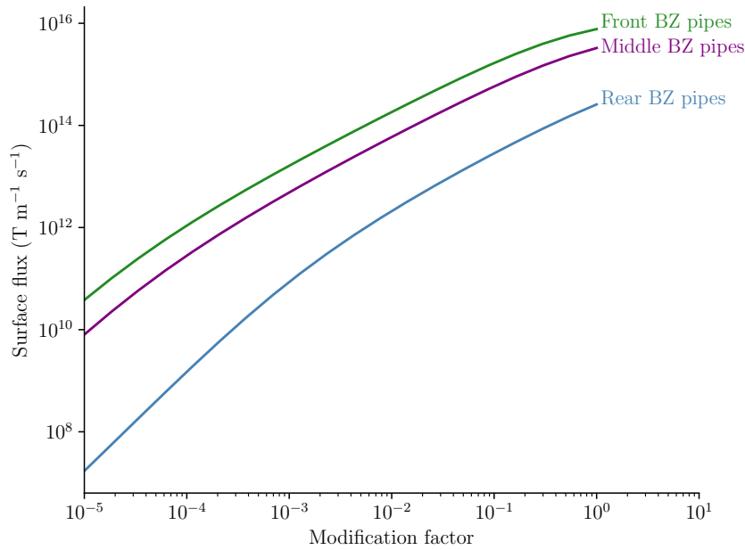
Figure 5.12: Tritium surface flux entering the different regions of BZ pipes at steady state varying the modification factor applied to the solubility value of the Eurofer in the BZ pipes. For colours, see figure 5.4a
