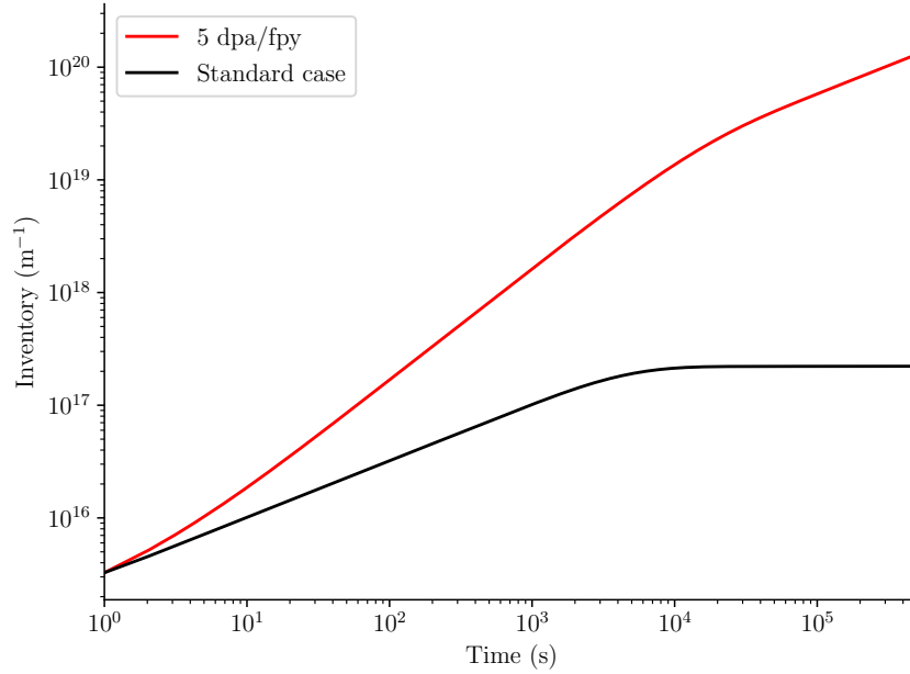
Figure 4.14: Temporal evolution of tritium retention in tungsten FW as a result of damage at 5 dpa/fpy, relative to an undamaged case
