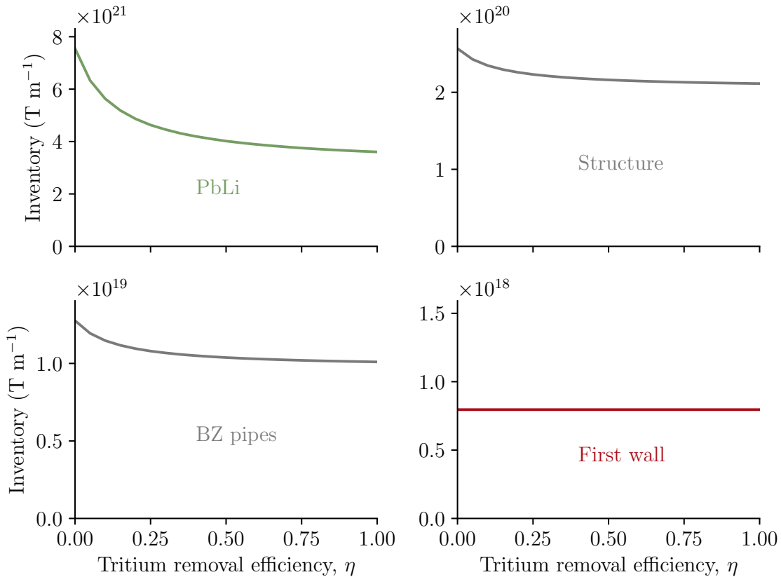
Figure 5.3: Tritium inventories in the PbLi, structure, BZ pipes and FW as a function of tritium re-entering the WCLL. Standard case at \eta = 1.0
