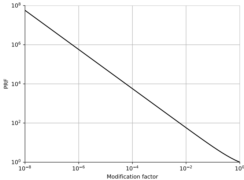
Figure 5.9: Measured PRF compared to a standard material interface condition against modification factor for Eurofer solubility
