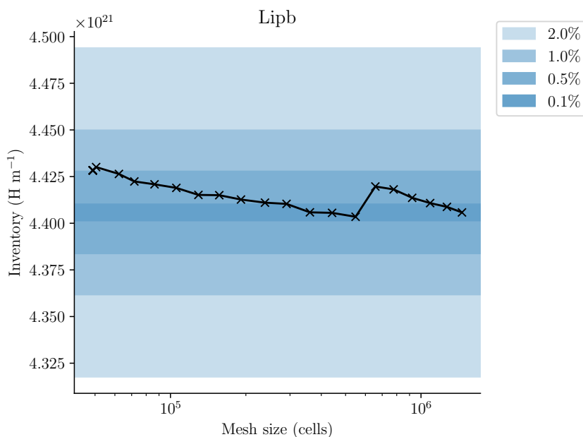
Figure B.4: Tritium inventories with increasing mesh size in the PbLi subdomain
