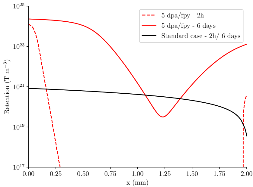
Figure 4.15: Tritium retention profile across the tungsten FW comparing the standard case against one considering trap creation after 2 h and 6 days of exposure to a damage rate of 5 dpa/fpy
