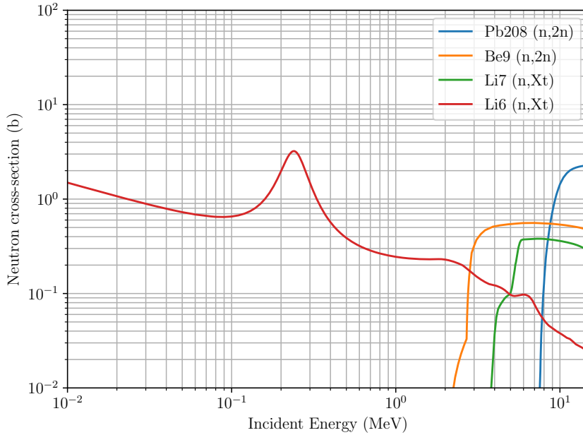
Figure 1.8: cross-section of neutron capture reactions with Pb and Be compared to lithium isotopes [40]
