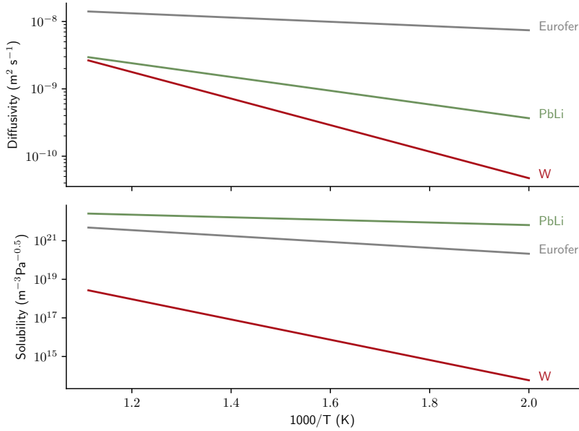
Figure 3.5: Hydrogen transport properties of diffusivity (top) and solubility (bottom) of the materials in the WCLL: tungsten [124], Eurofer [126] and PbLi [190, 125] over a temperature range found within the operational conditions of the WCLL and beyond
