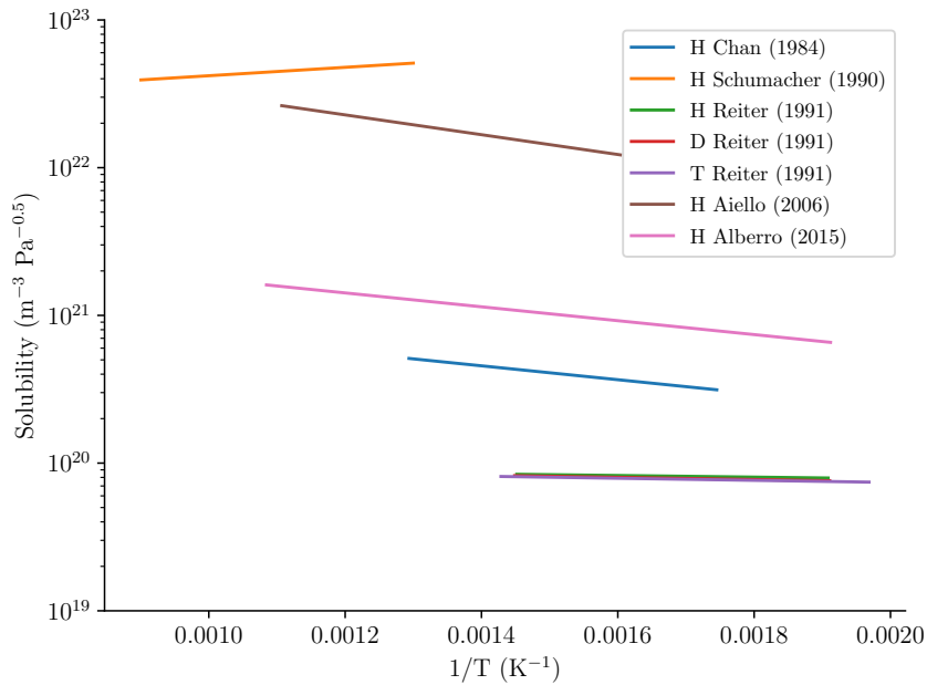
Figure 3.25: Solubilities for hydrogen isotopes H, D and T in PbLi [198, 199, 190, 125, 200]. Values obtained from HTM [201]
