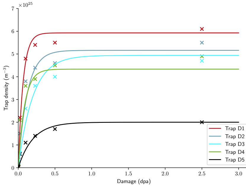
Figure 4.6: Trap concentrations with increasing damage dose from the fitted TDS, then fitted using the current model.
