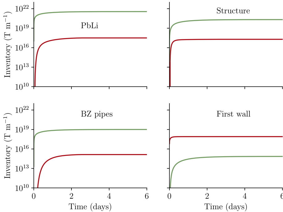
Figure 3.24: Temporal evolution of the tritium inventory in the PbLi, FW, BZ pipes and structure divided into contributions from the plasma ■ and the breeder ■
