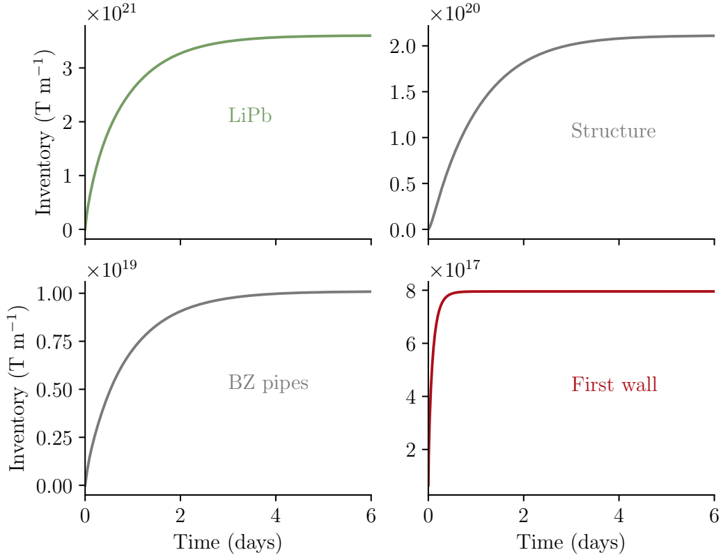
Figure 3.14: Temporal evolution of the tritium inventories in the PbLi, structure, BZ pipes and first wall
