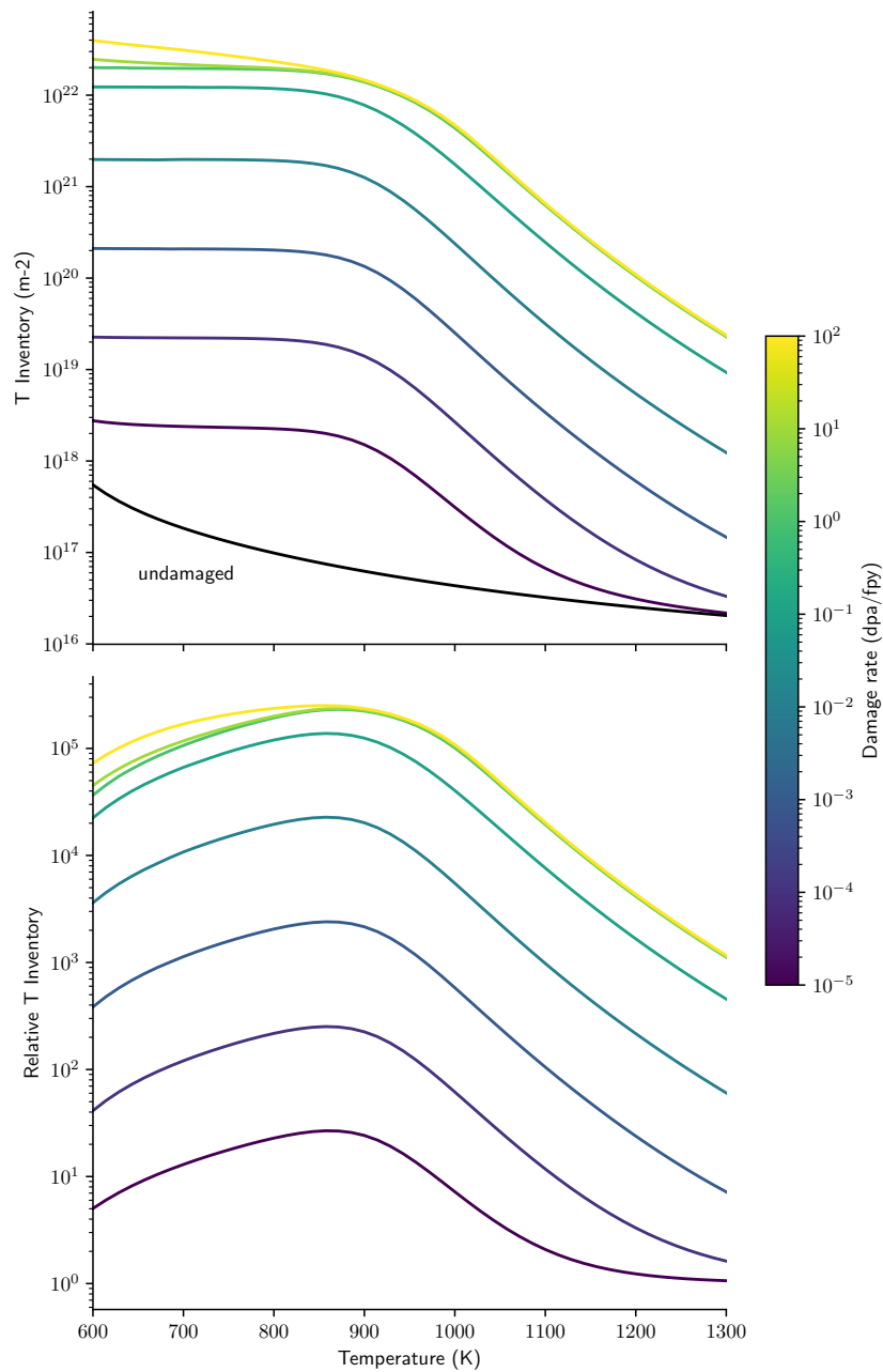
Figure 4.9: Tritium retention in tungsten in varying damaged cases, relative to an undamaged case, after 1 FPY varying temperature.
