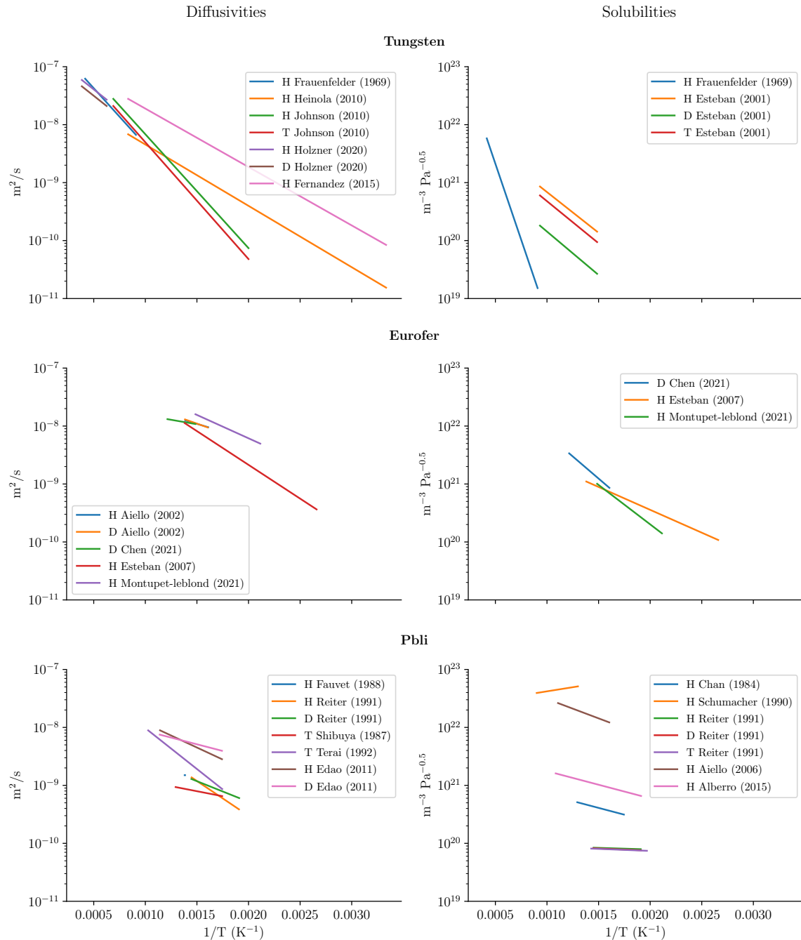
Figure 3.4: Diffusivities and solubilities for hydrogen isotopes H, D and T in tungsten [124, 61, 68, 136, 59, 192], Eurofer 97 [193, 126, 134, 54] and PbLi [194, 190, 195, 196, 197, 198, 199, 125, 200]. Values obtained from HTM [201]
