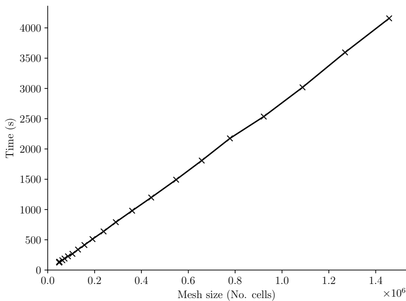
Figure B.3: Time to run steady state simulation with increasing mesh size
