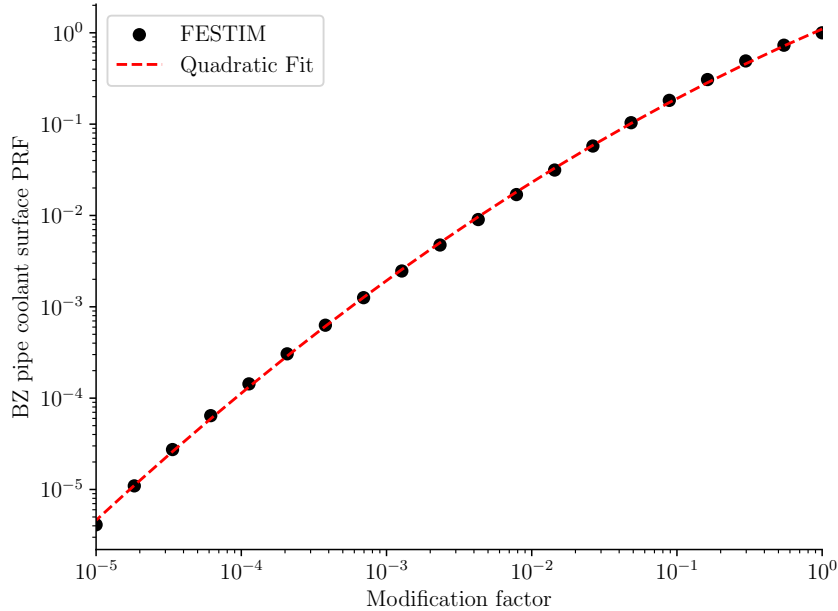
Figure 5.13: The measured PRF of the total BZ pipe surface flux against the standard flux, against respective modification factor, with quadratic fitting
