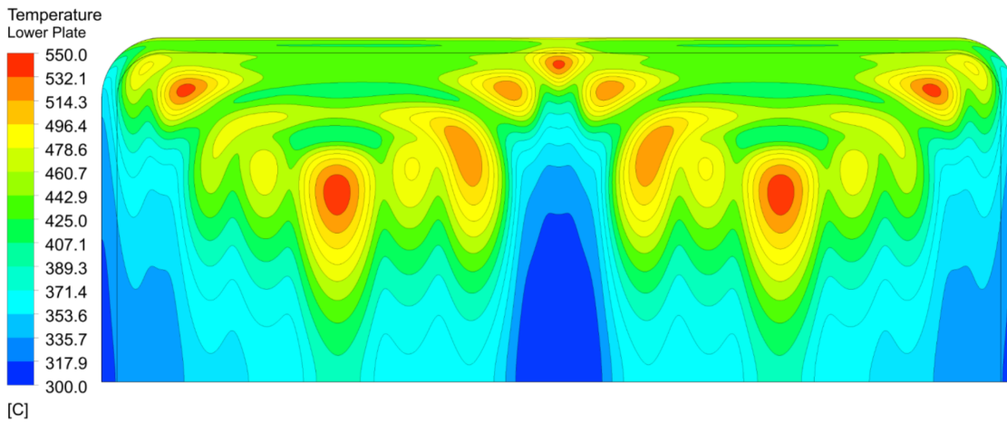
Figure 1.14: WCLL v0.6B thermal field [87]
