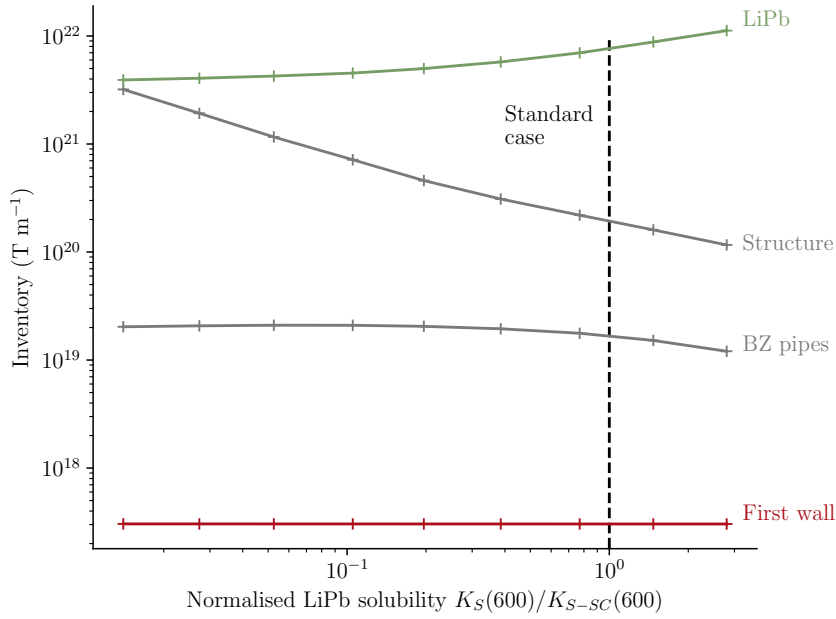
Figure 3.26: Evolution of the steady state tritium inventories as a function of hydrogen solubility, K_S , in PbLi normalised to the standard case solubility, K_{S-SC}
