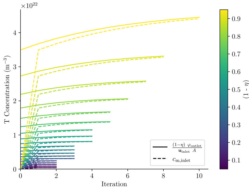
Figure 5.2: Tritium concentration of the inlet, c_{m,\text{inlet}} , with resulting evaluation for contraction to use in next iteration, ((1 - \eta) \varphi_{\text{outlet}})/(\mathbf{u}_{\text{inlet}} A) , converging to a max difference of 1%, for each case of (1 - \eta)
