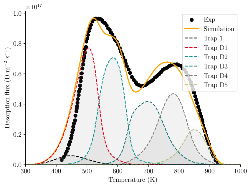
Figure D.8: TDS data for tungsten sample damaged to 2.5 dpa, fitted using one intrinsic trap and five extrinsic traps
