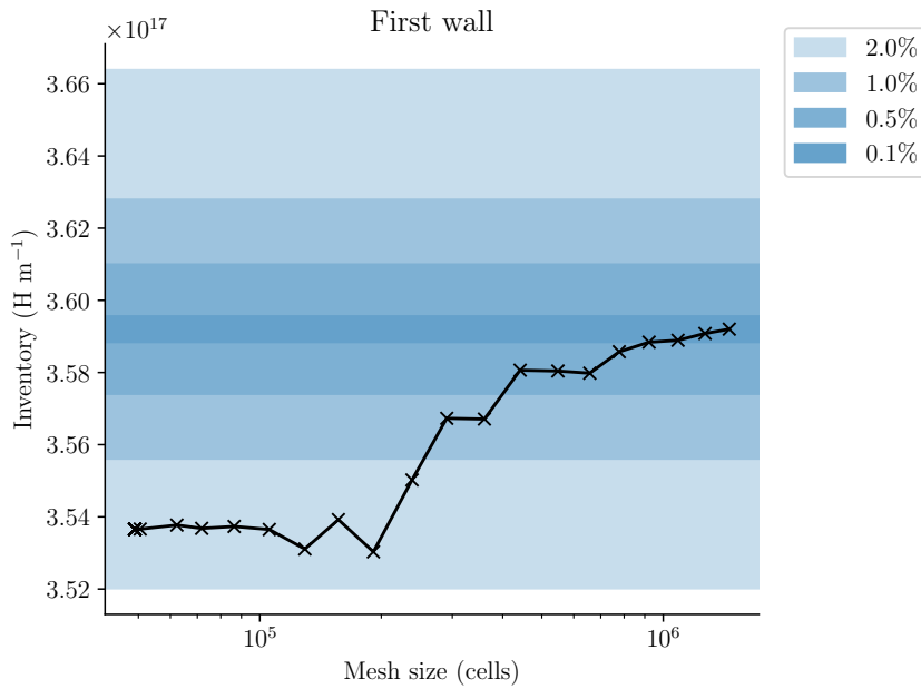
Figure B.6: Tritium inventories with increasing mesh size in the FW domain
