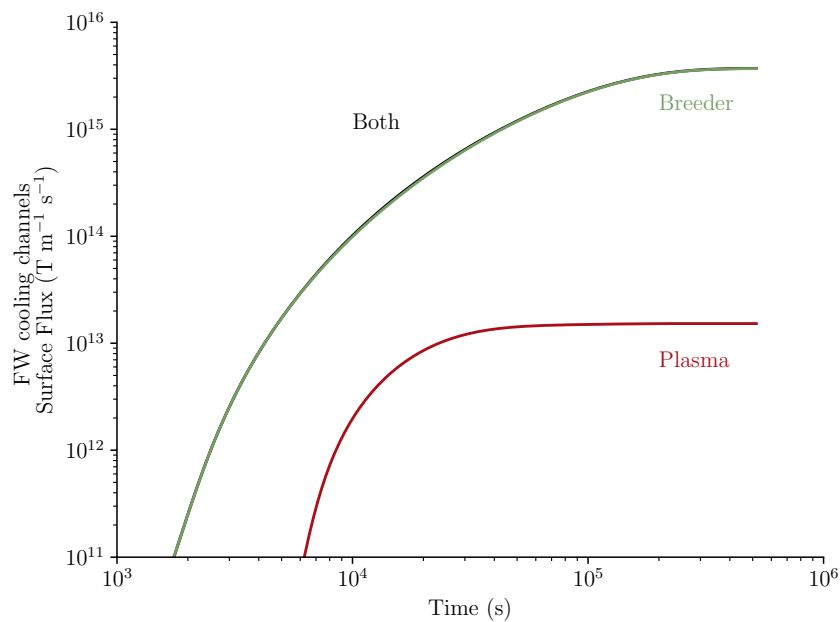
Figure 3.23: Surface flux at the first wall cooling channels divided into contributions from the plasma ■ , from the breeder ■ , and both together ■
