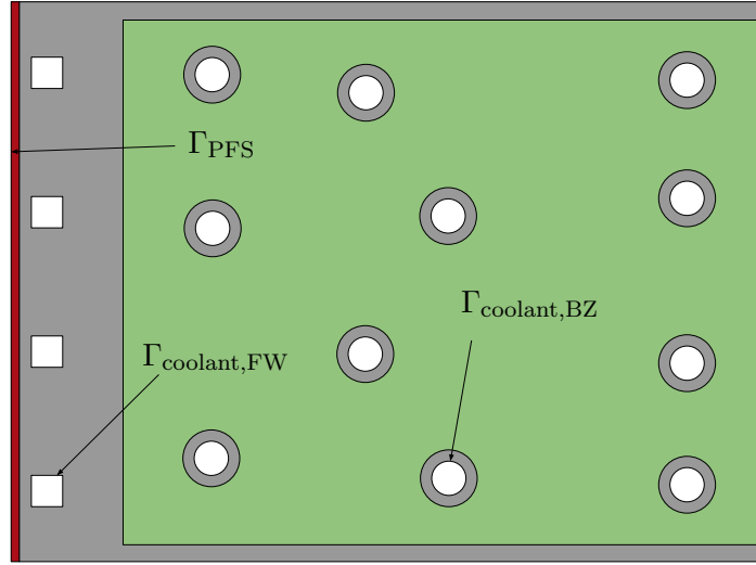
Figure 3.7: Front end of 2D WCLL geometry showing tungsten ■ , Eurofer ■ , LiPb ■ . \Gamma represents a defined surface, PFS is the Plasma Facing Surface, FW is the First Wall, and BZ is the Breeding Zone
