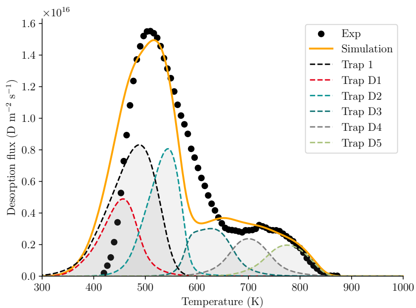
Figure D.3: TDS data for tungsten sample damaged to 0.005 dpa, fitted using one intrinsic trap and five extrinsic traps
