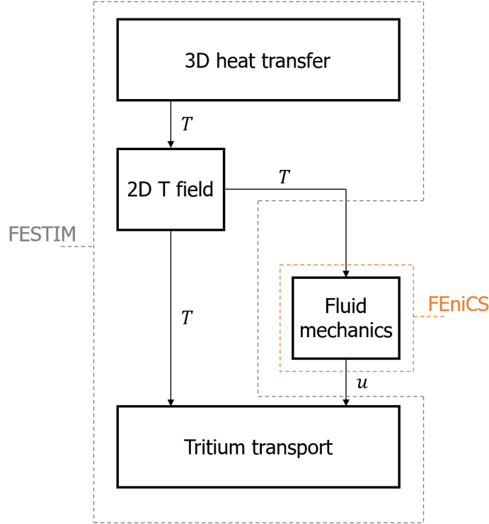
Figure 3.1: Simulation workflow for multiphysics modelling of the WCLL, highlighting in dashed lines which physics is solved by FESTIM and FEniCS
