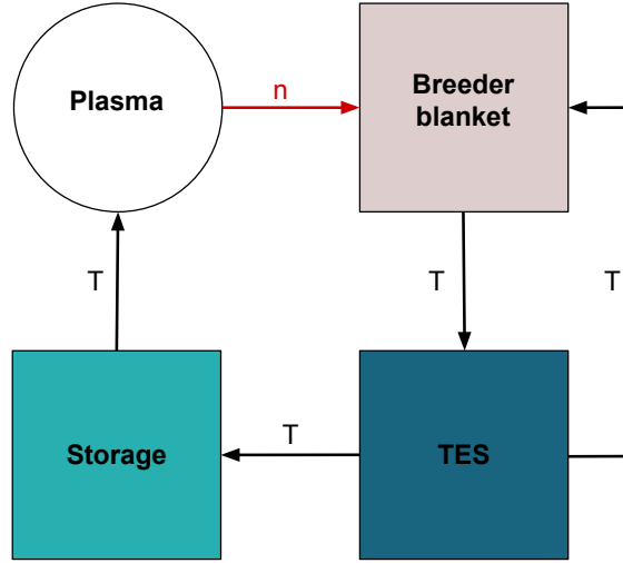
Figure 1.5: A schematic process diagram for a simplified fuel cycle
