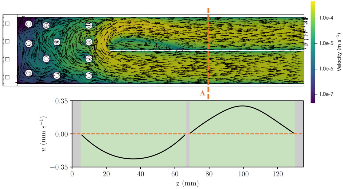
Figure 3.11: Steady state velocity field with associated profile A across the PbLi █ channels and Eurofer █ structure
