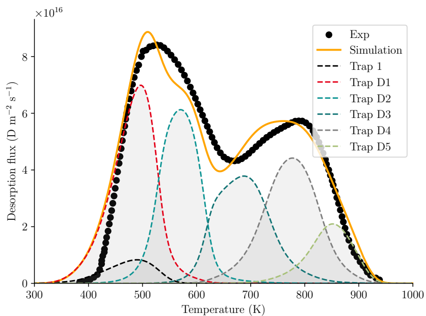
Figure D.7: TDS data for tungsten sample damaged to 0.5 dpa, fitted using one intrinsic trap and five extrinsic traps
