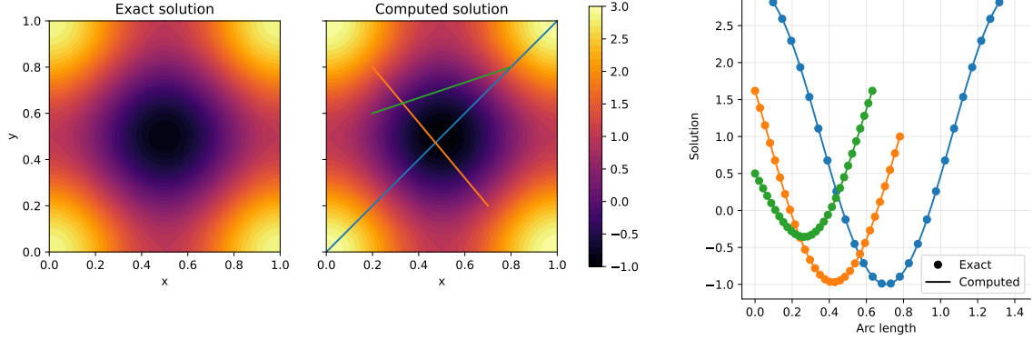
Figure 2.7: Verification case 2: heat transfer [150]
