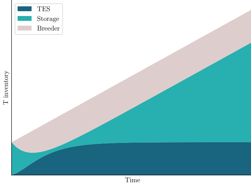
Figure 1.6: Tritium inventory changes over time in the TES, storage and breeder
