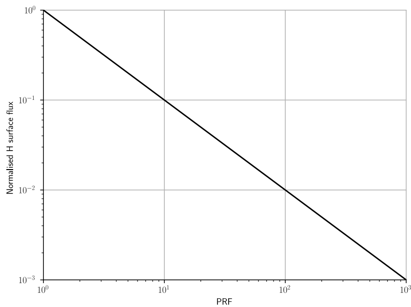
Figure F.2: Measured PRF compared to a recombination flux boundary condition against an enforced PRF value
