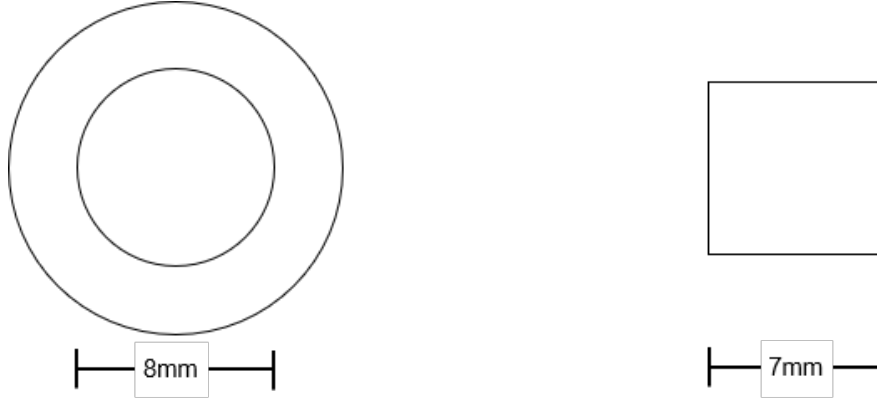
Figure 3.16: BZ cooling pipe (left) and FW cooling channel (right) dimensions
