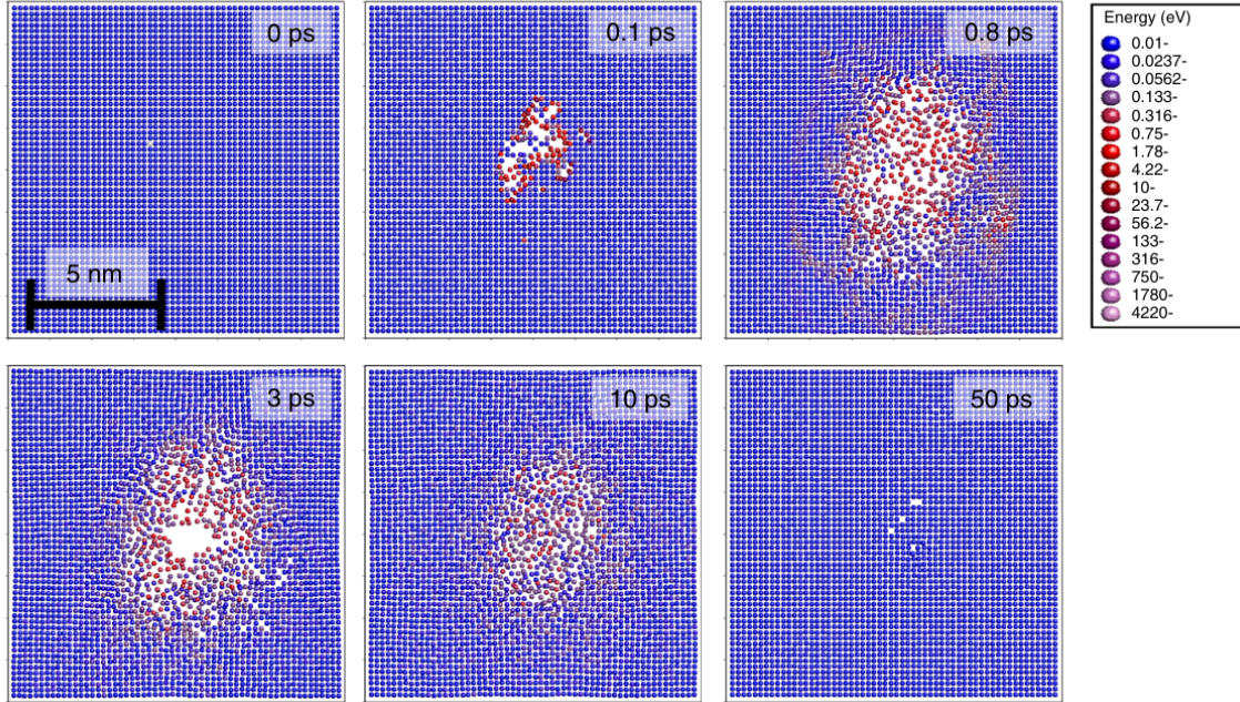
Figure 1.12: A cross-sectional view of a collision cascade in gold, induced by a 10 keV primary knock-on atom [91]
