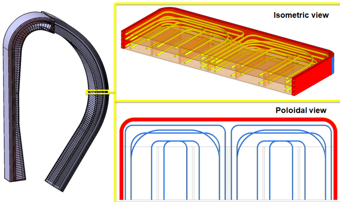
Figure 1.11: WCLL v0.6B COB equatorial elementary cell in isometric and poloidal views [87]
