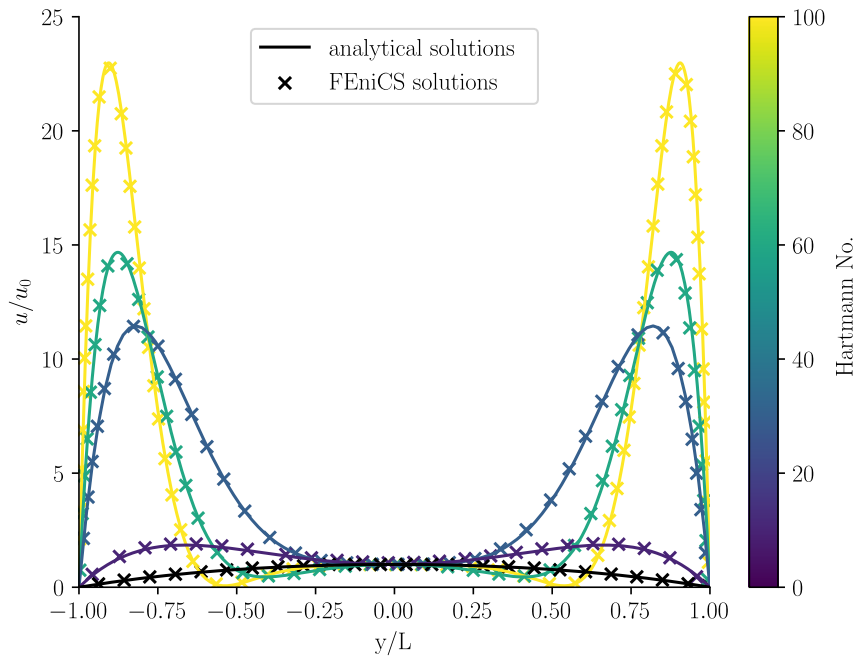
Figure C.2: Fully conductive case ( \Phi = 0 on \Gamma_{\text{HW}} ) compared to analytical solutions [245]
