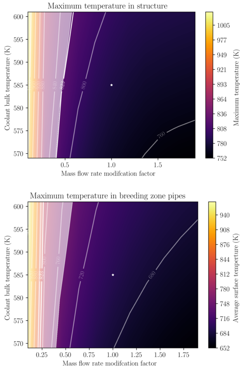
Figure 3.21: Maximum temperature observed in the Eurofer in the structure (top) and BZ pipes (bottom) as a result of varying the heat transfer coefficient as a function of bulk coolant temperature and mass flow rate. Values from the standard case are highlighted in the centre with a white star
