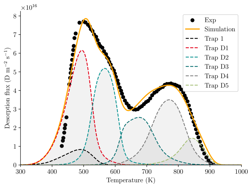
Figure D.5: TDS data for tungsten sample damaged to 0.1 dpa, fitted using one intrinsic trap and five extrinsic traps
