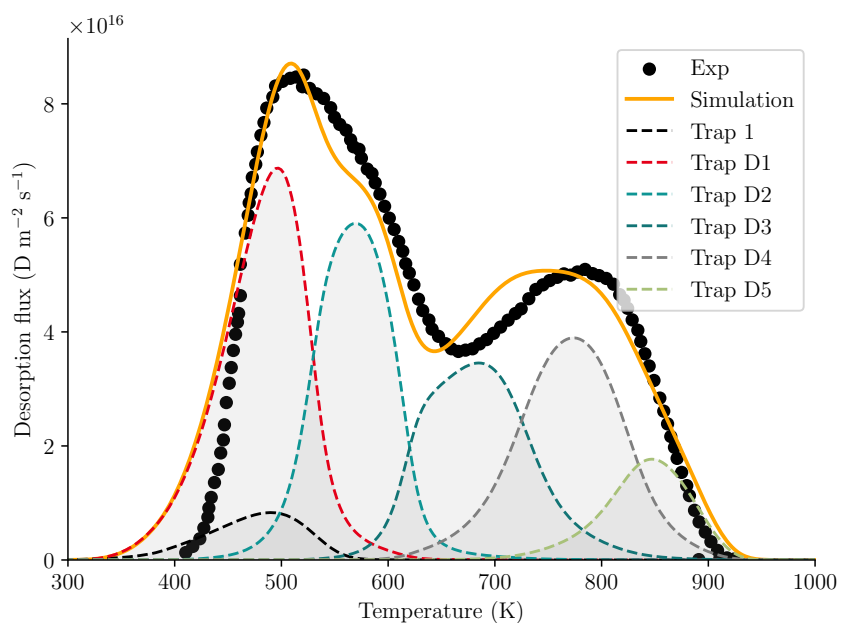
Figure D.6: TDS data for tungsten sample damaged to 0.23 dpa, fitted using one intrinsic trap and five extrinsic traps
