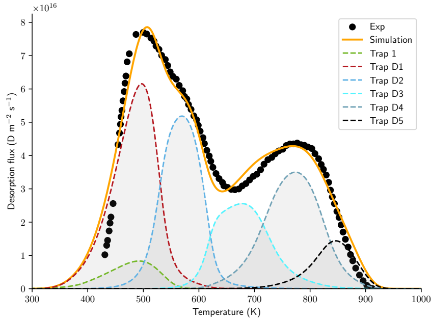
Figure 4.5: TDS data for tungsten sample damaged to 0.1 dpa, fitted using one intrinsic trap and five extrinsic traps
