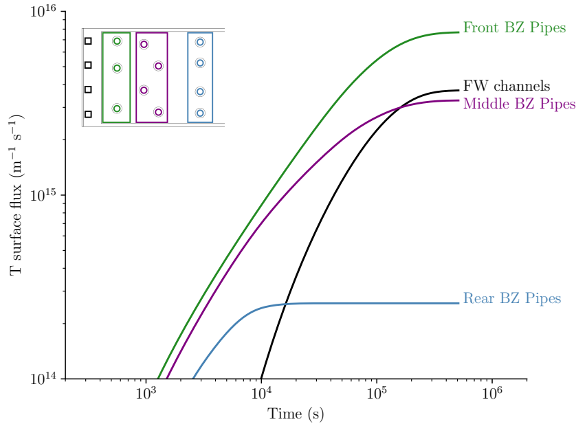
Figure 3.15: Temporal evolution of the tritium permeation rate at the cooling surfaces for the first wall cooling channels and breeding zone pipes at the front, middle and rear position relative to the plasma facing surface
