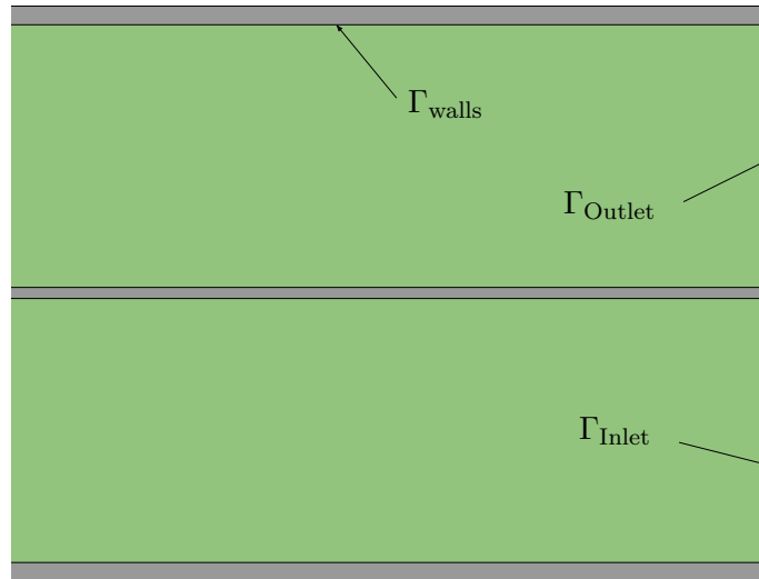
Figure 3.8: Rear end of 2D geometry showing Eurofer ■ , LiPb ■ . \Gamma represents a defined surface, \Gamma_{\text{walls}} applies to all LiPb/Eurofer interfaces.
