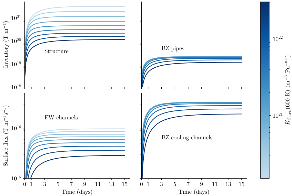
Figure 3.27: Influence of the solubility of hydrogen in PbLi on the temporal evolution of tritium inventory (top) and surface flux (bottom). The solubility at 600 K varies from 1.5 \times 10^{20} to 3.0 \times 10^{22} \text{ m}^{-3} \text{ Pa}^{-0.5} .
