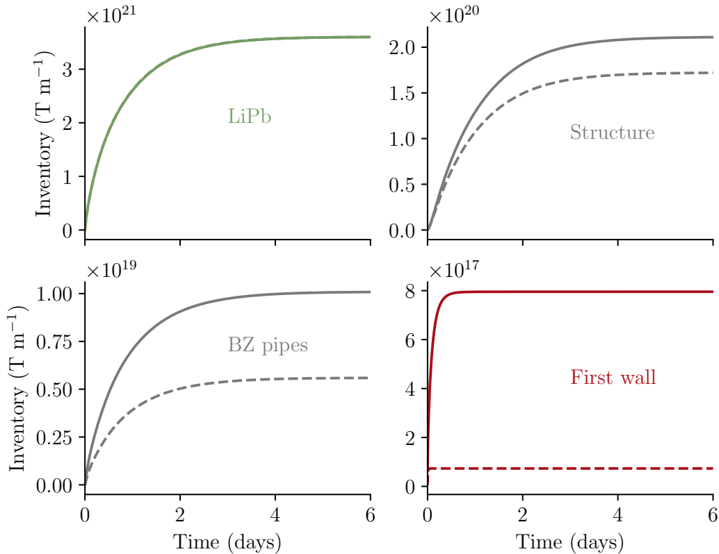
Figure 4.10: Temporal evolution of the tritium inventory in the PbLi, FW, BZ pipes and structure. Dashed lines correspond to a case without traps.
