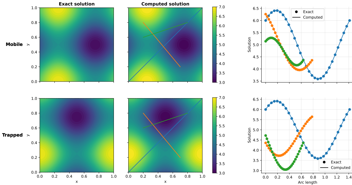
Figure 2.8: Verification case 3: trapping [150]
