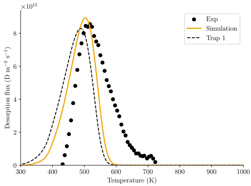
Figure D.1: TDS data for tungsten sample damaged to 0 dpa, fitted using one intrinsic trap
