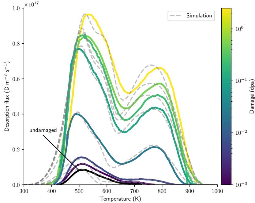
Figure 4.4: Results of TDS analysis from tungsten samples damaged to various levels (0.001 - 2.5 dpa at 800 K and decorated with D at 370 K
