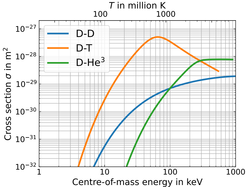
Figure 1.2: Fusion reaction cross-sections [5]
