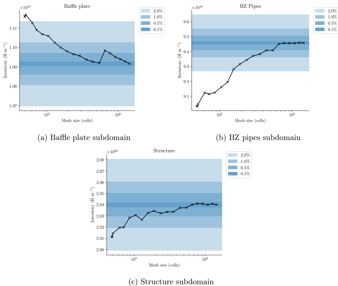
Figure B.5: Tritium inventories with increasing mesh size in the eurofer subdomains
