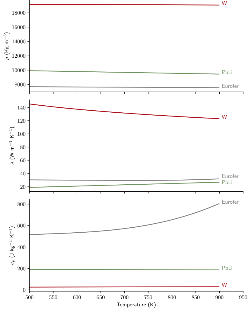
Figure 3.3: Thermophysical properties of density, \rho (top), thermal conductivity, \lambda (middle) and specific heat capacity, c_p (bottom) of the materials in the WCLL: tungsten [141], Eurofer [189] and PbLi [140] over a temperature range found within the operational conditions of the WCLL and beyond
