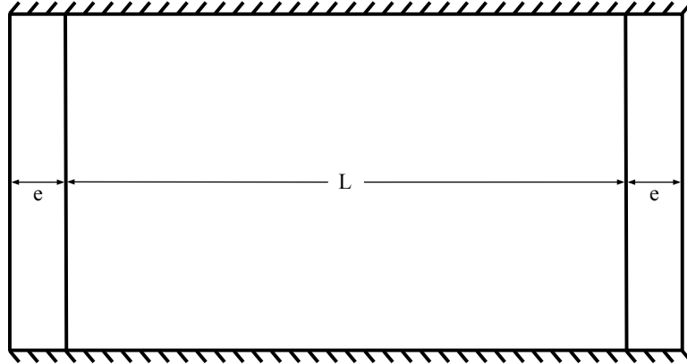
Figure 5.5: 2D representation of the 1D cartesian geometry for permeation barrier analytical solution
