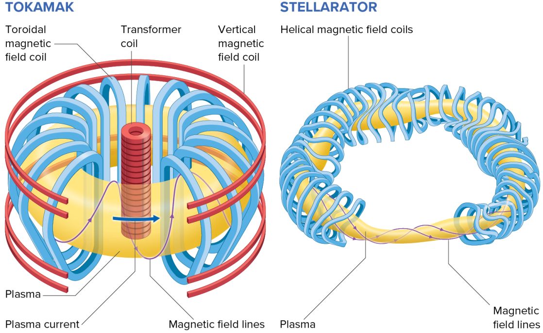
Figure 1.3: Tokamak reactors (left) and related designs known as stellarator reactors (right) both confine the plasma (yellow) with magnetic fields (purple) that are generated by electromagnetic coils (blue and red) [10]
