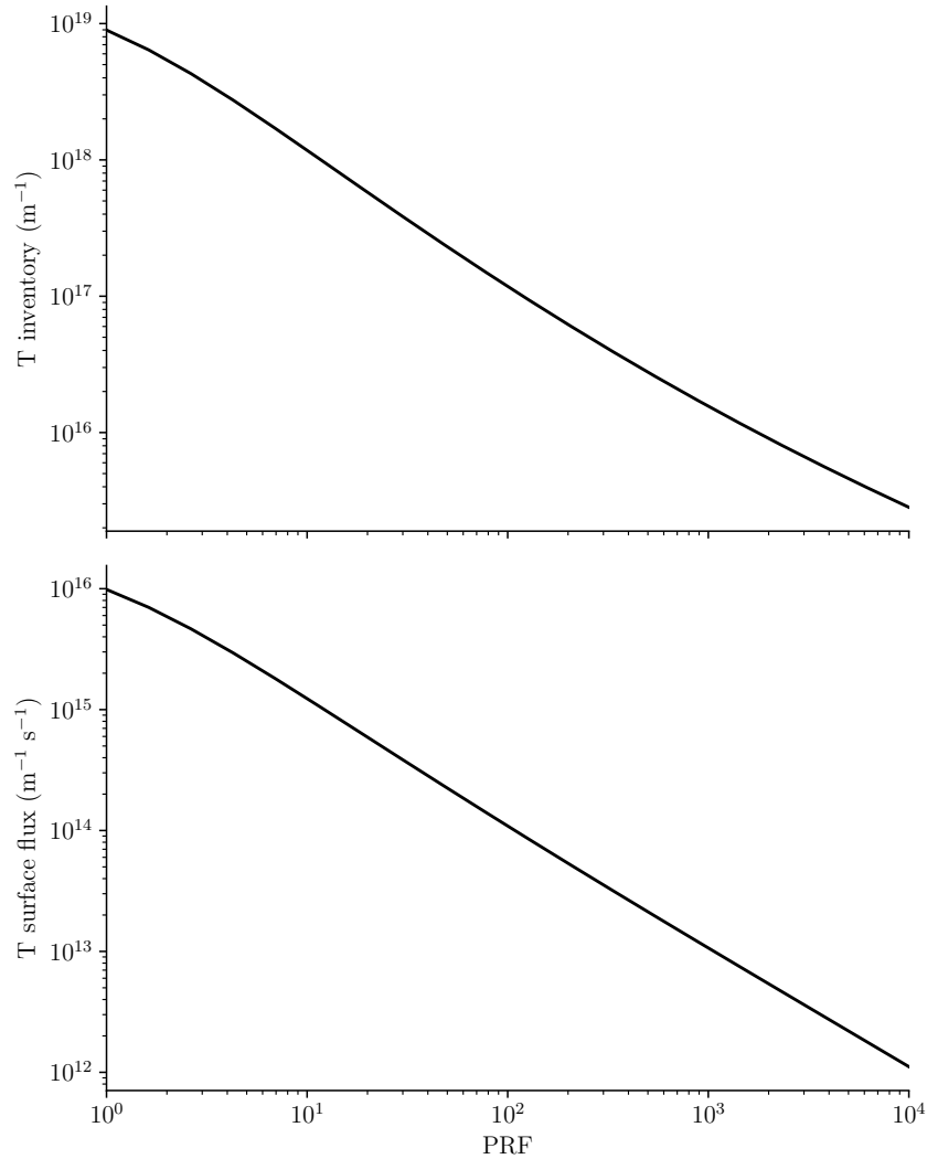
Figure 5.14: Steady-state tritium inventories in the BZ pipes (top) and surface flux at the BZ pipes coolant interfaces (bottom), varying the enforced PRF
