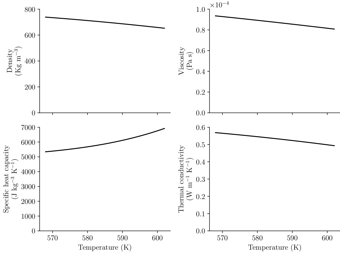
Figure 3.17: Variation of density, viscosity, specific heat capacity and thermal conductivity of water in the temperature range observed in the WCLL
