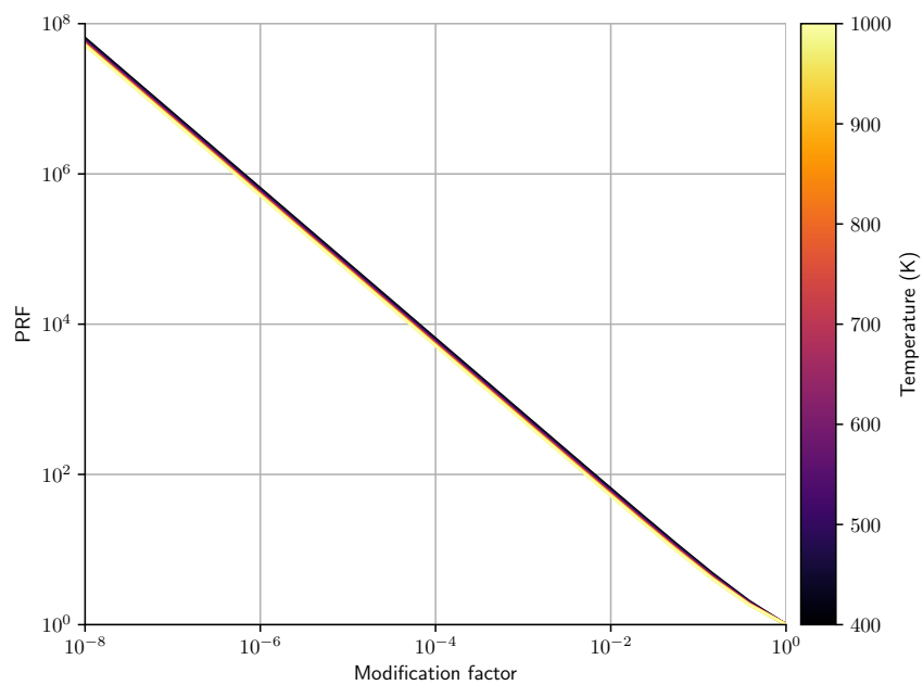
Figure 5.11: Measured PRF compared to a standard material interface condition against modification factor for Eurofer solubility, varying the temperature of the domain
