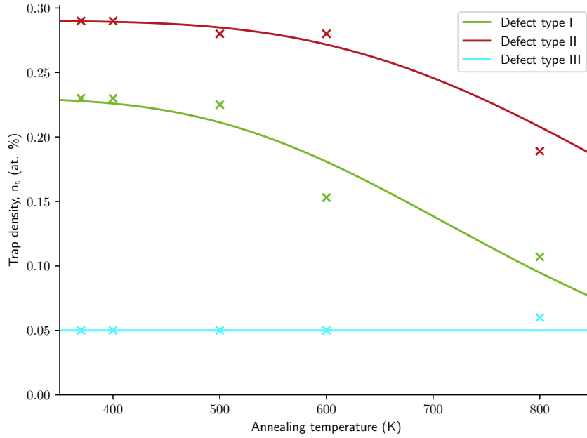
Figure 4.2: Trap densities evolution with annealing temperature fitted using Eq. (4.4). Experimental data points [104]
