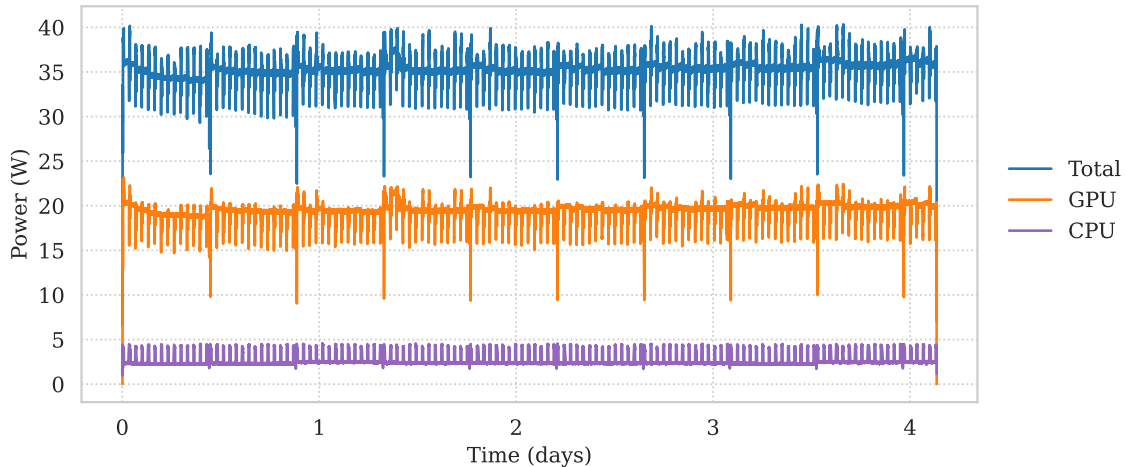
Figure 4.6: The power consumption of ResNet-50* FU on Jetson AGX Xavier.
