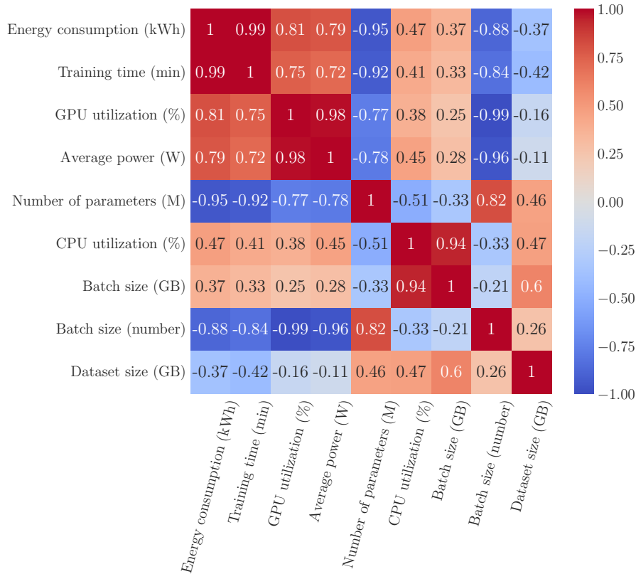
Figure 4.2: Correlation between model characteristics and training performances.
