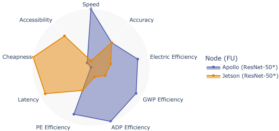
Figure 6.1: Multi-criteria comparison of the ResNet-50* on Jetson and Apollo. For criteria with values outside of the [0,1] interval, values were normalized between 0 and 1, with 1 being the target of the corresponding criteria. Minimum and maximum values are set to (3, 0) , (100, 0) , (0.70, 0) , (0.00013, 0) , (50, 0) for electricity consumption (kWh), duration (hours), GWP (kg CO 2 eq), ADP (kg Sbeq), and PE (MJ), respectively, thus converting them into efficiency metrics.
