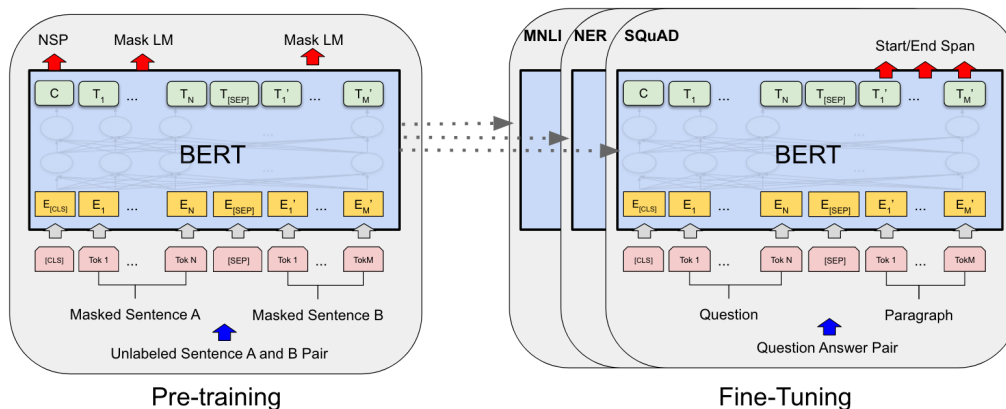
Figure 2.4: Pre-training and fine-tuning procedures for BERT.
