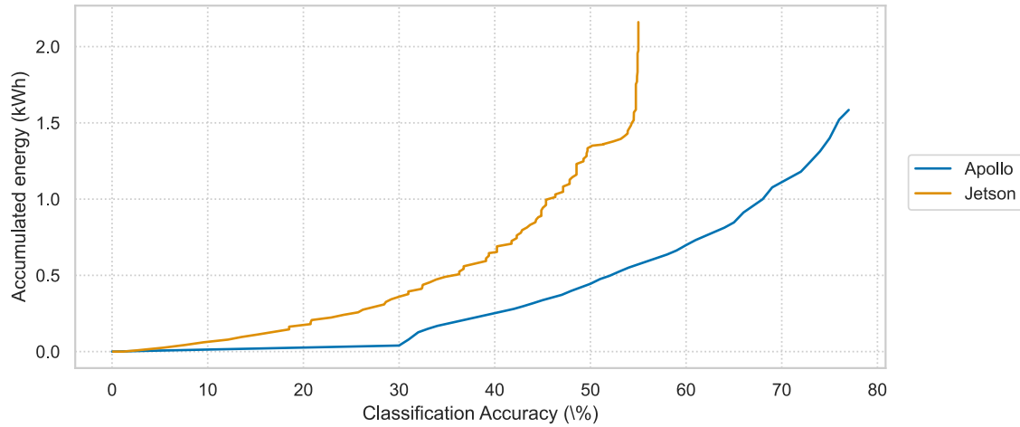
Figure 4.8: Energy required to reach each accuracy point for the Jetson node and the Apollo node while training ResNet-50 on ImageNet.
