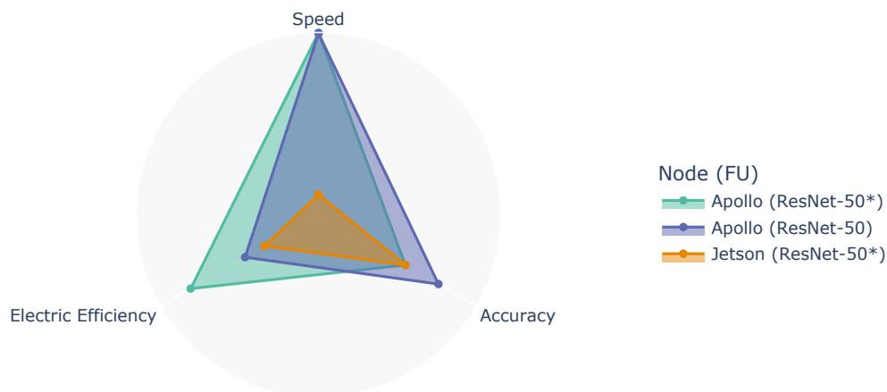
Figure 4.9: Multi-criteria comparison of the ResNet-50 and ResNet-50* FUs on Jetson and Apollo. Values were normalized between 0 and 1, with 1 being the target of the corresponding criteria. For criteria with values outside of the [0,1] interval, values were normalized between 0 and 1, with 1 being the target of the corresponding criteria. Minimum and maximum values are set to (3, 0), (100, 0) for electricity consumption (kWh) and duration (hours), respectively, thus converting them into efficiency metrics.
