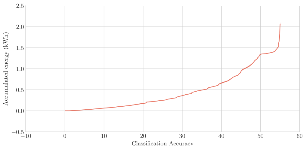
Figure 4.7: Energy required to reach each accuracy point for the Jetson node on the ResNet-50* FU.
