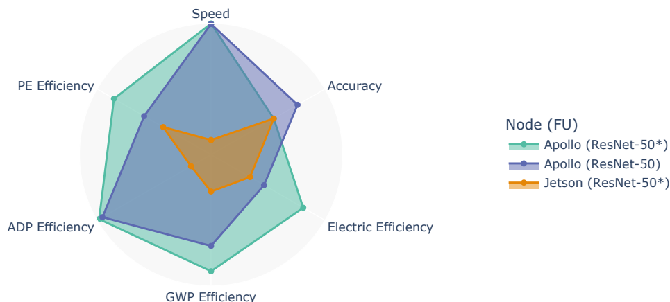
Figure 5.3: Multi-criteria comparison of the ResNet-50 and ResNet-50* FUs on Jetson and Apollo. Values were normalized between 0 and 1, with 1 being the target of the corresponding criteria. For criteria with values outside of the [0,1] interval, values were normalized between 0 and 1, with 1 being the target of the corresponding criteria. Minimum and maximum values are set to (3, 0), (100, 0), (0.70, 0), (0.00013, 0), (50, 0) for electricity consumption (kWh), duration (hours), GWP (kg CO 2 eq), ADP (kg Sbeq), and PE (MJ), respectively, thus converting them into efficiency metrics.
