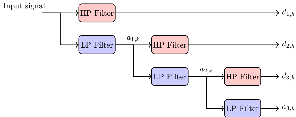
Figure 7.1: General principle of Multiresolution Analysis using LP and HP Filters. The notation a_{j,k} and d_{j,k} denote the coefficients at the j th level of decomposition.
