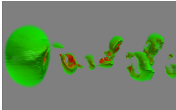
Figure 9.7: D3Q27 LBM simulation at t_{\max} = 600s (24777 iterations) with a 165 \times 680 \times 170 grid ( \approx 1.92GB ) and lossy compression.
