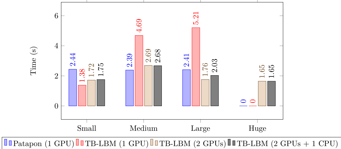
Figure 5.2: Execution times for the different grid sizes ( small , medium , large and huge ) and three hardware setup alternatives. Patapon is a state-of-the-art software that is only able to run on 1 GPU. TB-LBM implements the subgrid mechanism and is able to run on multicore hybrid configurations.
