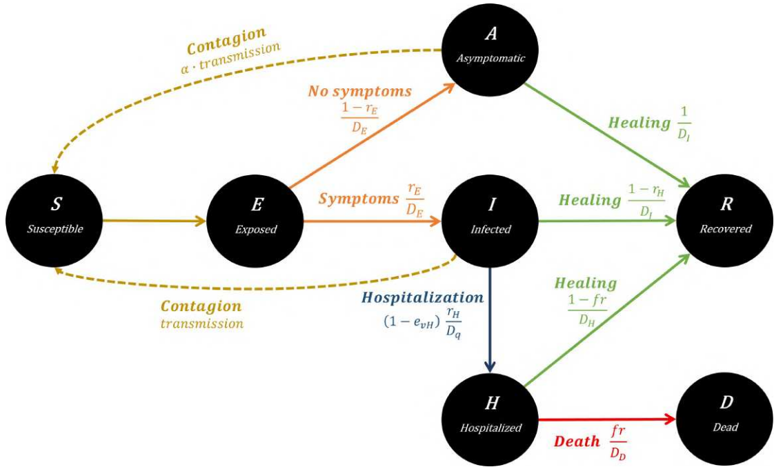
Figure S5.1: Flowchart of SEIRAH model.
