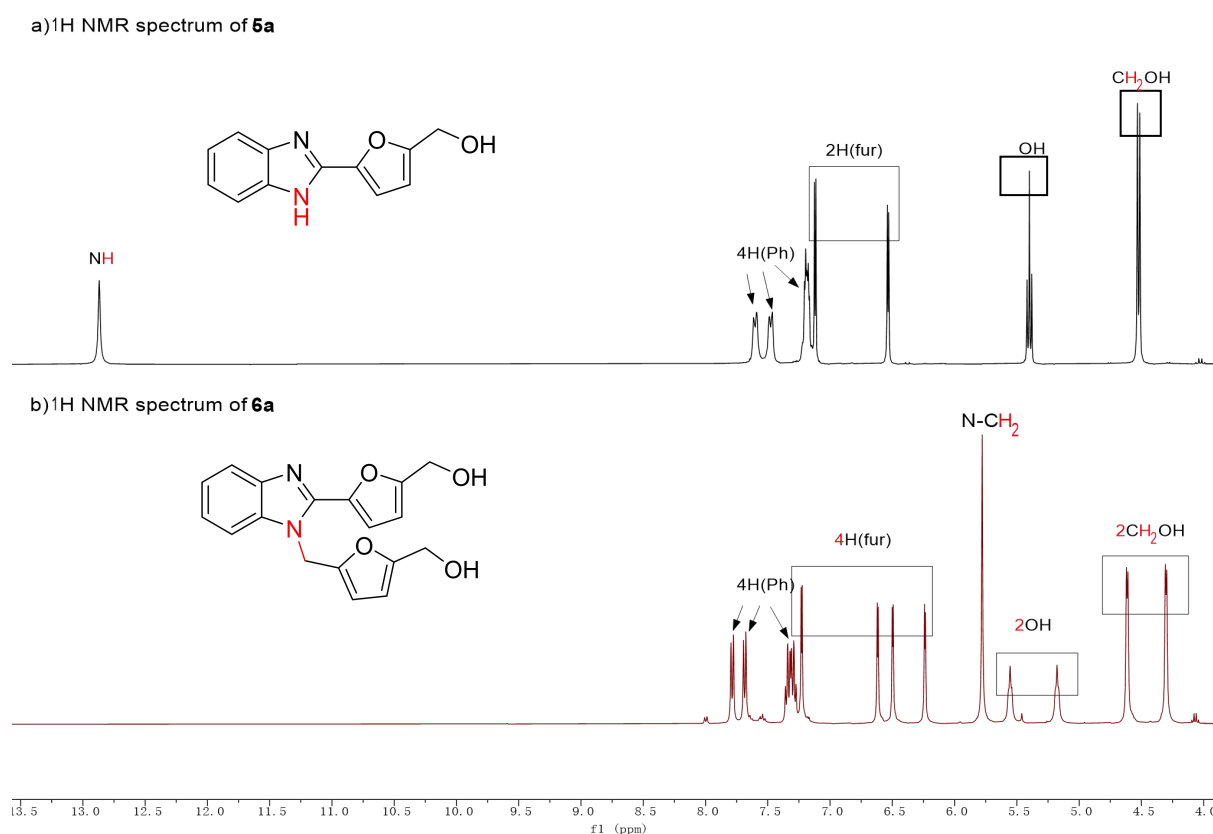
Figure 15. Comparison of ^1\text{H} NMR spectra of by-products 5a and 6a
