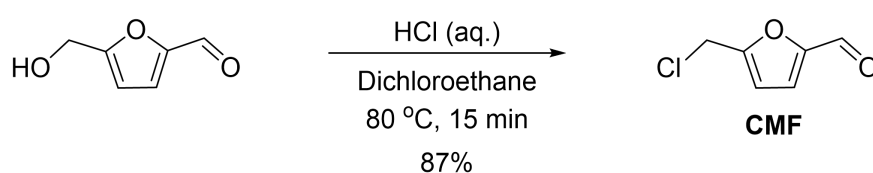
Scheme 28. The formation of 5-halomethylfurfural
