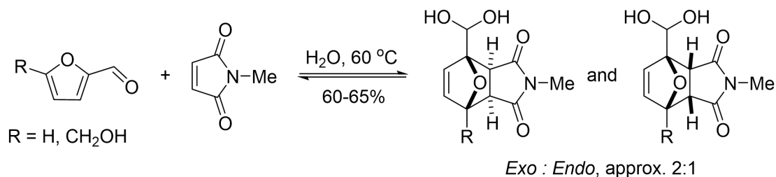
Scheme 41. Novel Diels-Alder adducts from HMF or furfural with N-methyl maleimide
