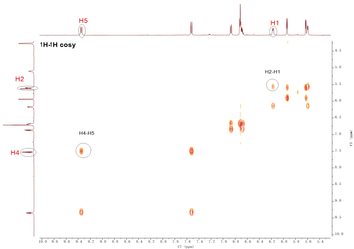
Figure 12. ^1\text{H} - ^1\text{H} COSY NMR spectrum of the 1,5-benzodiazepine 4a
