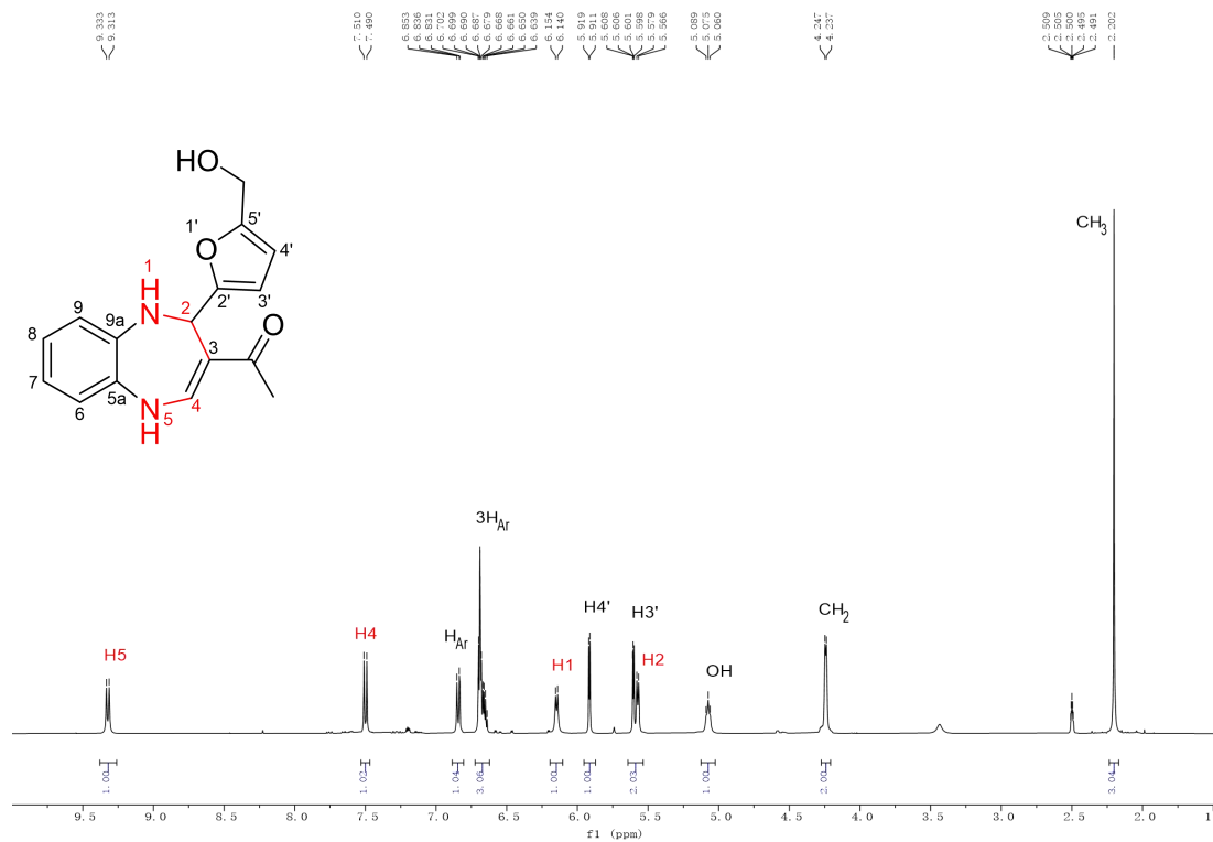
Figure 11. ^1\text{H} NMR spectrum of the 1,5-benzodiazepine 4a
