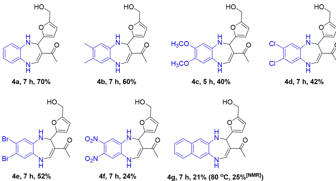
Figure 17. Scope of substituted o -phenylenediamine substrates
