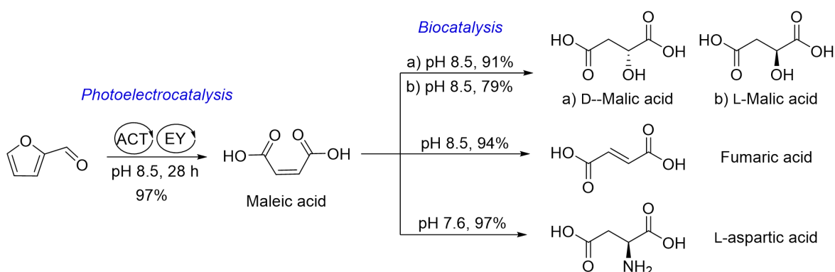
Scheme 19. Electro-, photo-, and biocatalysis for one-pot selective conversion of furfural into C 4 chemicals
