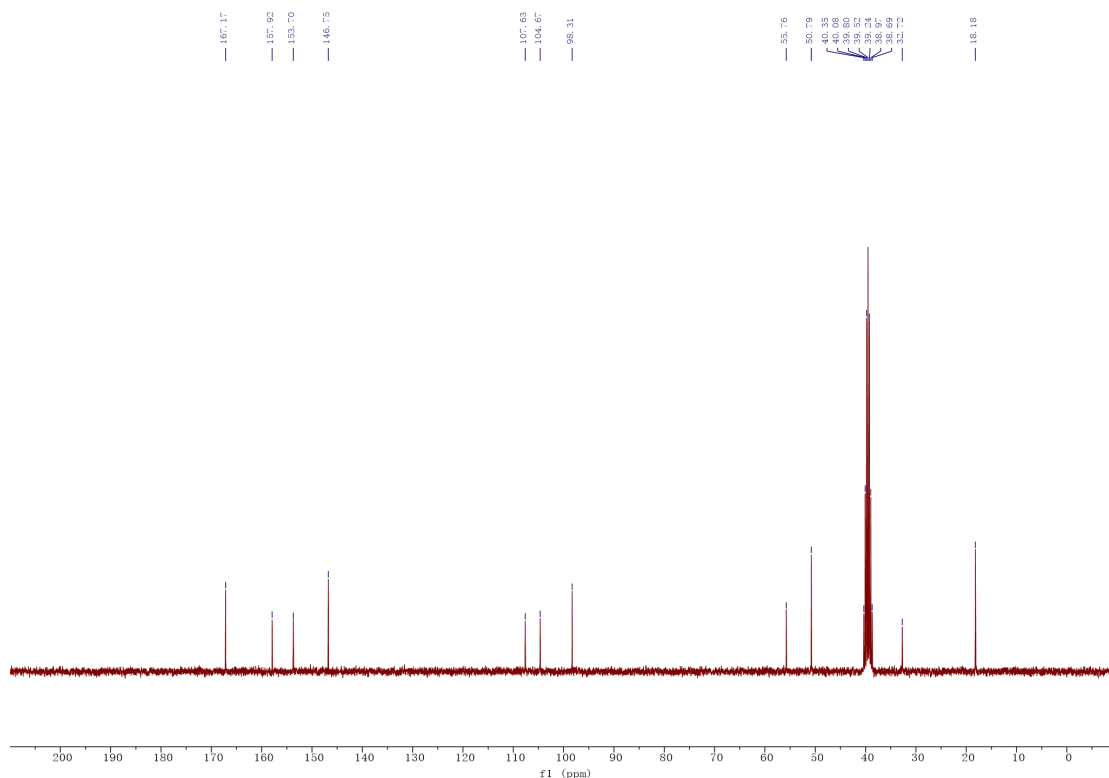
Dibenzyl 4-[5-(hydroxymethyl)furan-2-yl]-2,6-dimethyl-1,4-dihydropyridine-3,5-dicarboxylate (C 28 H 27 NO 6 ) 135
