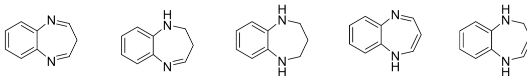
Figure 8. Different forms on the seven-membered ring of 1,5-benzodiazepines
