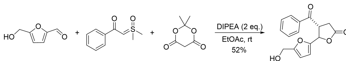
Scheme 63. Synthesis of HMF derived disubstituted \gamma -butyrolactone
