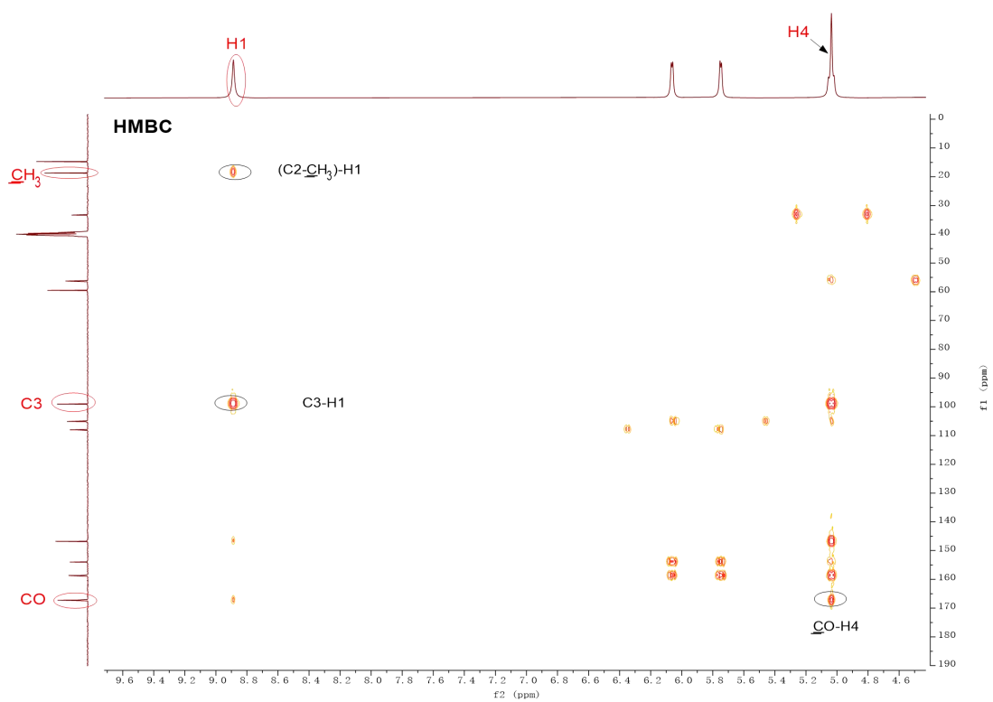
Figure 26. HMBC NMR spectrum of 1,4-dihydropyridine 11a .
