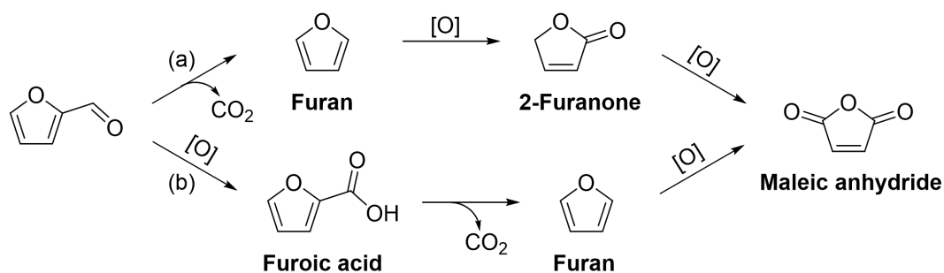
Scheme 18. Proposed VO x /Al 2 O 3 or VPO catalyzed conversion of furfural to maleic anhydride
