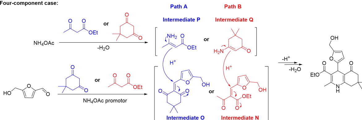
Scheme 94. Formation of the 5-HMF based unsymmetrical 1,4-dihydropyridine
