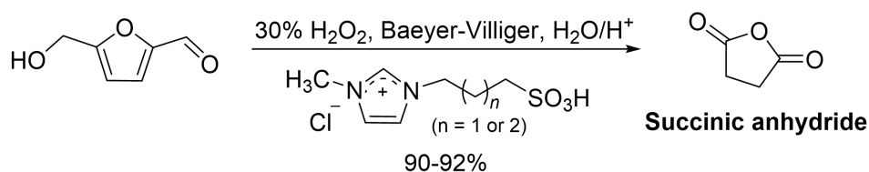
Scheme 38. Conversion of HMF to succinic anhydride
