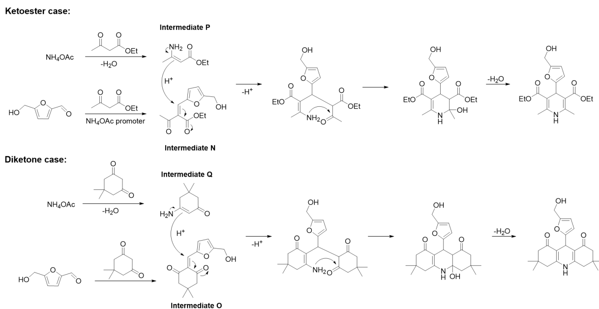
Scheme 93. Formation of the 5-HMF based symmetrical 1,4-dihydropyridines
