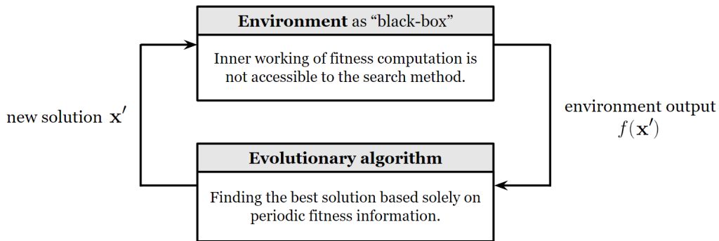
Figure 2.3 – Evolutionary algorithms are derivative-free black-box optimization methods.
