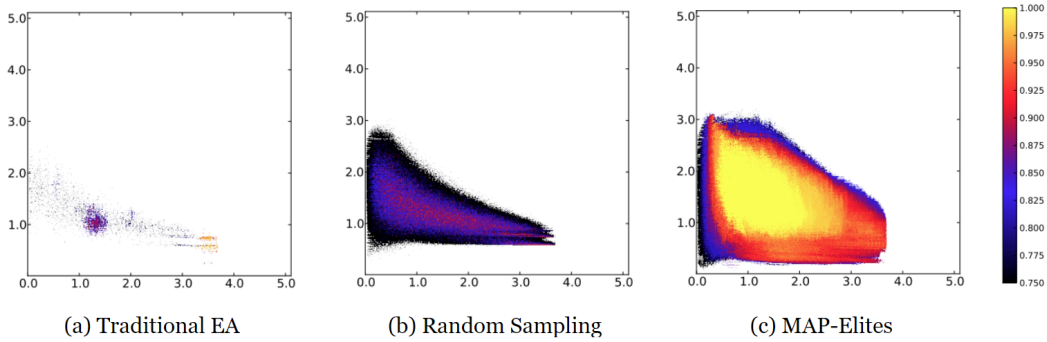
Figure 2.5 – MAP-Elites produces significantly higher-performing and more diverse solutions than control algorithms for the pattern recognition task described in Clune, Mouret, and Lipson (2013). x and y axes represent the arbitrary space of interest to explore, while color indicates performance. Taken from Mouret and Clune (2015).
