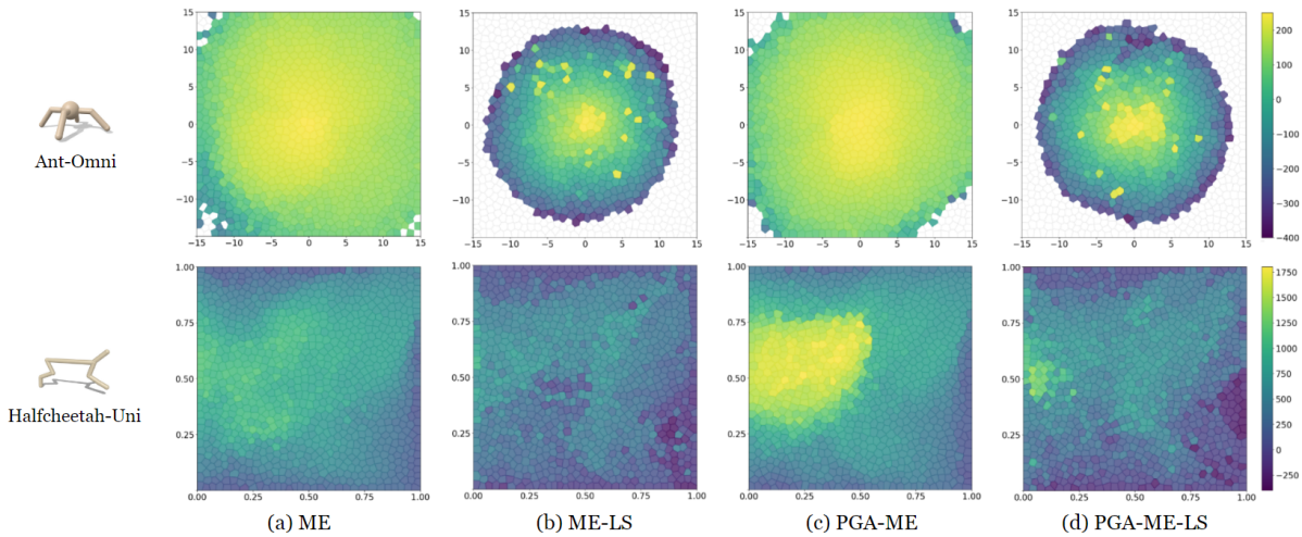
Figure 4.13 – Coverage maps of QD algorithms. Fitness is represented by color; lighter is better.
