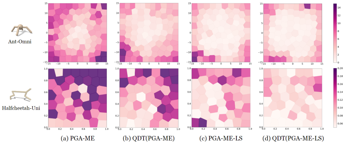
Figure 4.9 – Results of the accuracy experiment for PGA-ME and its variants. The experimental process is strictly identical to that of Figure 4.8. Analogously to results of the MAP-Elites variants in Figure 4.8, QDT(PGA-ME-LS) appears to be the most accurate method to achieve behaviors on demand.
