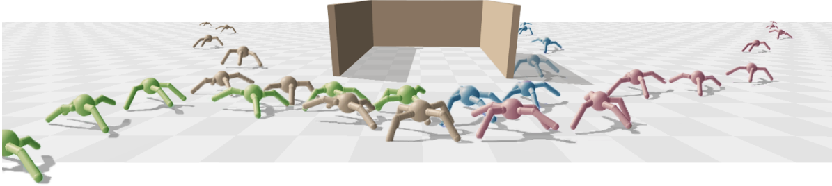
Figure 3.1 – An agent robot is rewarded for running forward as fast as possible. Following the reward signal without further exploration leads into a trap corresponding to a poor local minimum. Our method, QD-PG, produces a collection of solutions that are diverse and high-performing, allowing deeper exploration necessary to solve hard-exploration problems.
