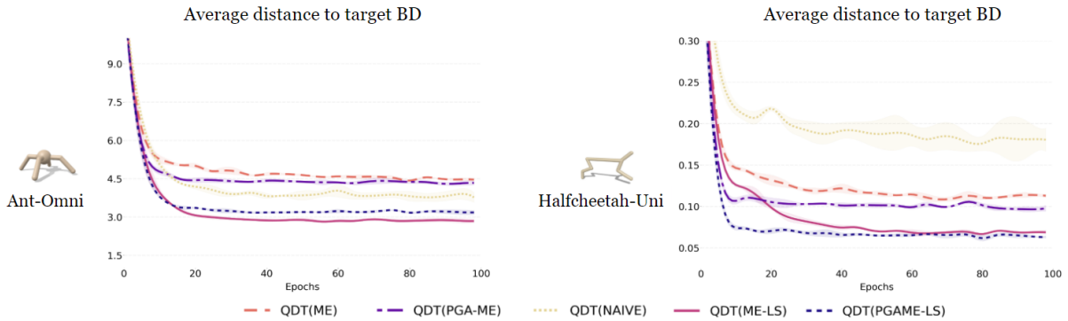
Figure 4.7 – Evaluation results of the QDT through the training process (average values and std ranges on 3 seeds). We evaluate the model over multiple goals (target BDs) covering the behavior space and report the total average Euclidian distance to these goals. The models trained on datasets created by Low-Spread methods, whether using ME-LS or PGA-ME-LS, show significantly better performances.
