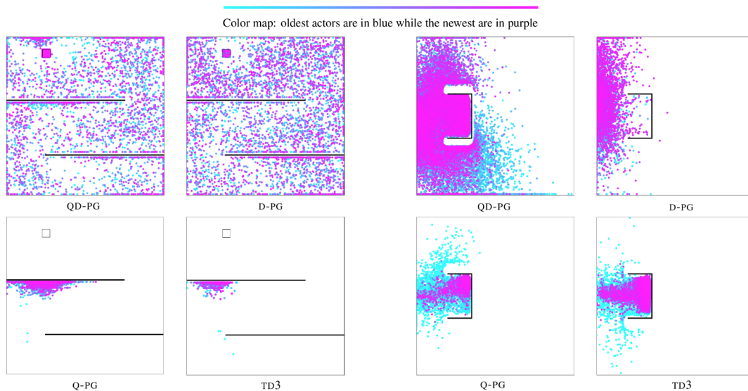
Figure 3.8 – Coverage map of the Point-Maze (left) and Ant-Trap (right) environments for all ablations. Each dot corresponds to the final position of a policy through the training process.
