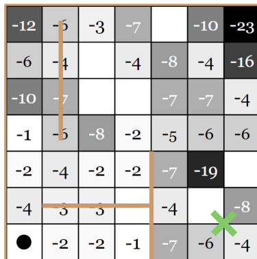
Figure 3.7 – Results of the fast-adaptation experiment repeated 100 times in Ant-Maze. In each square, we display the score of the best experiment whose goal was sampled in this region of the maze, as several experiments may have goals in the same square. Empty squares correspond to regions where no goal was sampled during the experiments. The black circle shows the agent starting position, the black lines represent the walls in Ant-Maze and the green cross marks the location of the original goal in Ant-Maze.
