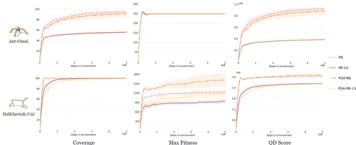
Figure 4.12 – Results of the Quality-Diversity algorithms: MAP-Elites (ME), PGA-MAP-Elites (PGA-ME) and their Low-Spread variations (ME-LS and PGA-ME-LS) in both environments over 5 seeds. Coverage indicates the proportion of the behavior space that have been covered in the repertoire, max fitness reports the best fitness obtained by any solution evaluated so far and the QD score represents the total sum of fitness across all solutions in the repertoire. Performances are plotted against the number of interactions with the environment.
