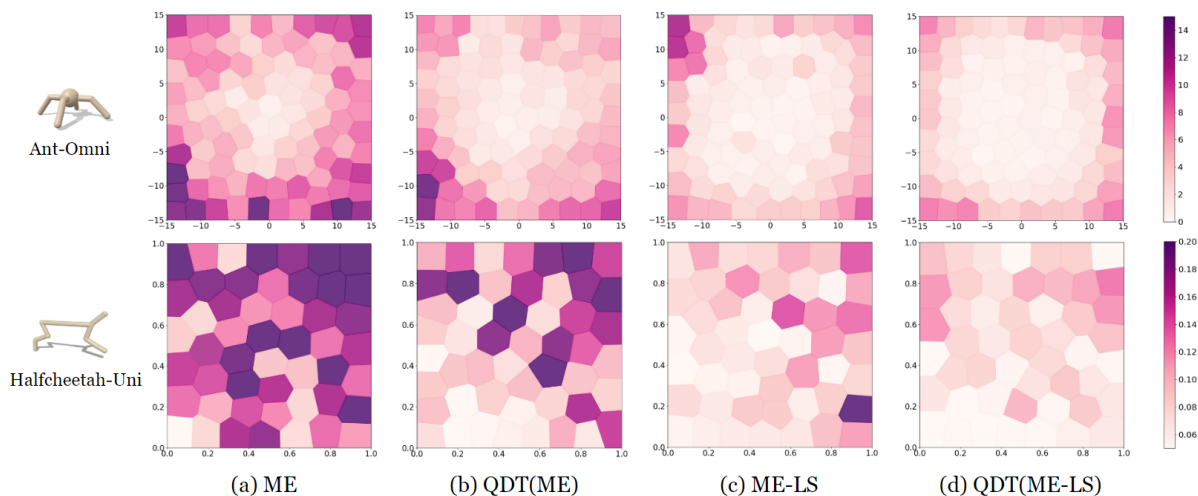
Figure 4.8 – Results of the accuracy experiment. This experiment can be described in 2 steps: 1. We select multiple evaluation goals (target BDs) in the behavior space, 100 and 50 for Ant-Omni and Halfcheetah-Uni respectively. To get meaningful goals, we simply compute a CVT of the BD space in which goals are the centers of each zone, 2. For each goal, we play 10 episodes and plot their average Euclidean distance to the goal. For ME and ME-LS, trajectories are played by the nearest policy to the goal in the repertoire. For the QDT, we simply condition it on the goal. Distance is represented by color: lighter is better. The QDT(ME-LS) appears to be the most accurate method to achieve behaviors on demand.
