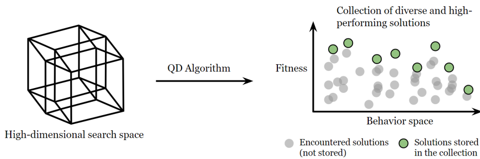
Figure 2.4 – QD algorithms are historically evolutionary algorithms that project a high-dimensional search space (the space of solution genotypes) into a lower-dimensional space capturing the solution behaviors. Here, for the sake of simplicity, the behavior space is unidimensional. Taken from Cully and Demiris (2017).
