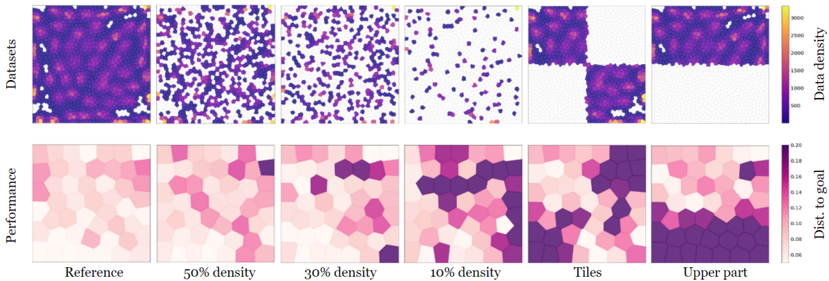
Figure 4.11 – Results of the QDT generalization experiment in Halfcheetah-Uni. The QDT shows strong interpolation ability on the 50%, and 30% density datasets and a limited ability to extrapolate in "Tiles" and "Upper part" datasets where entire zones of the BD space are deprived of data.
