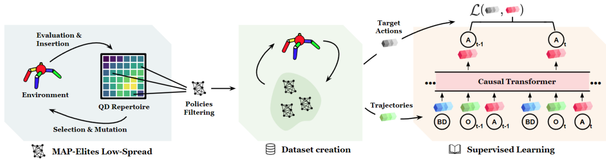
Figure 4.1 – High-level view of the Quality-Diversity Transformer pipeline. Our full algorithm is composed of three distinct and successive parts: 1. Execution of MAP-Elites Low-Spread, our variation of MAP-Elites that produces stable and consistent policies, 2. Creation of an offline dataset of trajectories by playing episodes with some of the policies produced by MAP-Elites Low-Spread, 3. Supervised training of a behavior-conditioned causal Transformer producing on-demand behaviors with high accuracy.
