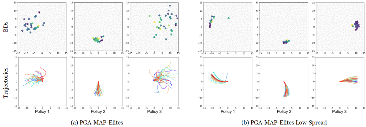
Figure 4.4 – Reproducibility problem in Ant-Omni. Here we reproduce the experiment proposed in Figure 4.3 for a) PGA-MAP-Elites and b) PGA-MAP-Elites Low-Spread.
