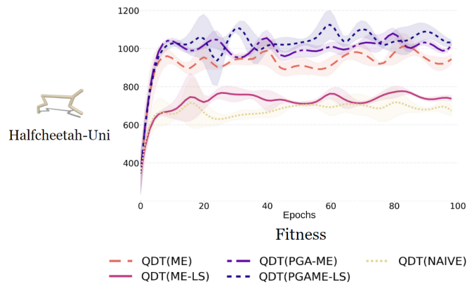
Figure 4.14 – Maximum fitness of the QDT in Halfcheetah-Uni for evaluations during the training phase (average values and std ranges on 3 seeds). We report the maximum fitness obtained over all goals. Performances are similar, if not superior, to values reported in the reassessment experiment in Table 4.5, meaning our model is able to replicate the fitness of QD policies.
