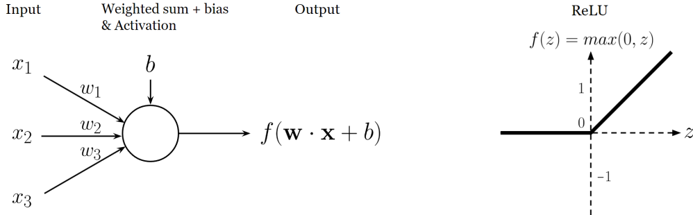
Figure 2.1 – Left: A single MLP node computes its output as a weighted sum of the input (plus a bias that acts as an additional parameter) and passes the result through a nonlinear activation function. Right: Example of a nonlinear activation function, the rectified linear unit (ReLU).
