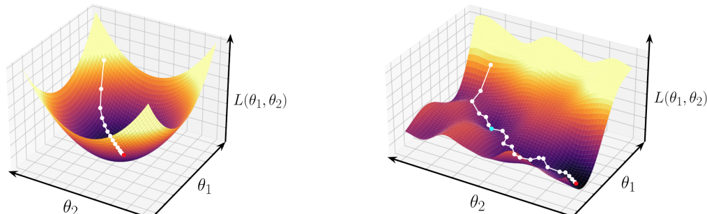
Figure 2.2 – A simple case of gradient descent with only two parameters: \theta_1 and \theta_2 , in the case of a perfectly convex loss function (left); a non-convex loss function (right) with a local minimum (blue dot).
