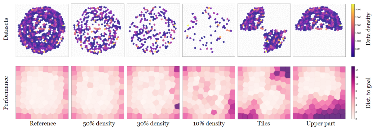
Figure 4.10 – Results of the QDT generalization experiment in Ant-Omni. In this experiment we run accuracy experiments (bottom row) on truncated datasets (top row) which are deprived of a part of their trajectories. The QDT shows strong interpolation ability on the 50%, 30% and 10% density datasets and a more limited ability to extrapolate in "Tiles" and "Upper part" datasets where entire zones of the BD space are deprived of data.
