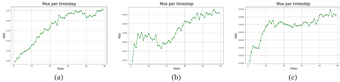
Figure 5.5 – Mean square error per timestep for all three examples (a), (b) and (c) presented in Figure 5.3, respectively.
