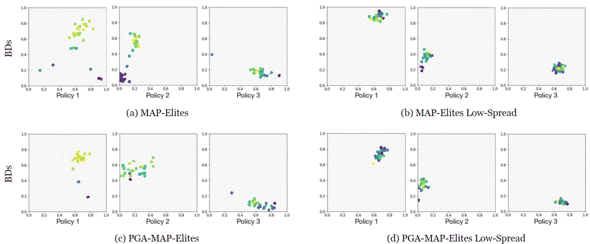
Figure 4.5 – Reproducibility problem in Halfcheetah-Uni for a) MAP-Elites, b) MAP-Elites Low-Spread, c) PGA-MAP-Elites, d) PGA-MAP-Elites Low-Spread.
