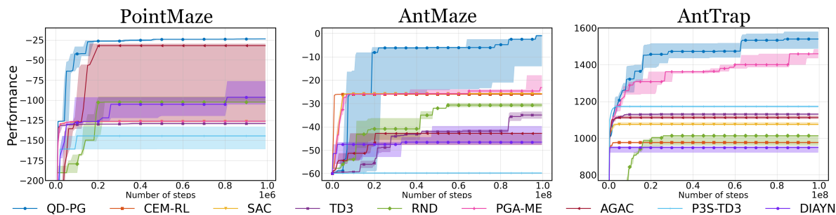
Figure 3.5 – Performance of QD-PG and baseline algorithms on all environments. Plots present median bounded by first and third quartiles.
