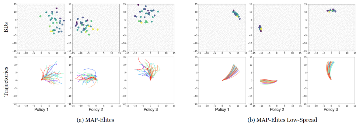
Figure 4.3 – Reproducibility problem in Ant-Omni. We select three representative policies from final repertoires that have been generated by a) MAP-Elites and b) MAP-Elites Low-Spread, our proposed variant, and play 30 episodes with each policy using slightly varying initial states. The top row depicts the final BDs obtained by each policy and the bottom row represents the corresponding entire trajectories in the behavior space. Each color represents a different random seed (initial condition).
