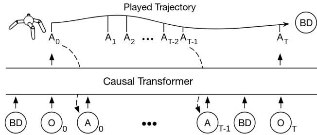
Figure 4.6 – The QDT autoregressively plays an evaluation episode by conditioning on a target BD. At any given timestep t , the QDT generates an action by looking at all elements of the trajectory that precede t . The first action A_0 is generated given the target BD and the first observation O_0 , while the last action A_T is generated given the whole trajectory of target BDs, observations and previously generated actions. Note that the target BD is the same for the entire trajectory.
