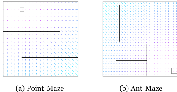
Figure 3.4 – Gradient maps on Point-Maze and Ant-Maze. Black lines are maze walls, arrows depict gradient fields and the square indicates the maze exit. Both settings present deceptive gradients as naively following them leads into a wall.
