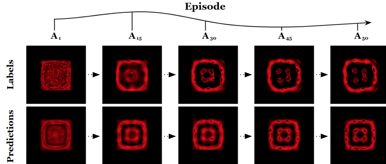
Figure 5.4 – Chronology of labels and predictions over the entire episode from Figure 5.3a. Prediction frames are denoised manually to better show the central pattern.
