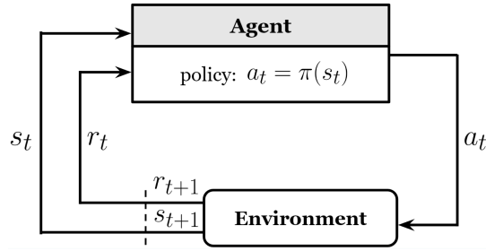
Figure 2.6 – The RL agent-environment interaction loop in a Markov decision process, taken from Sutton and Barto (2018). The environment provides states and rewards, and the agent policy chooses actions.
