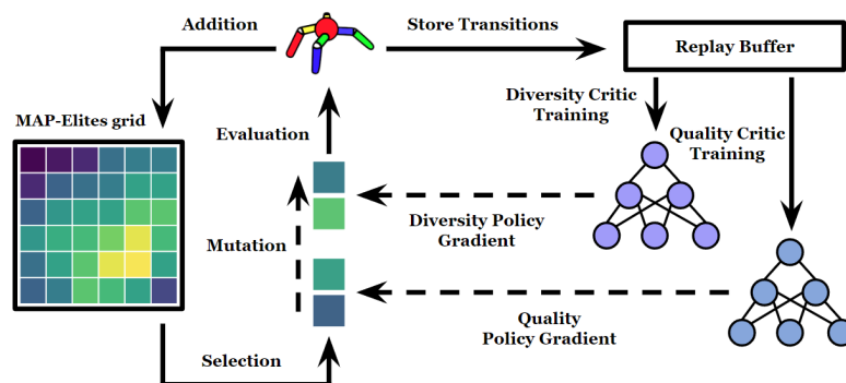
Figure 3.2 – QD-PG builds on the MAP-Elites framework and leverages reinforcement learning to derive policy gradient based mutations.
