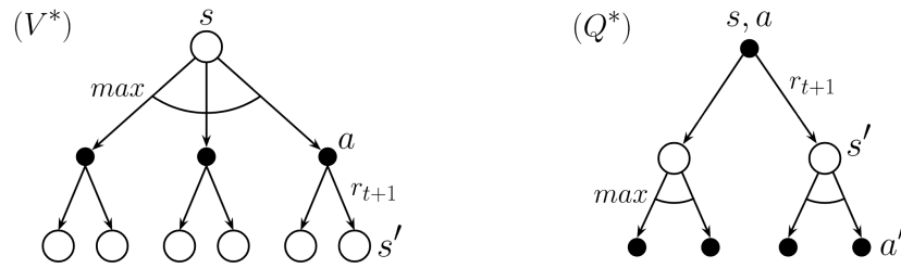
Figure 2.7 – Backup diagrams for the Bellman optimality equations for V^*(s) and Q^*(s, a) . Backup diagrams provide intuitive interpretations of Bellman equations, where states are represented as large empty circles and state-actions pairs as smaller black dots. Arrows denote the possible scenarios following either a state or a state-action pair.
