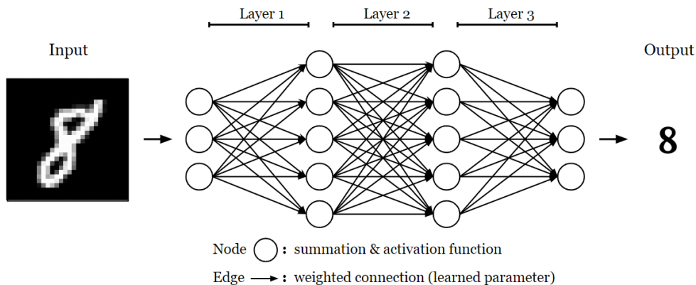
Figure 1.1 – High-level view of a trained multilayer perceptron neural network. An input image representing the hand-written digit "8" is fed to a trained neural network, which is able to identify it correctly.
