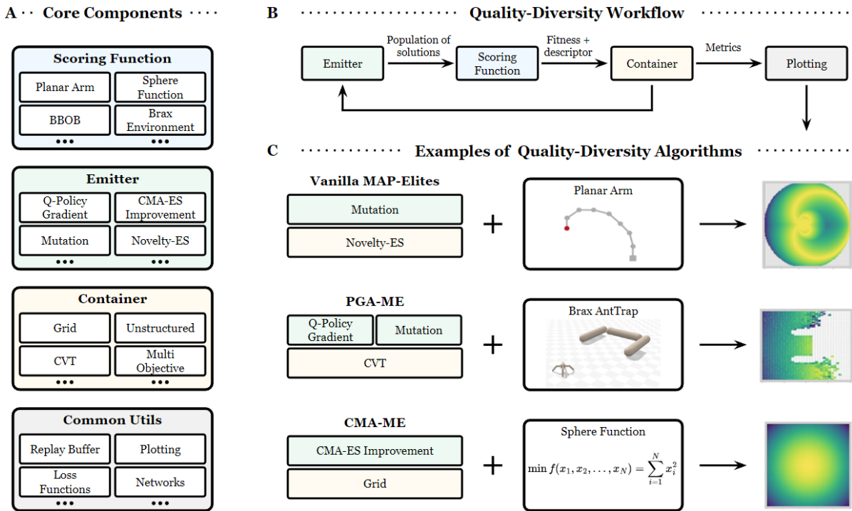
Figure 2.8 – A) Core components, used as building blocks to create optimization experiments. B) High-level software architecture of QDax. C) Various examples of QD algorithms used for a variety of tasks and problem settings available in QDax. Taken from Chalumeau, Lim, Boige, et al. (2024).
