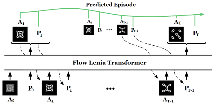
Figure 5.2 – Evaluation process of the FLT. The model autoregressively produces an entire episode based on an initial state made of initial activations A^0 and initial parameters map P^0 .
