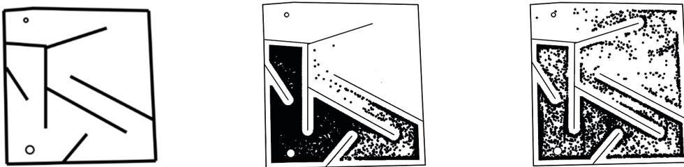
Figure 1.4 – A canonical hard-exploration problem. From left to right: 1. Picture of the maze where the agent (larger circle) is rewarded the closer it gets to the exit (smaller circle), 2. Results of using a classical evolutionary algorithm to solve the problem, most tries (black dots) end up in dead ends, 3. Results of running an exploration-oriented algorithm, which solves the maze by focusing on exploration and novelty search. Taken from Lehman and Stanley (2011a).
