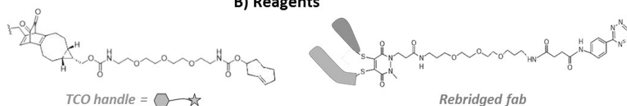
Figure 54: Schematic representation of the development of bispecific antibodies (bsAb) through bio-orthogonal tyrosine-based click chemistry. (A) BsAb formation reaction resumed in three steps: 1. deglycosylation of intact mAb using peptide-N-glycosidase F (PNGase F), 2. Functionalization of the Fc part with trans-cyclooctene (TCO) handles using mushroom tyrosine (mTyr) and 3. The attachment of the TCO-functionalized mAb to Fab fragments, prior rebridged using pyridazinediones (PD). Fab fragments used are either from trastuzumab or OKT3 antibodies. The theoretical masses of the used TCO and Fab fragments, along with the theoretical masses of the final products are represented on the scheme. (B) Structures of the reagents used for bsAb formation namely TCO and rebridged Fab fragments.
