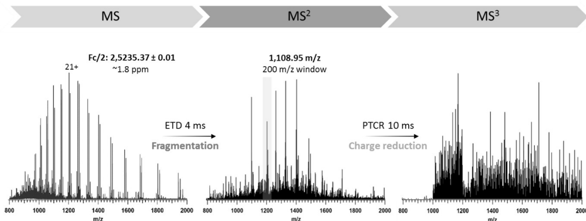
Figure 93: PTCR reaction after ETD fragmentation of the Fc/2 subunit. The Fc/2 is first analyzed at the MS level for accurate mass measurement, then the selected precursor ion (21+ in this case) is subjected to ETD fragmentations in the optimized conditions (4 ms here). A product ion (1108.95 m/z ) is selected using a window of 200 m/z and subjected to PTCR ion-ion reaction for charge reduction to identify more overlapping species in the selected window.
