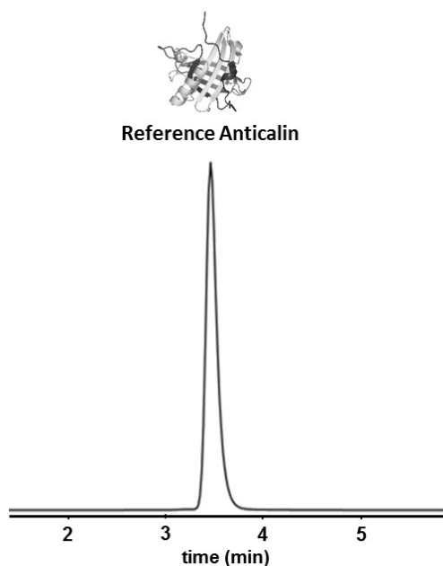
Figure 51: SEC-nMS analysis of reference Anticalin D11vs variant. (A) SEC-UV signal showing one homogeneous species at 3.45 min (B) Native MS spectra of the identified peak, showing three different regions namely denatured form of Anticalin, monomer and dimer forms. On the grey square, a zoom on the charge state 10+ of the monomer region showing the triplet profile of the peaks due to presence of modifications on the protein.
