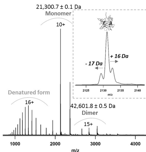
Figure 51: SEC-nMS analysis of reference Anticalin D11vs variant. (A) SEC-UV signal showing one homogeneous species at 3.45 min (B) Native MS spectra of the identified peak, showing three different regions namely denatured form of Anticalin, monomer and dimer forms. On the grey square, a zoom on the charge state 10+ of the monomer region showing the triplet profile of the peaks due to presence of modifications on the protein.
