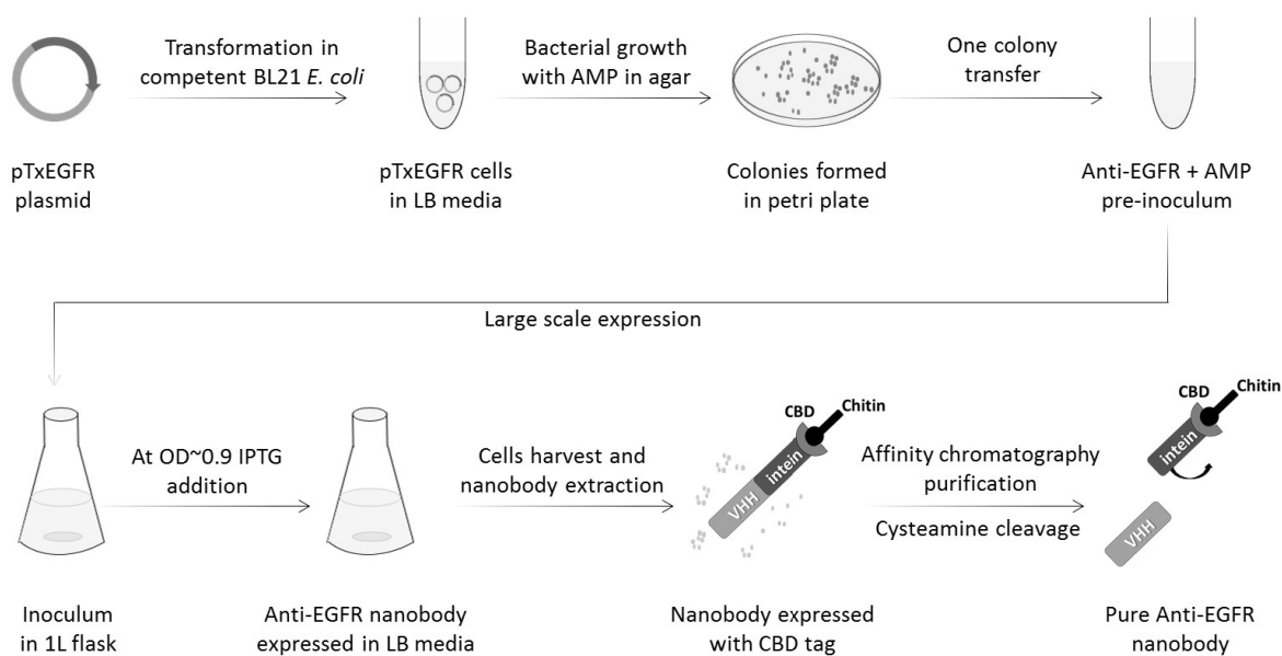
Figure 103: Bacterial expression anti-EGFR nanobody. The competent BL21 E. coli cells are transformed with the pTxEGFR plasmid containing the gene of the anti-EGFR nanobody, and are streaked on AMP agar plates for cells formation. A single colony was transferred to prepare a pre-inoculum that was then transferred to 1L flasks for large scale expression in LB media. At OD~0.9 the IPTG is added to the inoculum to induce protein expression. Protein expression resulted in a nanobody-intein-CBD complex that was purified with intein-CBD affinity chromatography with cysteamine cleavage to release the nanobody.
