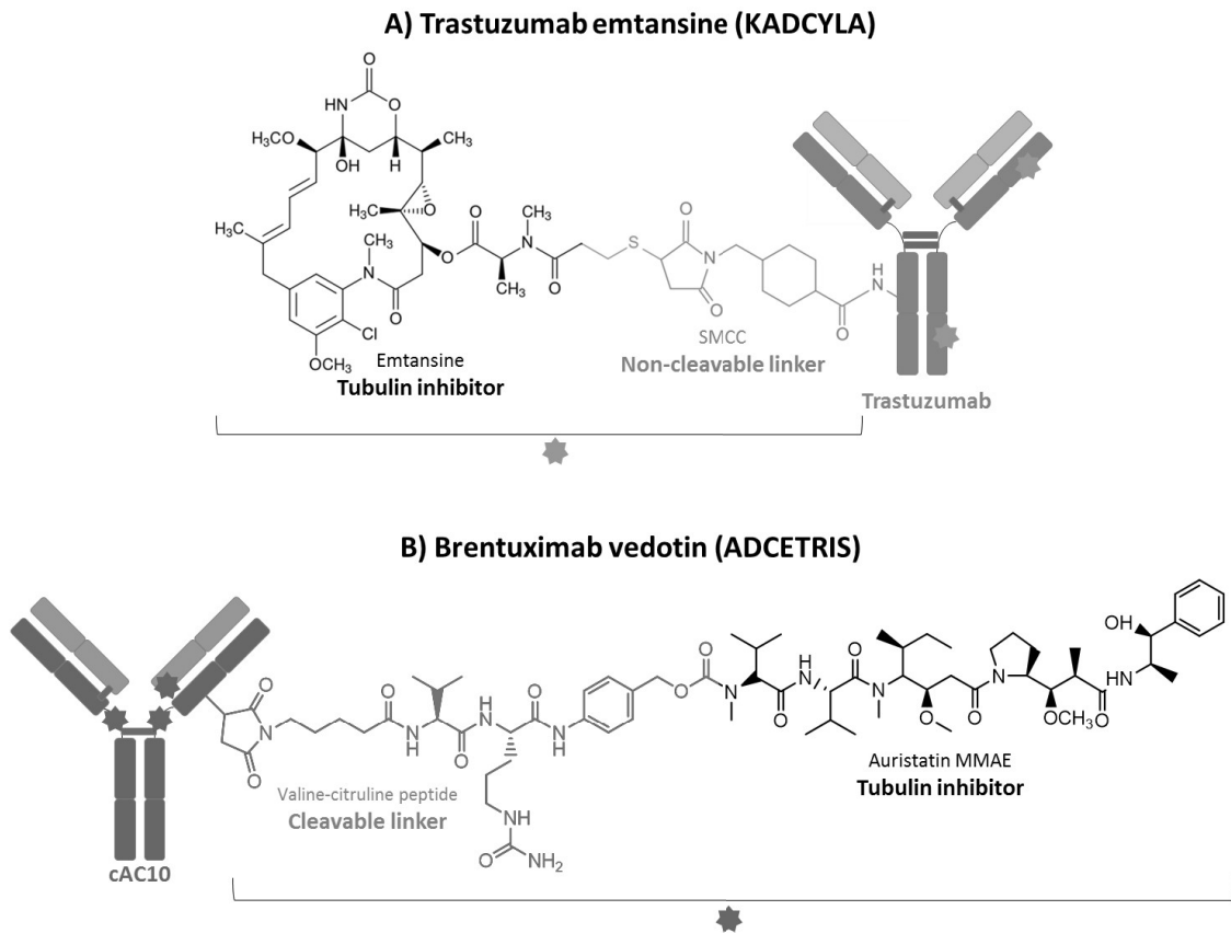
Figure 8: ADCs structure depicted with the example of trastuzumab emtansine (Kadcyla), a conjugated trastuzumab to a emtansine tubulin inhibitor through a non-cleavable linker (SMCC), and Brentuximab vedotin (ADCETRIS) which is a cAC10 mAb conjugated to an auristatin MMAE tubulin inhibitor through a cleavable linker (valine-citrulline peptide). Adapted from Beck et al. (2019) 10
