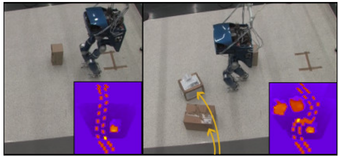
Figure 2.6: An experiment of vision-based footstep planning with the DLR-Biped (boxes are thrown in front of it while it walks, and the robot is able to reactively replan a path to the goal).
