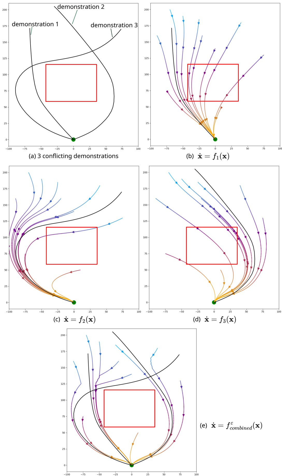
Figure 3.6: Single vector fields combined into \dot{\mathbf{x}} = f_{combined}^\epsilon(\mathbf{x}) , with \epsilon = 10 .
