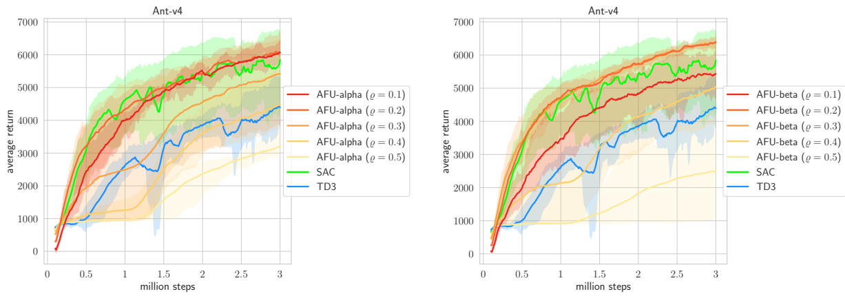
Figure 5.7: Ant-v4. Left: AFU-alpha. Right: AFU-beta.
