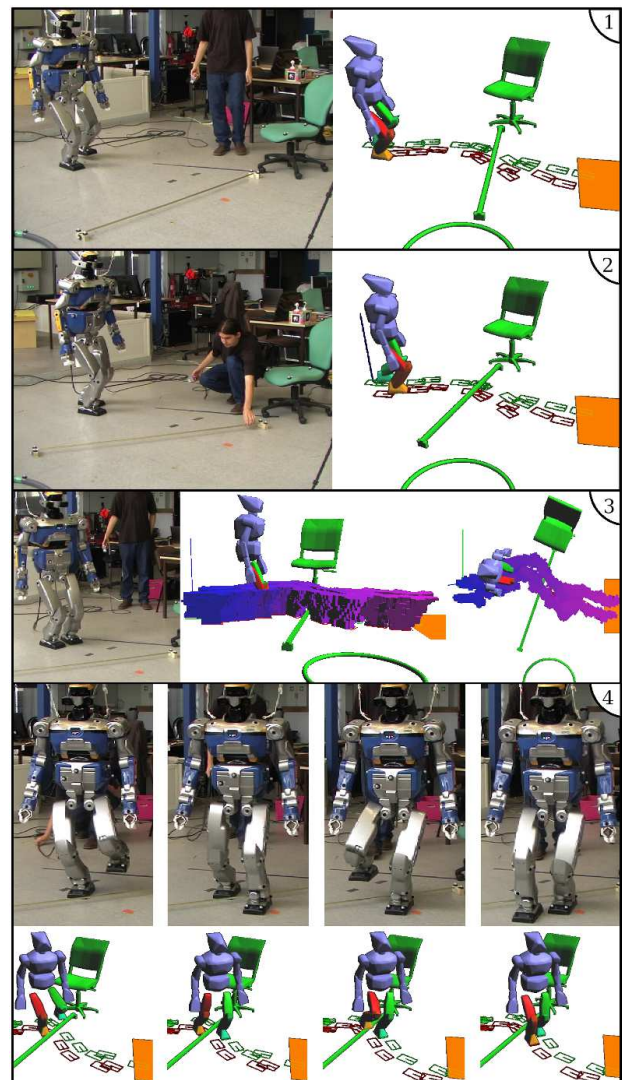
Figure 1.1: Experiment from [Perrin et al. 2012a]. (1): HRP-2 starts to execute the sequence initially found via footstep planning. (2): the bar is suddenly moved, and the current sequence of steps would lead to collisions. (3): while walking, a new sequence of steps toward the goal is computed in real-time. A concatenation of the swept volume approximations is used to ensure the avoidance of contacts with the bar. (4): the robot steps over the bar while optimizing the rest of the path toward the goal.
