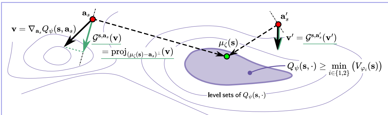
Figure 5.5: The gradient \mathbf{v} at \mathbf{a}_s (on the left) points away from \mu_\zeta(s) , which determines the direction toward the vicinity of the argmax of Q_\psi(s, \cdot) , so we modify \mathbf{v} to get \mathcal{G}^{s, \mathbf{a}_s}(\mathbf{v}) by projecting it on the hyperplane orthogonal to \mu_\zeta(s) - \mathbf{a}_s . The gradient \mathbf{v}' at \mathbf{a}'_s (on the right) points in the direction (half-space) of \mu_\zeta(s) , so we do not modify it, and \mathcal{G}^{s, \mathbf{a}'_s}(\mathbf{v}') = \mathbf{v}' .
