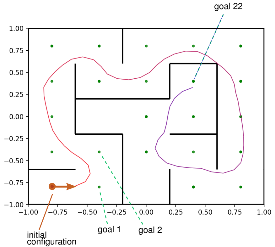
Figure 4.2: A Dubins car is trained to follow a sequence of 22 goals with Budget-based Switching (Algorithm 2). The off-policy RL for the goal-conditioned policy relies on a combination of Soft Actor-Critic (SAC) and Hindsight Experience Replay (HER). After 109k gradient and environment steps, the policy is able to reach the last goal.
