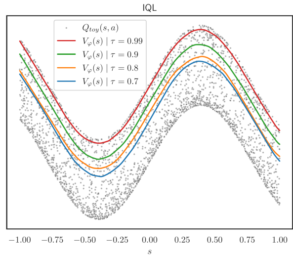
(b) Results of the training with the loss from IQL [Kostrikov et al. 2022] for 4 different values of the hyperparameter \tau . Values used in actual (offline) RL experiments are not greater than 0.9.
