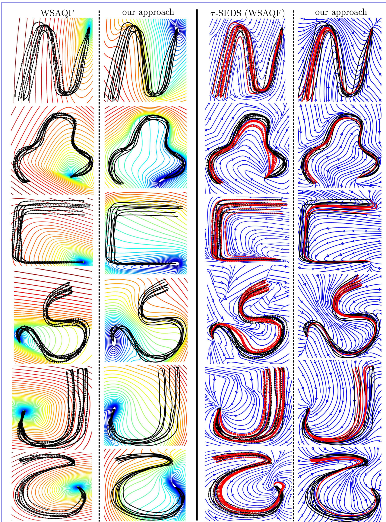
Figure 3.4: Demonstrations are in black, and reproduced trajectories in red. On the left: level sets of the Lyapunov candidates obtained with WSAQF (1st column) and with our approach (2nd column). On the right: streamlines of the DS produced by \tau -SEDS (WSAQF) [Neumann & Steil 2015] (3rd column) and with our approach (4th column).
