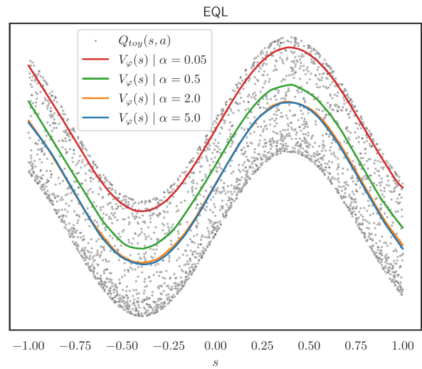
(d) Results of the training with the loss from EQL [Xu et al. 2023] for 4 different values of the hyperparameter \alpha . Values used in actual (offline) RL experiments are not smaller than 0.5..
