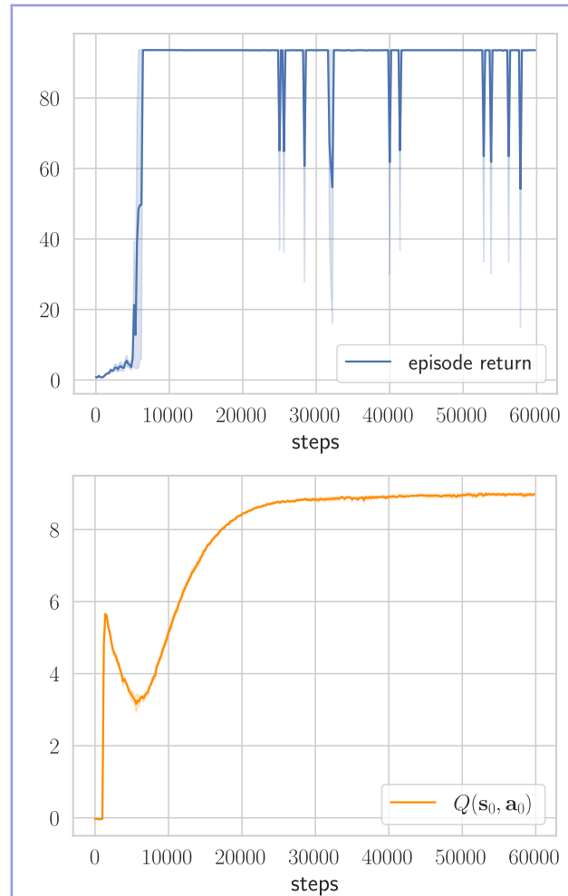
Figure 4.1: Training of Soft Actor-Critic (SAC) on InvertedDoublePendulum-v4 . Results show the interquartile mean (see [Agarwal et al. 2021]) from experiments on 10 different random seeds. The orange curve (bottom) displays the Q -value of the first state and action of evaluation episodes. In fewer than 7,000 steps, the trained policy is near-optimal, yet after 30,000 steps, the Q -values are still slowly increasing.
