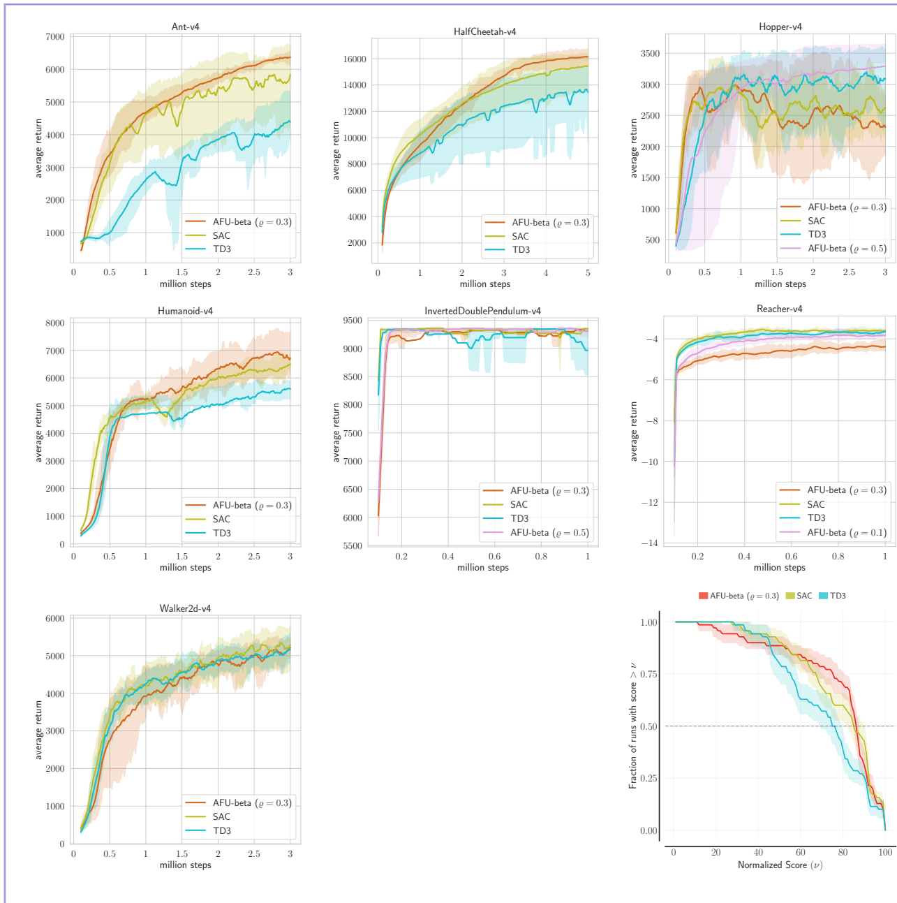
Figure 5.6: Experimental evaluation of AFU-beta for \rho = 0.3 on 7 MuJoCo tasks. We show results with other values of \rho (among \{0.1, 0.2, 0.4, 0.5\} ) for tasks in which one of the other values performed significantly better than 0.3. Results are averaged over 10 runs with different random seeds, and the shaded areas range from the 25th to the 75th percentile. The performance profile plot at the bottom right summarizes results and shows that AFU-beta is competitive with SAC and TD3.
