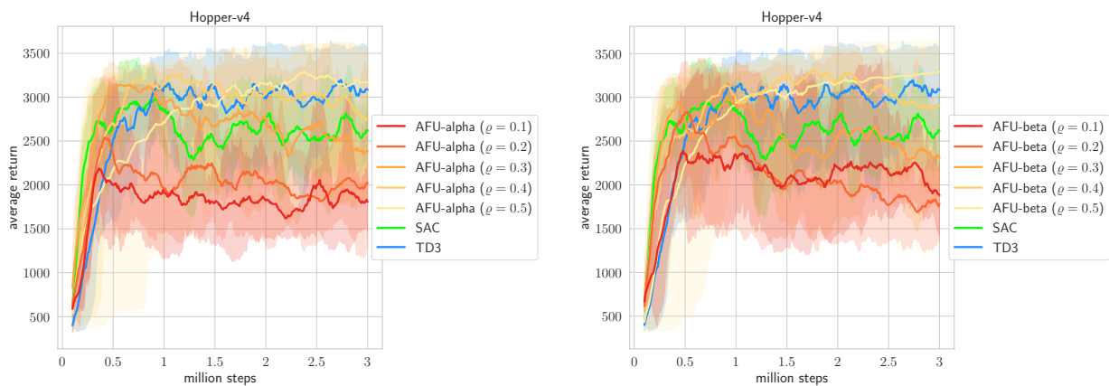
Figure 5.9: Hopper-v4. Left: AFU-alpha. Right: AFU-beta.
