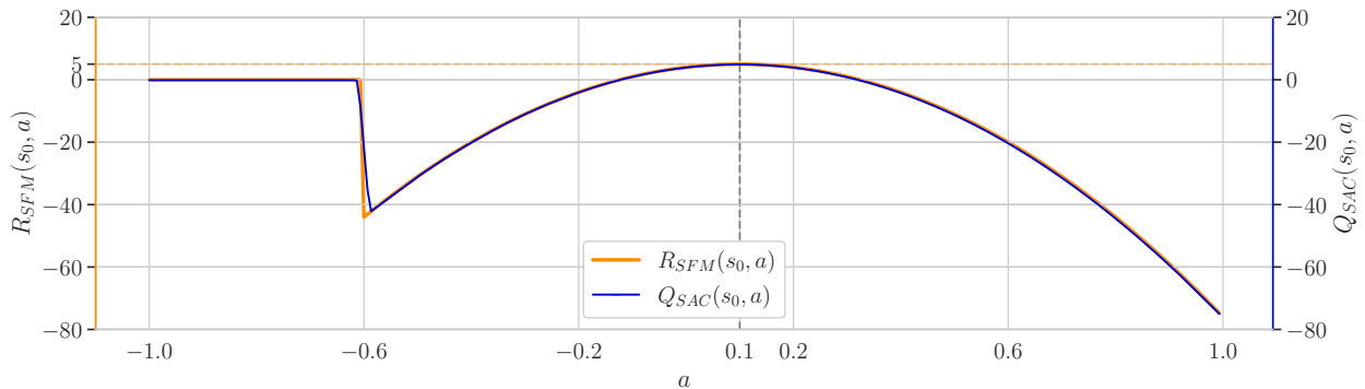
Figure 5.3: In orange: the reward function R_{SFM} of the SFM environment. Since all transitions are terminal, R_{SFM} coincides with the optimal Q-function. In blue: the critic ( Q_{SAC} ) obtained after a training of 20,000 steps with SAC [Haarnoja et al. 2018].
