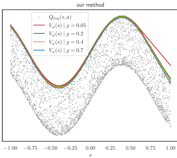
(a) V_\varphi(s) is trained jointly with A_\xi(s, a) by iterating gradient descent steps on the loss \Lambda'_{V, A}(\varphi, \xi) described by Equation (5.5). \varrho \in [0.2, 0.7] results in precise approximations of s \mapsto \max_{a \in A}(Q_\psi(s, a)) .
