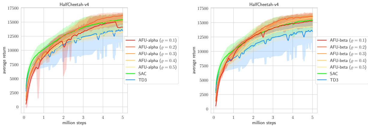
Figure 5.8: HalfCheetah-v4. Left: AFU-alpha. Right: AFU-beta.
