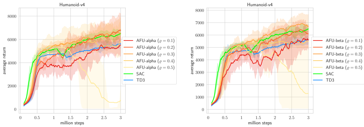
Figure 5.10: Humanoid-v4. Left: AFU-alpha. Right: AFU-beta.
