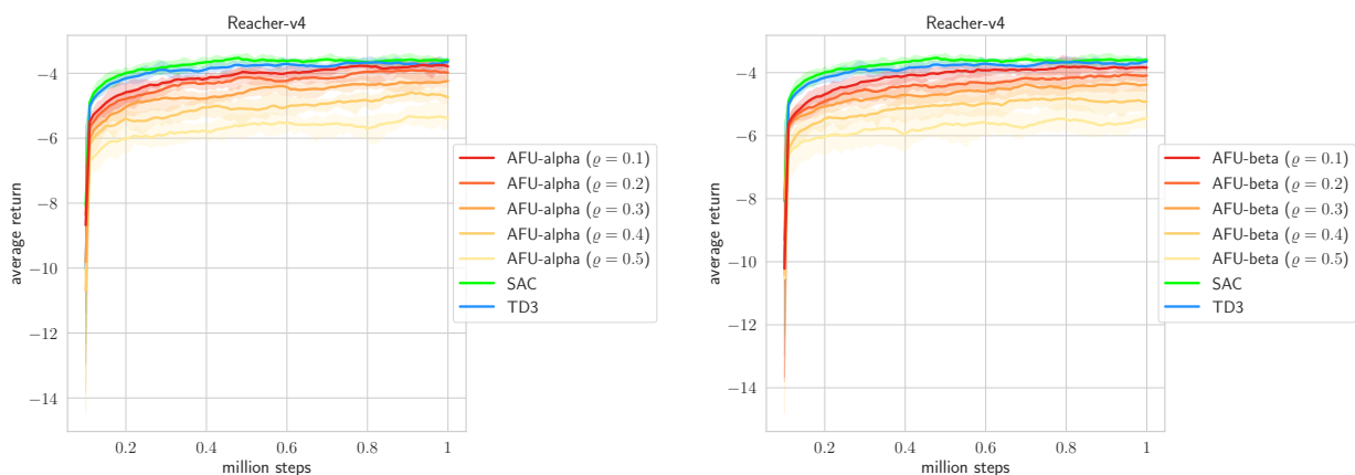
Figure 5.12: Reacher-v4. Left: AFU-alpha. Right: AFU-beta.
