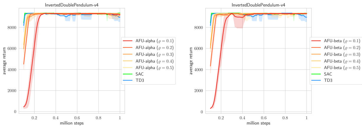
Figure 5.11: InvertedDoublePendulum-v4. Left: AFU-alpha. Right: AFU-beta.
