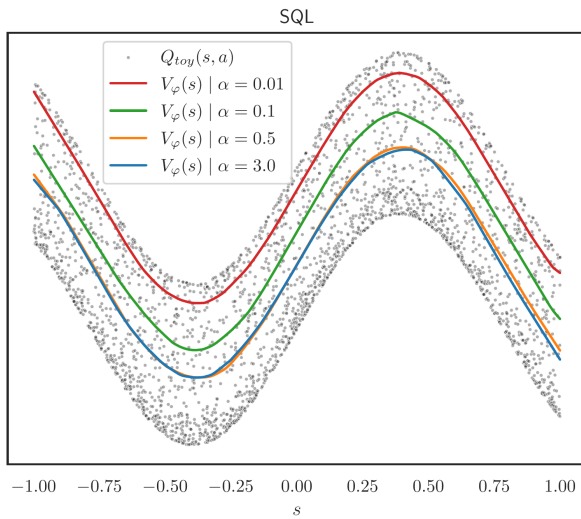
(c) Results of the training with the loss from SQL [Xu et al. 2023] for 4 different values of the hyperparameter \alpha . Values used in actual (offline) RL experiments are not smaller than 0.1.
