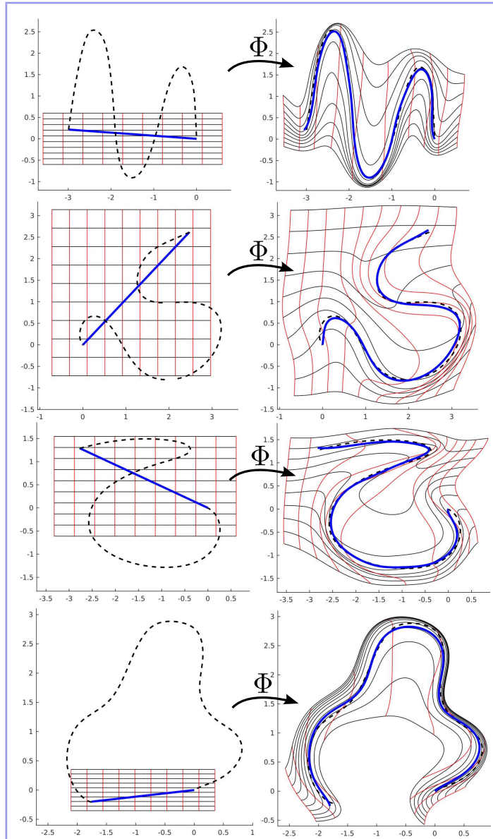
Figure 3.2: On the left, the dashed curve is a trajectory represented by a sequence of points \mathbf{Y} = (\mathbf{y}_i)_{i \in \{0, \dots, N\}} . The solid line is \mathbf{X} = (\mathbf{y}_0 + \frac{i}{N}(\mathbf{y}_N - \mathbf{y}_0))_{i \in \{0, \dots, N\}} . The right side shows the result of the application of the diffeomorphism \Phi constructed by the GDM algorithm to map \mathbf{X} onto \mathbf{Y} .
