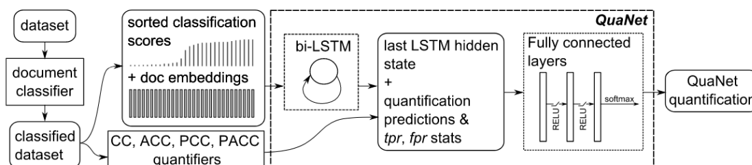
Figure 2.9: Architecture of QuaNet, taken from [37].
