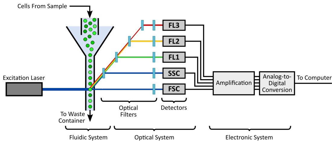
Figure 1.3: Diagram of a flow cytometer, illustrating the fluidic, optical and electronic systems. Image source: AAT Bioquest, Inc [8].
