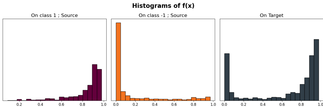
Figure 2.6: Figure inspired by Gonzalez et al. [59] with the data for Figure 2.1. The figure illustrates the output distributions of a kernel SVM for the two classes in the source (left and middle) and the target (right).
