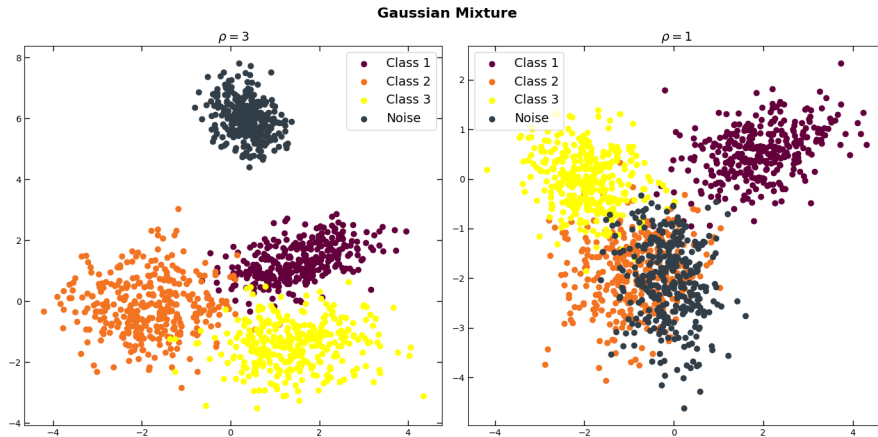
Figure 3.2: On both plots d = 2 , c = 3 , R = 2 , D = 1 and \varepsilon = 0.25 . With these parameters the plum, orange and yellow sources are well separated. On the left \rho = 3 and on the right \rho = 1 . In the light of our theoretical analysis, we expect robustness for RFFM for the left setting and no robustness for the right setting.
