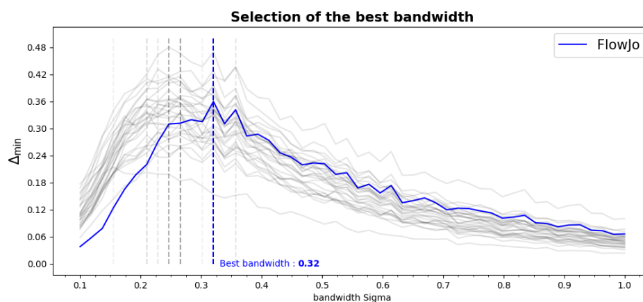
Figure 5.6: Value of the \Delta_{\min} criterion for different values of \sigma . In blue, the sources are a concatenation of all FlowJo gates. Each grey line corresponds to one patient. The grey dashed vertical lines are the argmax of each grey line and the blue dashed vertical line is the argmax of the blue line.
