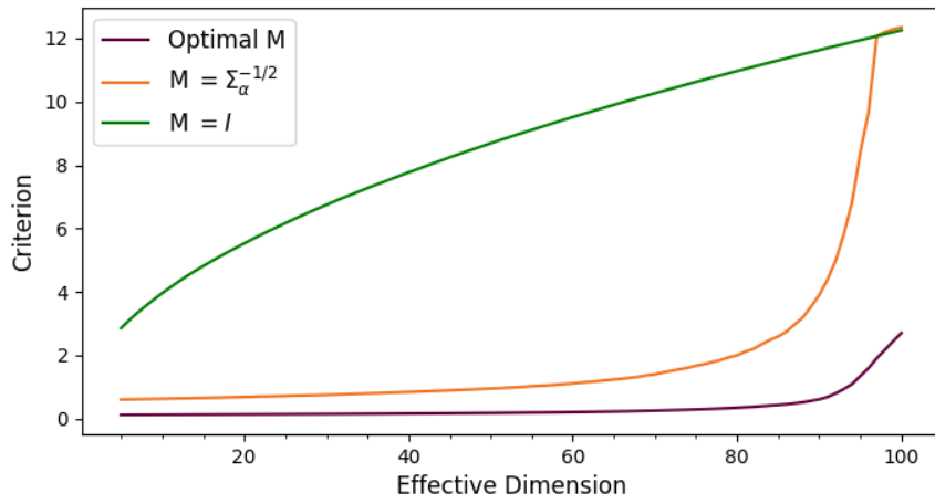
Figure 4.4: Value of criterion (4.6) for different effective dimensions D_{\text{eff}} , depending on the choice of matrix M .
