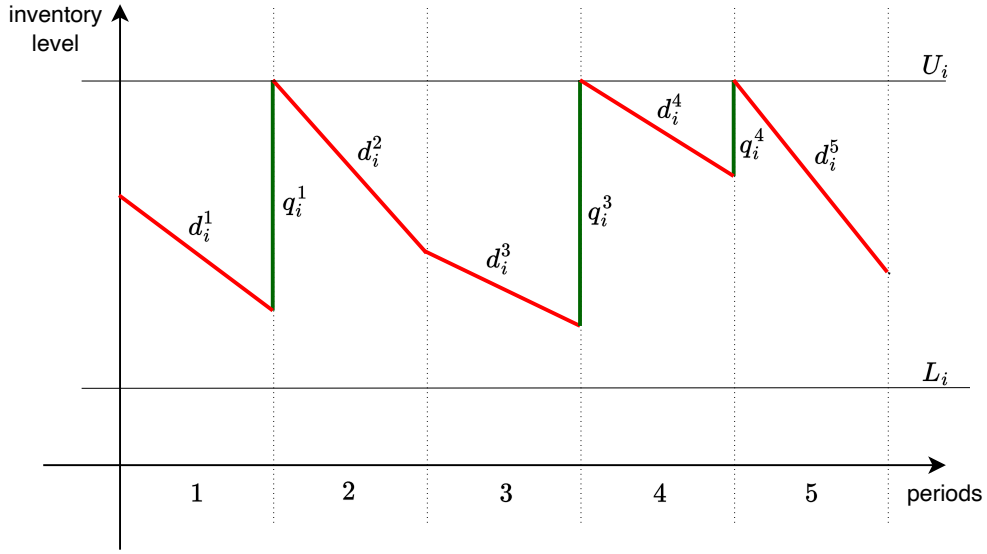
Figure 1.11: OU replenishment policy
