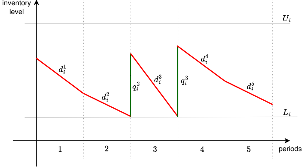
Figure 1.12: ZIO replenishment policy
