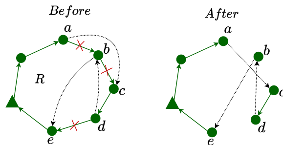
Figure 4.15: Insertion intra routes
