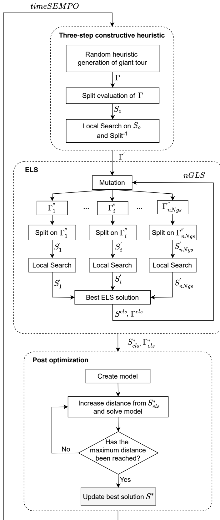
Figure 4.1: Schema of the SEMPO algorithm
