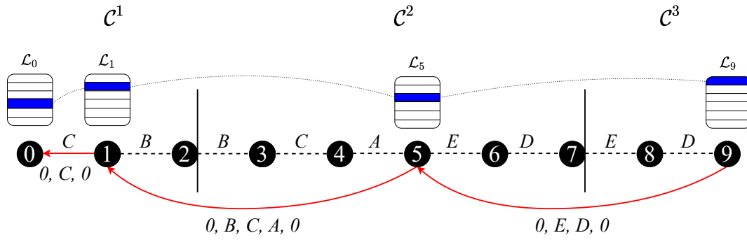
Figure 4.9: Retrieving the critical path
