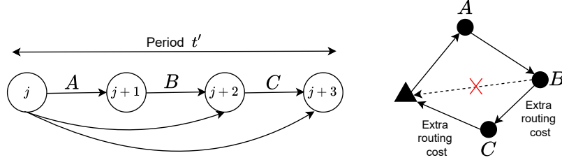
Figure 4.6: Addition of customer \Gamma_{j+3} in the route
