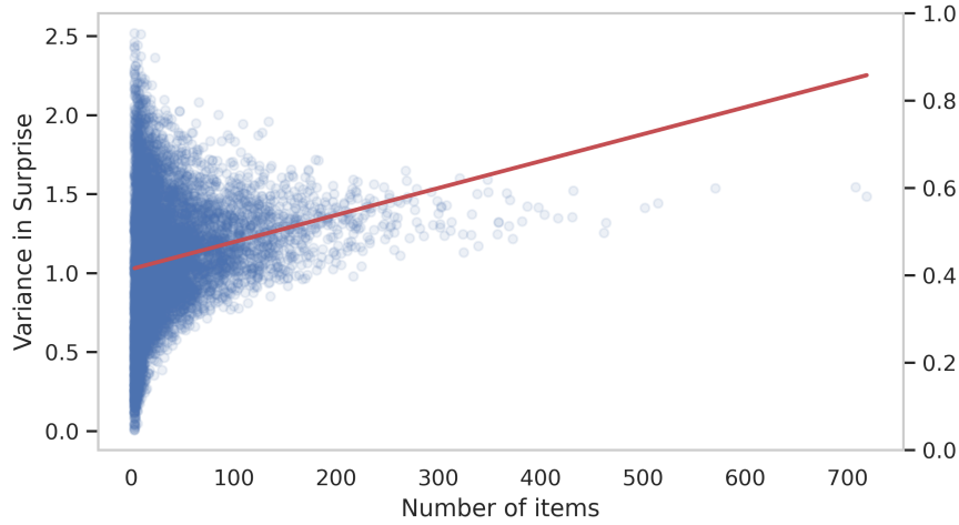
Figure 8.17: \text{std}(S(u)) vs |u| on the Netflix Small dataset, along with the linear fit
