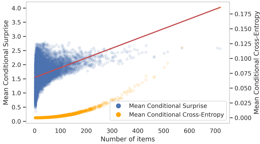
Figure 8.16: CS(u) and \widetilde{CS}(u) vs |u| on the Netflix Small dataset, along with the linear fit of CS(u) on |u|
