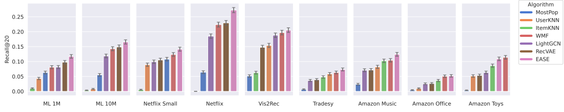
Figure 6.10: Overall algorithms performance across datasets, measured in Recall@20 with confidence intervals at 95%.
