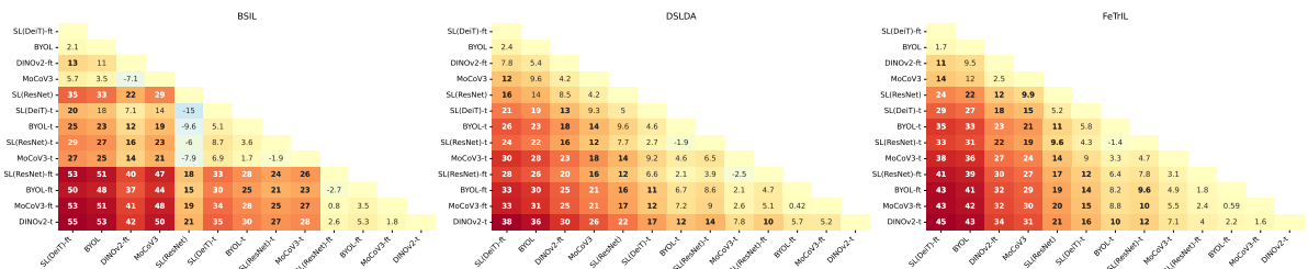
Figure 8.2: Pairwise accuracy gain per EFCIL algorithm. Significant values in bold (black or white font).
