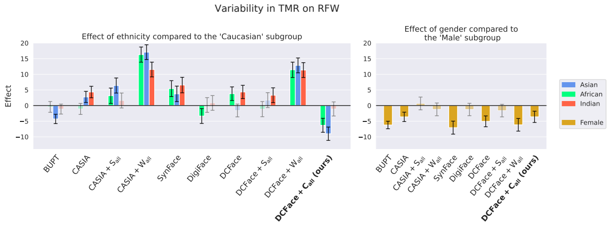
Figure 8.10: Marginal effects on TMR (lower in absolute is better) for each method compared to the unprotected group. Analysis done on RFW
