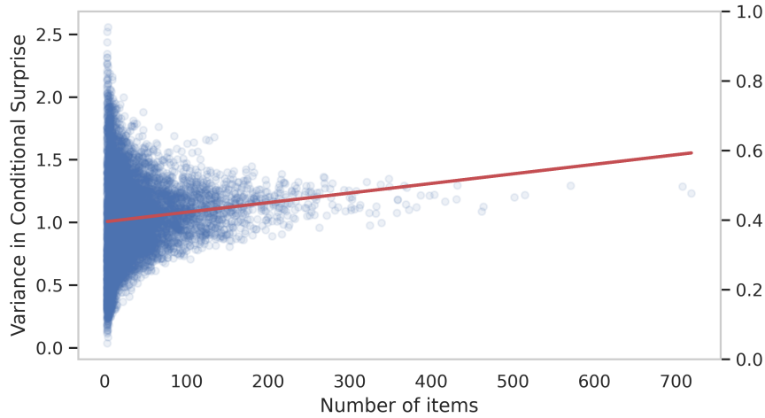
Figure 8.18: \text{std}(CS(u)) vs |u| on the Netflix Small dataset, along with the linear fit.
