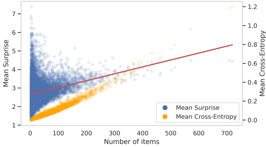
Figure 8.15: S(u) and \widetilde{S}(u) vs |u| on the Netflix Small dataset, along with the linear fit of S(u) on |u|
