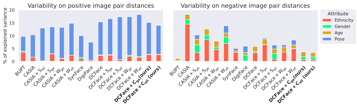
Figure 8.9: ANOVA results on BFW: total height corresponds to R^2 , the explained variance by the variables. Each bar is decomposed into multiple \eta^2 , i.e. the individual contributions to the variance
