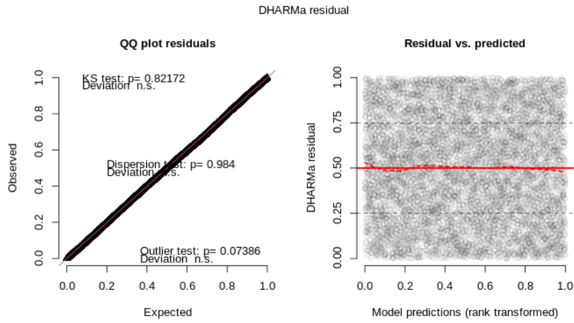
Figure 5.8: QQ-plot of residuals and Residual vs. predicted plot: logit model is adapted and log-odds are linear in the variables.
