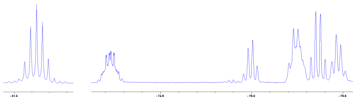
Figure 3. Crude (solution) ^{19}\text{F} NMR after cation exchange and extraction ( \text{Si-CF}_3 at -61.6\text{ppm} and ligands -\text{CF}_3 with special coupling at -74.2\text{ppm} ).
