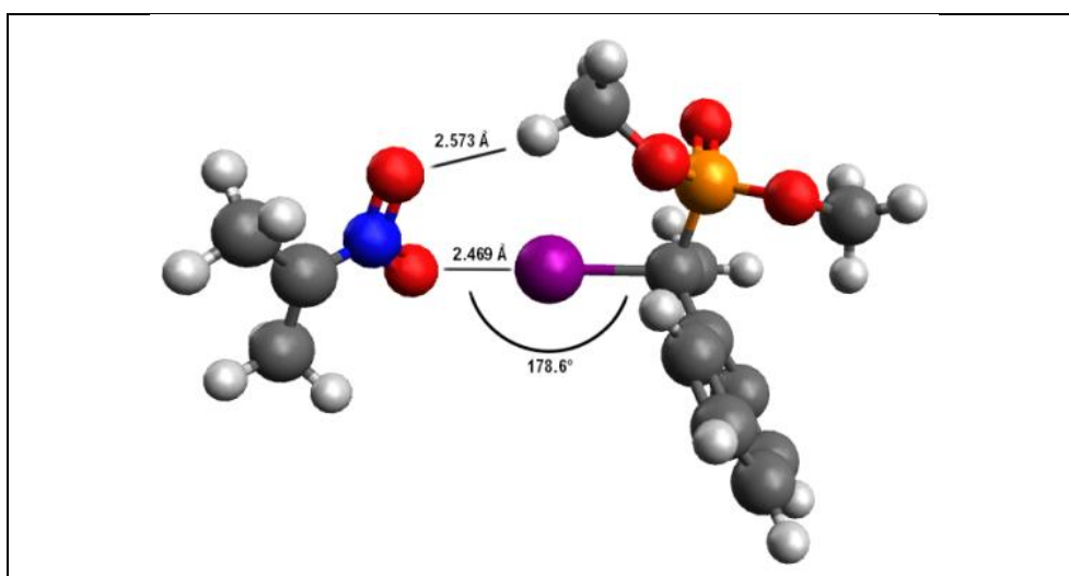
Figure 17. Optimized geometry between 2-nitropropane anion and iodo-phosphonate
