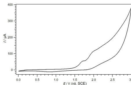
Figure 6. Cyclic voltammetry of 3 in DCM with [\text{Bu}_4\text{N}][\text{PF}_6] as supporting electrolyte.
