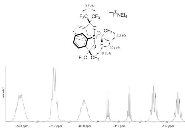
Figure 5. Attributed ^{19}\text{F} NMR coupling from ^{19}\text{F} NMR spectrum (bottom) of 3 .
