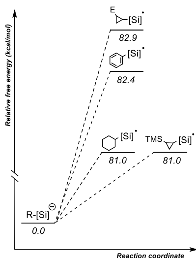
Figure 4. Relative free energy for the 1e - oxidation of anionic bis(catecholato) silicates.
