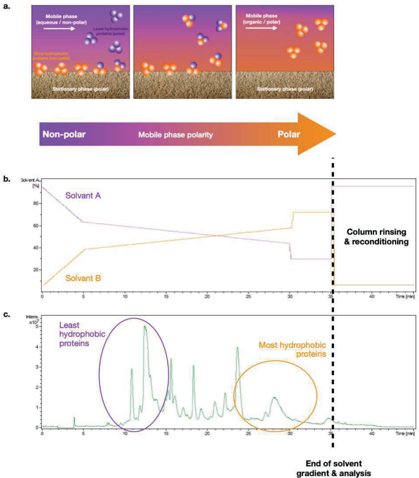
Figure 5. Reversed-phase chromatography: (a) Principle (b) Solvent gradient (c) Chromatogram
