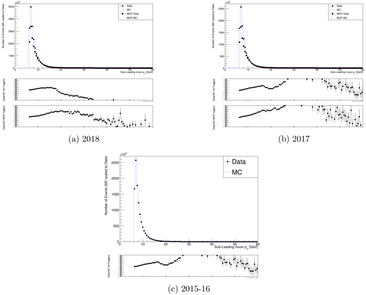
Figure 5.5: Sub-leading muon p_T^\mu for simulation and data using different trigger list: MC and Data for general trigger list, MCP MC and MCP Data for MCP trigger list. Selection applied is corresponding to Table 5.2
