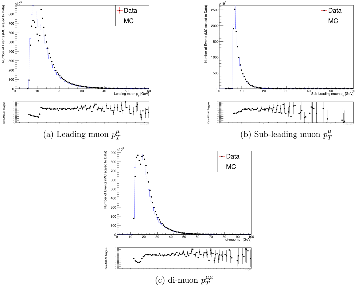
Figure 4.21: Comparison of data and simulation ( J/\psi ) for kinematic observables, for 2.8 < m_{\mu\mu} < 3.3
