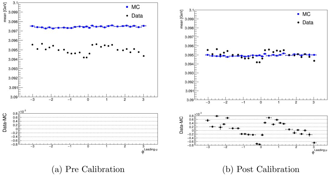
Figure 5.27: Mean of the m_{\mu\mu} distribution as a function of \phi^{\text{leading-}\mu} before and after calibration applied. The samples correspond to 2017 campaign, corrected for the calibration as a function of \eta^\mu presented in the Figure 5.23 .
