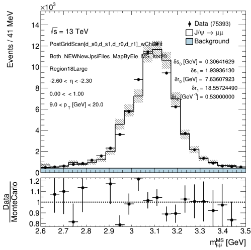
(b) Mass J/\psi 9.0 < p_T^{sub-leading} < 20.0
