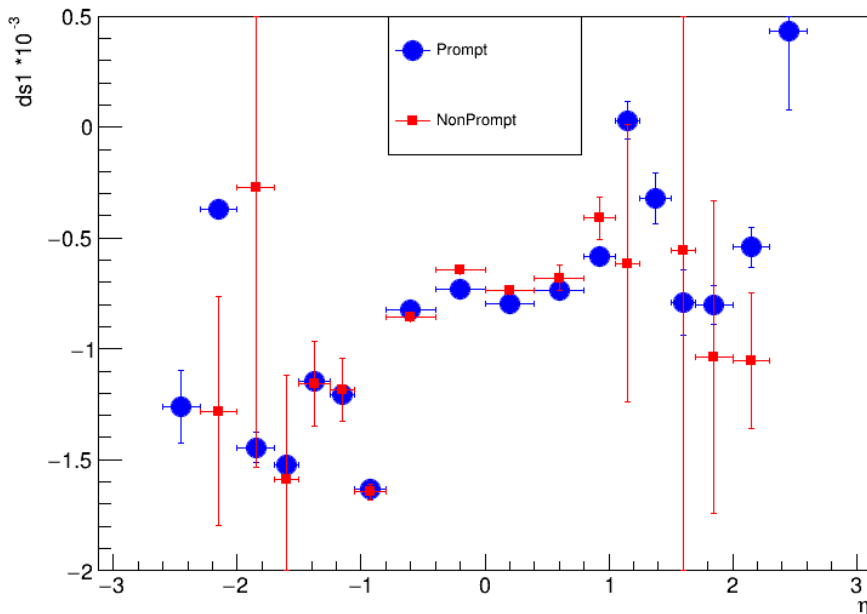
Figure 5.20: Scale as a function of \eta^\mu for Prompt (blue) and Non Prompt (red) J/\psi samples, Prompt data and MC and Non Prompt MC are re-weighted to Non Prompt data as defined in Table 5.6. ID tracks. Points are average over iterations and error bars are Standard Deviation.
