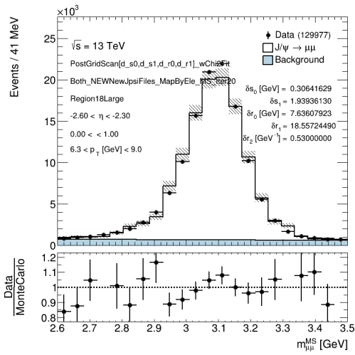
(a) Mass J/\psi 6.3 < p_T^{sub-leading} < 9.0
