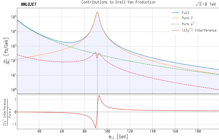
Figure 1.10: Theoretical prediction of Z, \gamma interference as a function of m_{ll} at Drell-Yan process, in the context of a hadron collider, calculated at LO in QCD. Top panel shows absolute values of pure Z , pure \gamma and Z/\gamma interference. The bottom plot shows ratio of Z\gamma to \gamma pure contributions. Black dotted line is at \approx m_Z pole. Taken from ref. [23].
