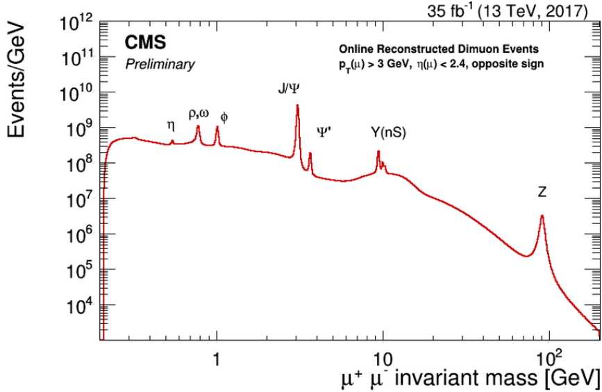
Figure 1.9: Di-muon mass spectrum in CMS from Run-2 (2017 and 2018 campaigns). Taken from ref. [22].
