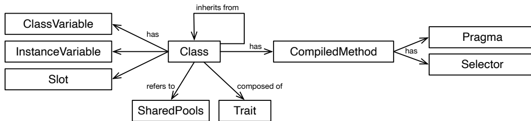
Figure 2.1: The structural Pharo metamodel: Class aggregates variables, methods, constant management (SharedPools) and method annotation (Pragma) and exposes related APIs.
