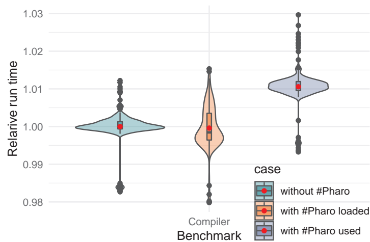
Figure 7.4: Results with lookup cache enabled on the Compiler benchmark. Lower is better. Red dots mark the average.
