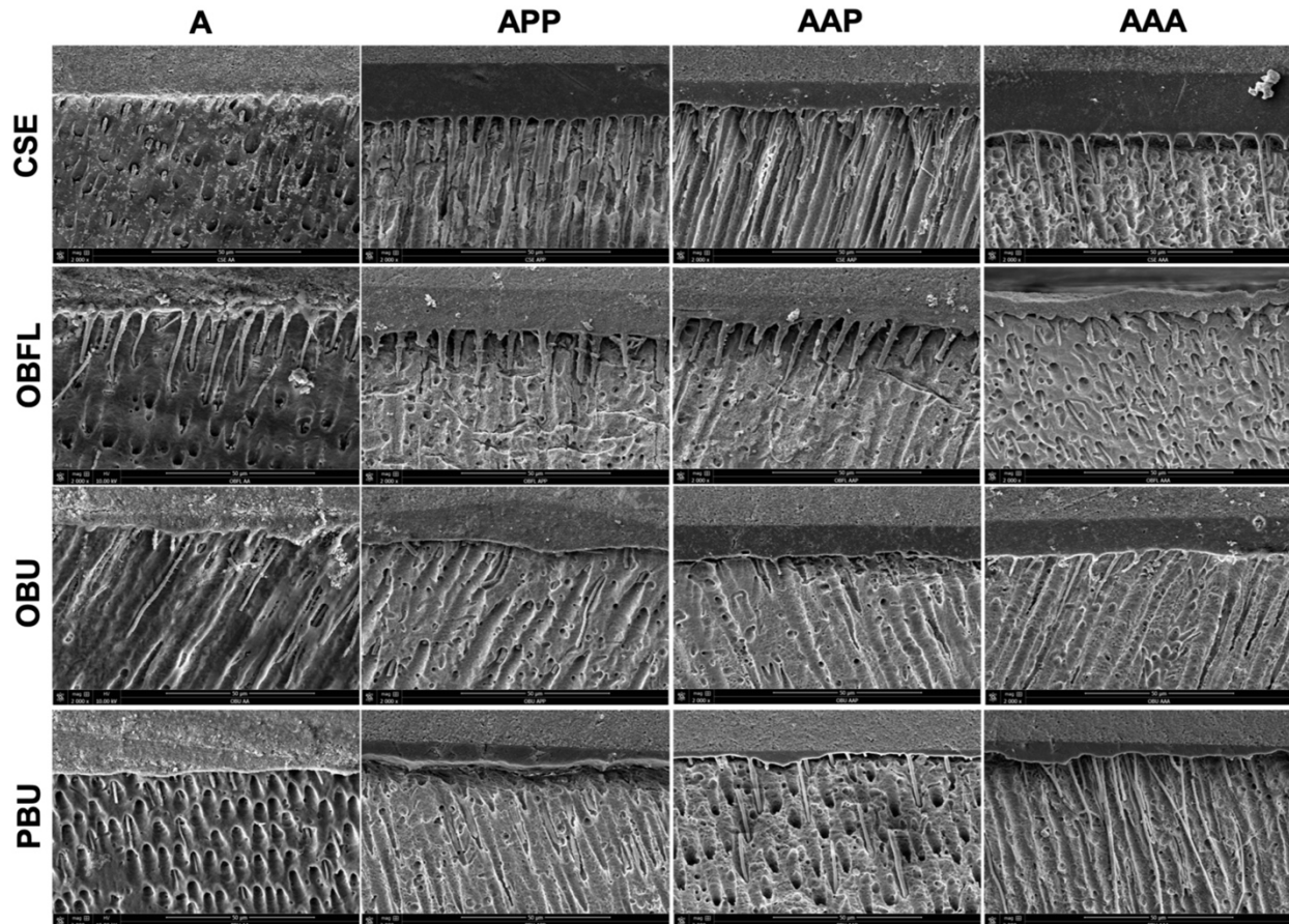
Figure 35: Scanning electron microscopy images ( \times 2000 magnifications) determine the adhesive layer and resin tag infiltration of the distinctive dental adhesive systems examined with the modified triple-layer application and the control group. Clearfil SE Bond (CSE); OptiBond FL (OBFL); OptiBond Universal (OBU); Prime&Bond Universal (PBU); Single active application (A); triple application, Active–Passive–Passive (APP); triple application, Active–Active–Passive (AAP); triple application, Active–Active–Active (AAA).
