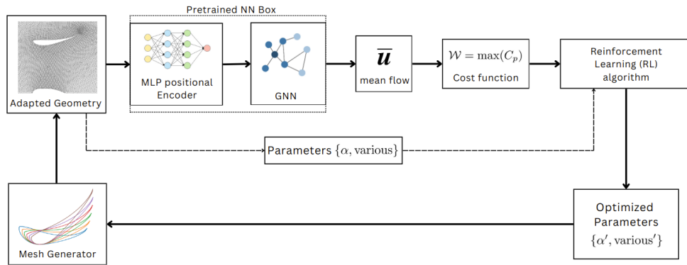
Figure 8.7: End-to-end optimization loop; the complete mesh along with the control variable \alpha are the NN's block input (Sec. 8.4); \bar{u} is the GNN's predicted mean flow; C_p is power coefficient to maximize.
