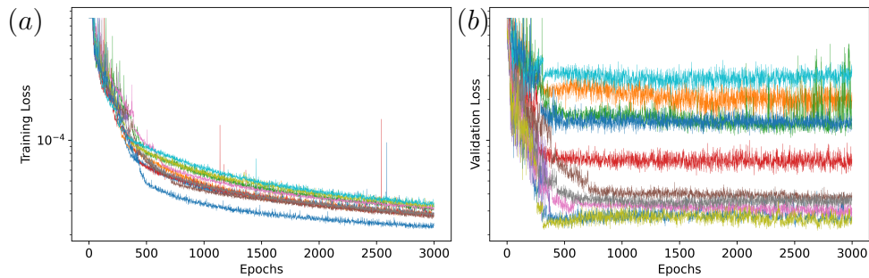
Figure 6.10: Training and validation loss curves for models trained using 10 k -fold up to 3000 epochs. (a) shows the training curves, (b) the corresponding validation curves for each fold.
