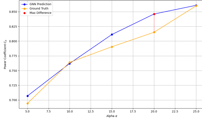
Figure 8.9: Ground truth C_p values for duct angles \alpha ranging from 5^\circ to 25^\circ , used as a reference dataset for optimization as compared with the C_p obtained by the GNN predicted flows.
