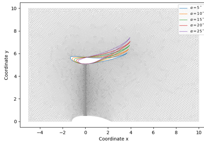
Figure 8.10: Cross-sectional generated mesh with refinement near the actuator disk at x = 0 along with the different duct positioning based on the angle \alpha from 5^\circ to 25^\circ
