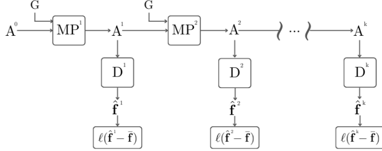
Figure 4.3: The overall framework of our GNN training process. MP^k are the message passing algorithms; D^k are the k decoders trainable MLPs; \mathbf{A}^k are the k matrices containing the embedded states from each node; \mathbf{G} is the vector containing the input injected in the GNN. Figure inspired by Donon et al. [2020] .
