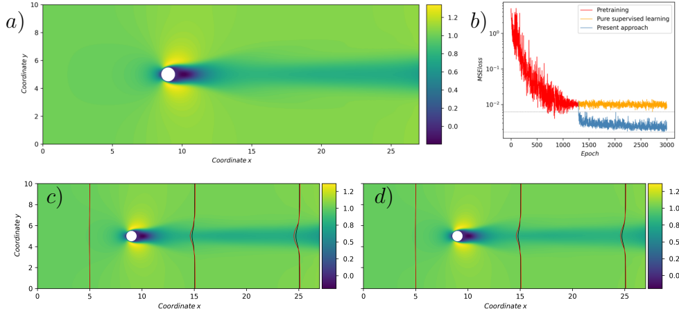
Figure 7.4: (a) The training mean flow input (at Re = 120 ) from the ground truth. The training dataset is composed by 3 meanflow-forcing pair at Reynolds number Re = [90, 110, 130] while the validation dataset contains cylinder cases at Re = [120, 150] ; (b) the loss curves for the pure supervised learning (orange line) and the proposed approach (blue line) are shown. The two horizontal dotted lines indicate the minimum values of both curves, while the dotted vertical line indicates the end of the pre-training phase (Sec. 7.2.2); (c) the reconstructed mean flow (at Re = 120 ) from the pure supervised approach; (d) the reconstructed mean flow (at Re = 120 ) from the present approach. 1D line plots are overlaid on figures (c) and (d), comparing the predicted flow values (red line) with the ground truth (black line) at various sections along the flow field.
