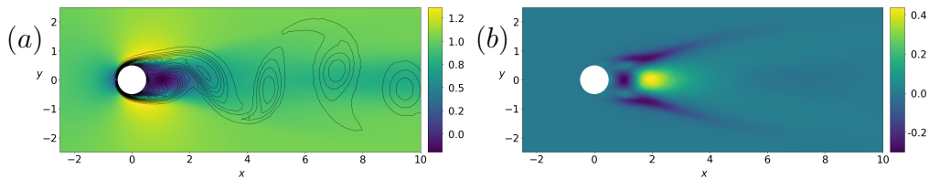
Figure 6.1: (a) Stream-wise component of the meanflow \bar{\mathbf{u}} and vorticity isolines \omega = \nabla \times \mathbf{u} for the flow past a cylinder at Re = 150 . (b) For the same case, the stream-wise component of the closure term \mathbf{f} is shown. In both cases, only a portion of the domain is shown.
