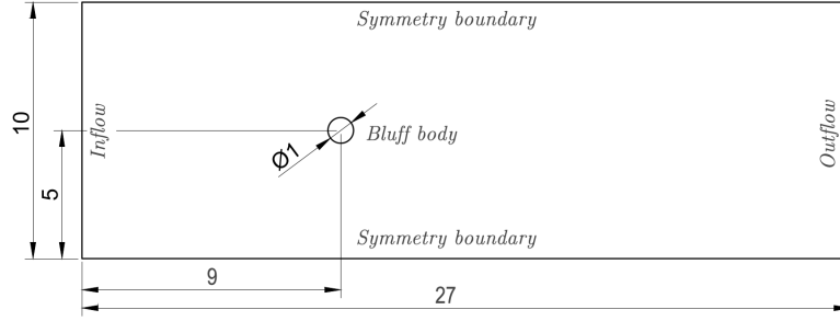
Figure 6.2: Sketch of the computational domain geometry. The diameter of the circumscribed circle of the bluff body, the height and length of the domain are given in non-dimensional units.
