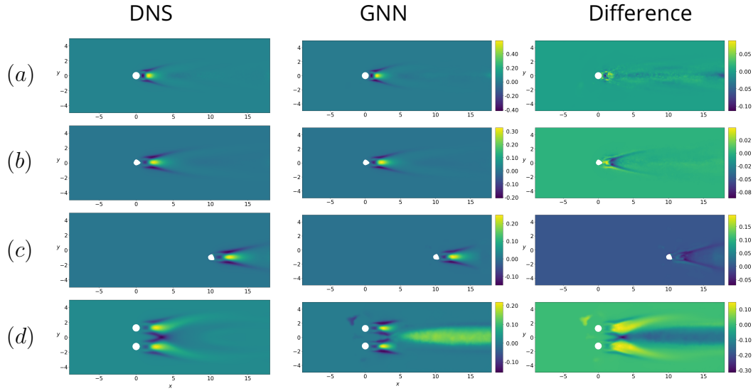
Figure 6.7: Stream-wise component comparison of the Reynolds stress tensor. The GNN's model is trained with a dataset composed by 11 cases of cylinder shape bluff bodies, ranging in 50 \leq Re \leq 150 , \Delta Re = 10 . (a) Case 1, Re = 200 , cylinder bluff body shape; (b) Case 2, Re = 120 , random shape bluff body; (c) Case 3, Re = 100 , random shape shifted bluff body; (d) Case 4, Re = 90 , flow past two side-by-side cylinders.
