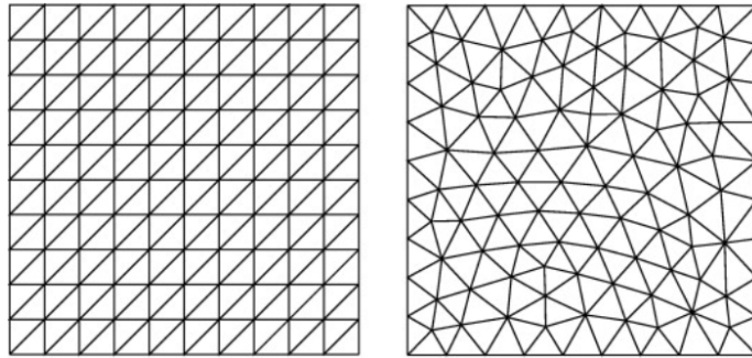
Figure 3.4: (Left) Structured mesh (Right) Unstructured mesh
