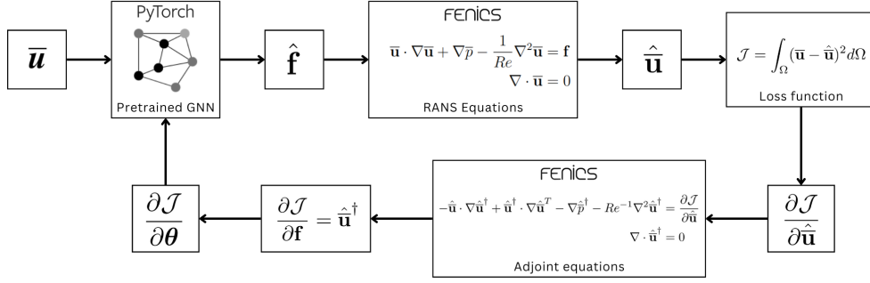
Figure 7.1: End-to-end training loop; \bar{\mathbf{u}} is the GNN's input mean flow; \hat{\mathbf{f}} is the GNN's predicted forcing stress term; \theta are the GNN's trainable parameters; \mathcal{J}(\hat{\mathbf{u}}) is the cost function to minimize.
