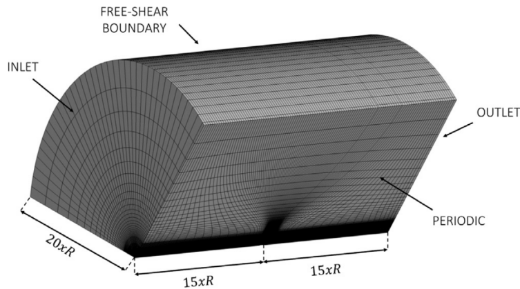
Figure 8.4: Representation of a portion of the computational domain along with the adopted boundary conditions. Figure adapted from Bontempo and Di Marzo [2023]
