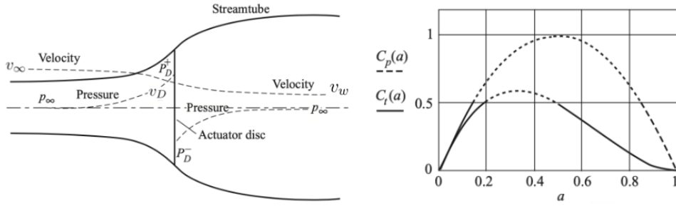
Figure 8.1: (Left) Representation of the actuator disk configuration for a wind turbine. (Right) Power coefficient C_p as a function of the axial flow induction factor a for a wind turbine.
