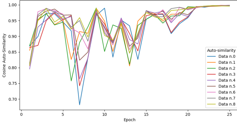
Figure 6.13: Visualization of gradient auto-similarity convergence over multiple training epochs using MAE for 9 distinct cases within the training data set.
