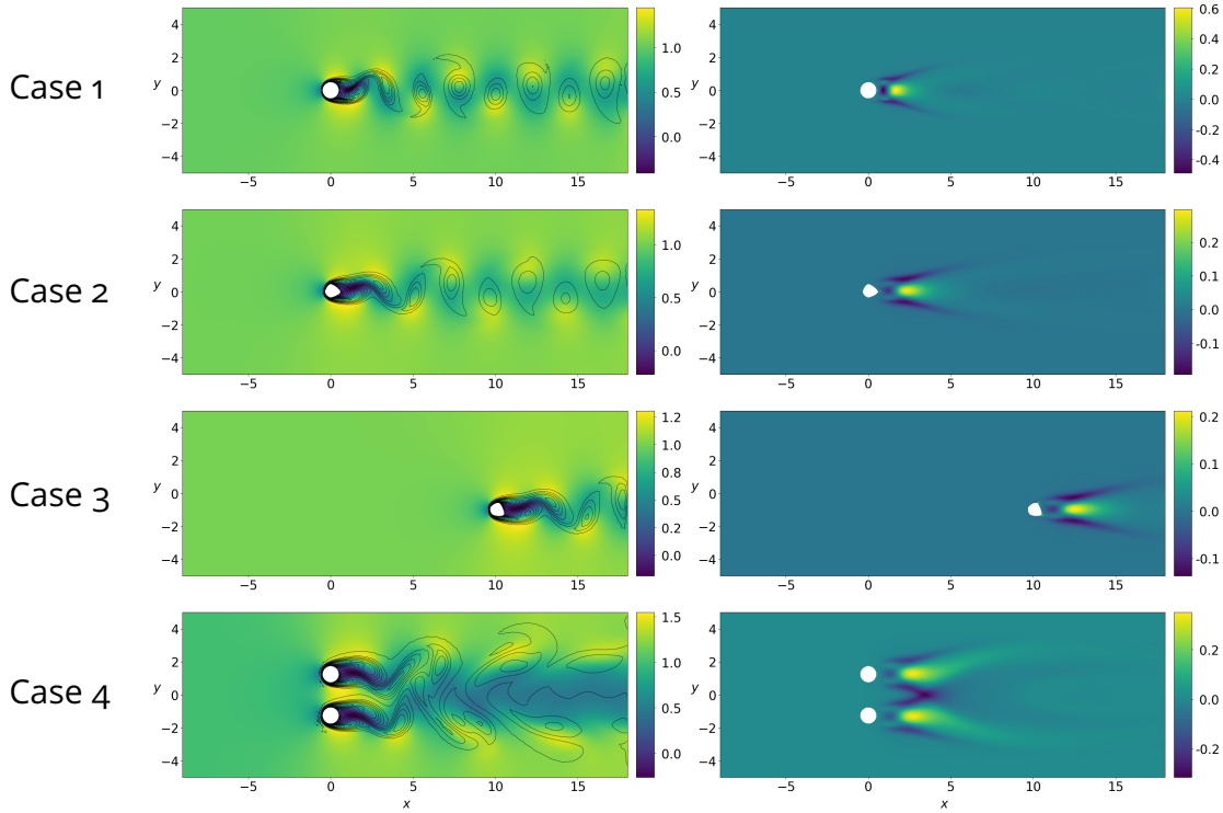
Figure 6.5: Test cases used as a benchmark of the learning strategies discussed in Sec. 6.3. From the top row to the bottom one: Case 1, cylinder flow at Re = 200 ; Case 2, flow past a random-shaped bluff body at Re = 120 ; Case 3, flow past a random-shaped bluff body shifted in the computational domain at Re = 100 ; Case 4, flow past a two side-by-side cylinders configuration at Re = 90 . For each of the cases, the left column shows the stream-wise component of the meanflow \bar{u} , along with the vorticity isolines \omega = \nabla \times \mathbf{u} , while the right column show the stream-wise component of the forcing stress \mathbf{f} .
