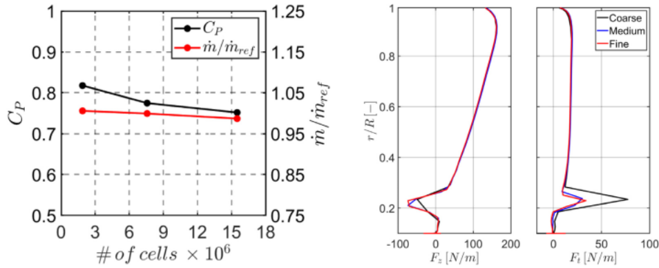
Figure 8.5: Grid independence test. (Left) Power Coefficient C_p and mass flow rate ingested by the rotor (Right) Linear density of the axial and tangential forces. Figure taken from Bontempo and Di Marzo [2023]
