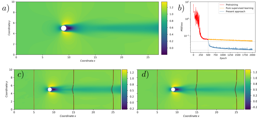
Figure 7.2: (a) The training mean flow input from the ground truth. The training dataset is composed by 1 meanflow-forcing pair at Reynolds number Re = 150 ; (b) the loss curves for the pure supervised approach (orange line) and the proposed approach (blue line) are shown. The two horizontal dotted lines indicate the minimum values of both curves, while the dotted vertical line indicates the end of the pre-training phase (Sec. 7.2.2); (c) the reconstructed mean flow from the pure supervised approach; (d) the reconstructed mean flow from the present approach. 1D line plots are overlaid on figures (c) and (d), comparing the predicted flow values (red line) with the ground truth (black line) at various sections along the flow field.
