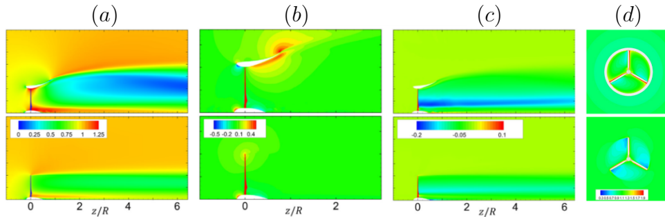
Figure 8.6: Comparison between the ducted (DAWT) (Top) and open (OWT) (Bottom) configurations for V_\infty = 7\text{m/s} : (a) azimuthally-averaged normalized axial velocity, (b) azimuthally-averaged normalized radial velocity contours, (c) azimuthally-averaged normalized tangential velocity contours, (d) normalized axial velocity contours at the rotor plane. Figure adapted from Bontempo and Di Marzo [2023]
