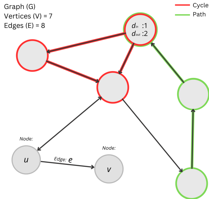
Figure 4.2: A pictorial representation of a graph G (Eq. 4.15)
