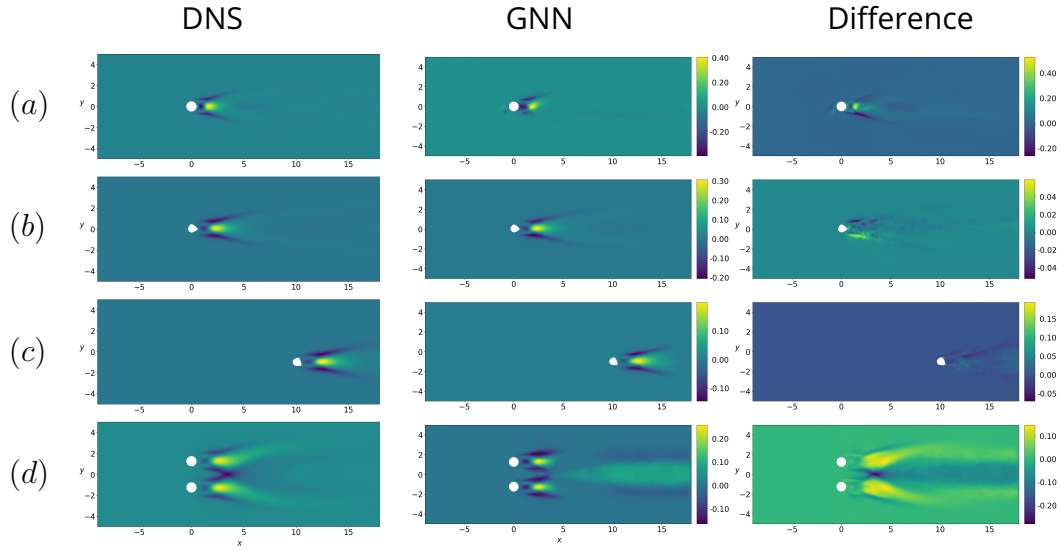
Figure 6.9: Stream-wise component comparison of the Reynolds stress tensor. The GNN's model is trained with a dataset composed by 11 cases of random shaped bluff bodies, ranging in the interval 50 \leq Re \leq 150 , \Delta Re = 10 . (a) Case 1, Re = 200 , cylinder bluff body shape; (b) Case 2, Re = 120 , random shape bluff body; (c) Case 3, Re = 100 , random shape shifted bluff body; (d) Case 4, Re = 90 , flow past two side-by-side cylinders.
