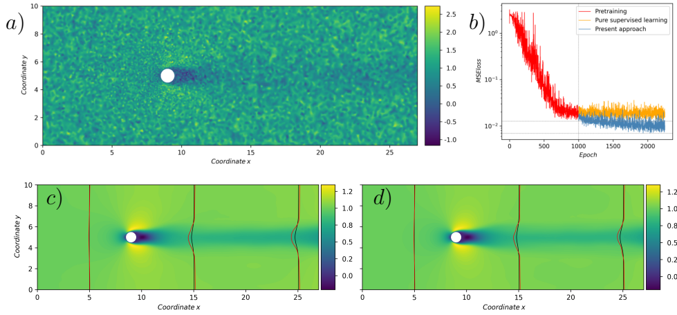
Figure 7.6: (a) Gaussian perturbed mean flow (at Re = 110 ). The training dataset is composed by 3 mean flow-forcing pairs at Reynolds number Re = [90, 110, 130] perturbed with a Gaussian noise having \mu = 0 and \sigma = [0.6, 0.4, 0.2] , respectively; (b) the loss curves for the pure supervised approach (orange line) and the proposed approach (blue line) are shown. The two horizontal dotted lines indicate the minimum values of both curves, while the dotted vertical line indicates the end of the pre-training phase (Sec. 7.2.2); (c) the reconstructed mean flow (at Re = 110 ) from the pure supervised approach; (d) the reconstructed mean flow (at Re = 110 ) from the present approach. 1D line plots are overlaid on figures (c) and (d), comparing the predicted flow values (red line) with the ground truth (black line) at various sections along the flow field.
