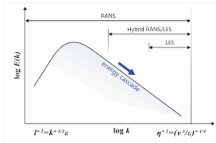
Figure 3.2: The Kolmogorov Energy Cascade
