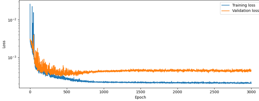
Figure 6.11: Training and validation loss curves are shown when AL with similarity threshold 0.8 is performed until 3000 epochs. The training dataset is formed by 6 random shaped bluff bodies. Their Reynolds number varies in the interval 50 \leq Re \leq 150 . The validation set is formed by the test cases presented in Sec. 6.3.1.
