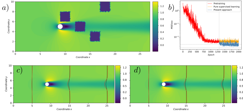
Figure 7.7: (a) Patch mask applied on the mean flow (at Re = 110 ). The training dataset is composed of 3 mean flow-forcing pairs at Reynolds number Re = [90, 110, 130] with randomly located patching mask; (b) the loss curves for the pure supervised approach (orange line) and the proposed approach (blue line) are shown. The two horizontal dotted lines indicate the minimum values of both curves, while the dotted vertical line indicates the end of the pre-training phase (Sec. 7.2.2); (c) the reconstructed mean flow (at Re = 110 ) from the pure supervised approach; (d) the reconstructed mean flow (at Re = 110 ) from the present approach. 1D line plots are superimposed on figures (c) and (d), comparing the predicted flow values (red line) with the ground truth (black line) at various sections along the flow field.
