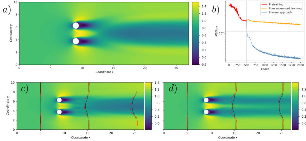
Figure 7.3: (a) The training mean flow input from the ground truth. The training dataset is composed by 1 meanflow-forcing pair at Reynolds number Re = 90 ; (b) the loss curves for the pure supervised approach (orange line) and the proposed approach (blue line) are shown. The two horizontal dotted lines indicate the minimum values of both curves, while the dotted vertical line indicates the end of the pre-training phase (Sec. 7.2.2); (c) the reconstructed mean flow from the pure supervised approach; (d) the reconstructed mean flow from the present approach. 1D line plots are overlaid on figures (c) and (d), comparing the predicted flow values (red line) with the ground truth (black line) at various sections along the flow field.
