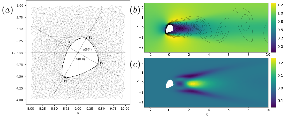
Figure 6.4: Flow past a bluff body with a randomly generated shape at Re = 90 . (a) Geometry of the bluff body with \alpha = 60^\circ and unitary diameter of the circumscribed circle around the body. The resulting meanflow and the vorticity isolines \omega = \nabla \times \mathbf{u} are shown in (b), while (c) shows the forcing stress term in a portion of the domain.
