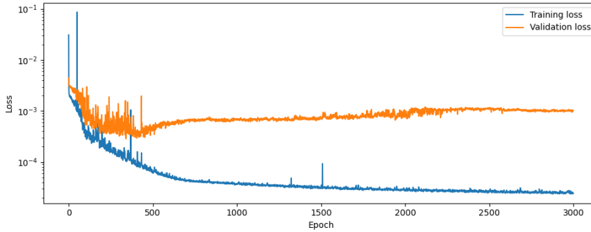
Figure 6.8: Curves for the training and validation loss for when DA is performed by introducing 11 cases of flows past random geometries in the dataset. The Reynolds number varies in the range 50 \leq Re \leq 150 with \Delta Re = 10 . The training runs until 3000 epochs. The validation set is formed by the test cases presented in Sec. 6.3.1.
