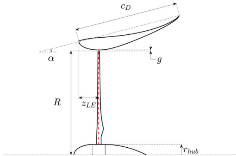
Figure 8.3: Sketch of a ducted wind turbine DAWT reporting the relevant geometrical parameters. Figure adapted from Bontempo and Di Marzo [2023] .
