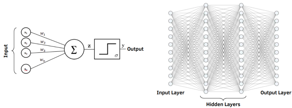
Figure 4.1: (Left) A Perceptron and (Right) a Multi-Layer Perceptron MLP representation.
