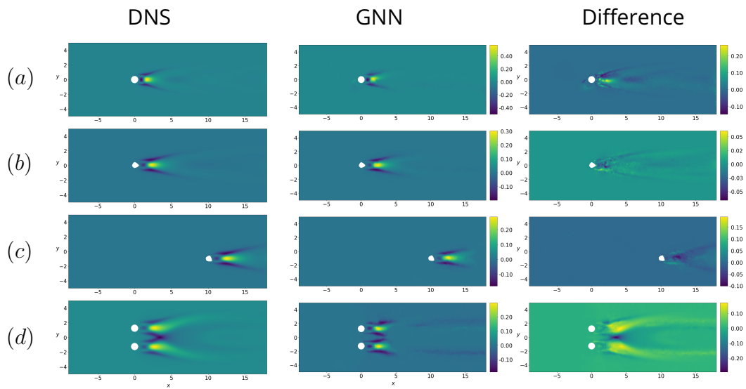
Figure 6.12: Stream-wise component comparison of the Reynolds stress tensor. The GNN's model is trained with a dataset composed by 6 cases of bluff bodies of random shape selected with the AL approach, ranging in the interval 50 \leq Re \leq 150 , \Delta Re = 10 . (a) Case 1, flow past a cylinder at Re = 200 ; (b) Case 2, flow past a random shaped bluff body at Re = 120 ; (c) Case 3, random shaped bluff body at Re = 100 , shifted downstream; (d) Case 4, flow past two side-by-side cylinders at Re = 90 .
