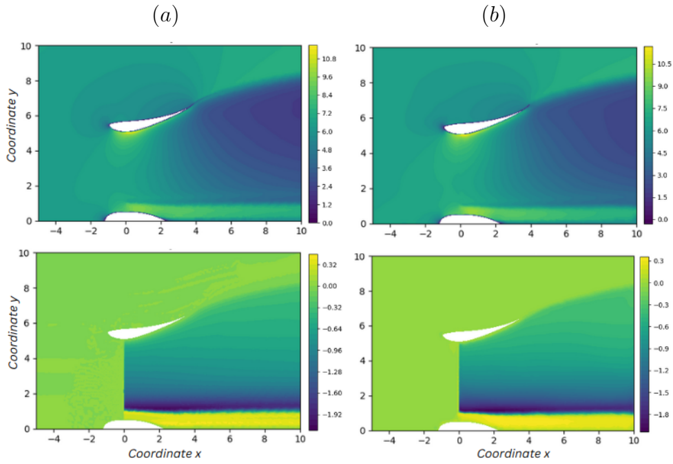
Figure 8.8: Comparison of flow fields for \alpha = 15^\circ (not included in the training dataset). (a) the ground truth flow fields, (b) the GNN flow fields prediction, (Top) axial velocity component, (Bottom) swirl velocity component.
