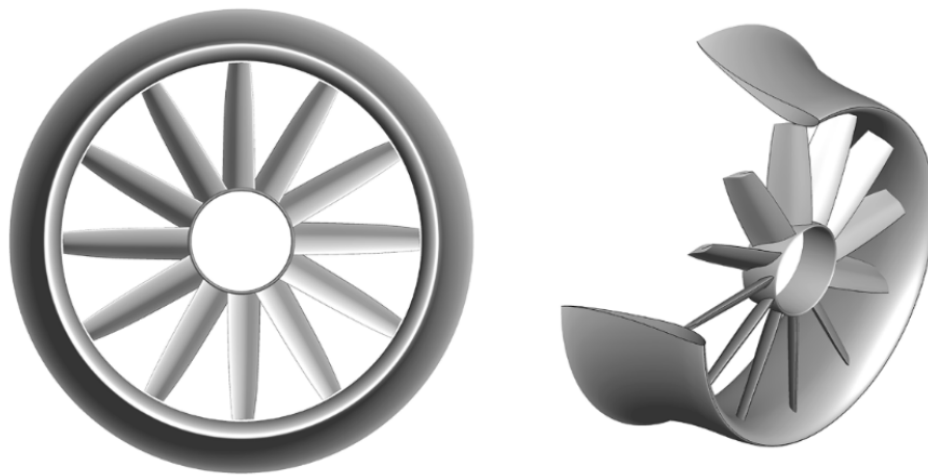
Figure 8.2: (Left) Frontal view of a Diffuser-Augmented Wind Turbine (DAWT) and its perspective view (Right). Figure inherited from Bontempo and Manna [2022]
