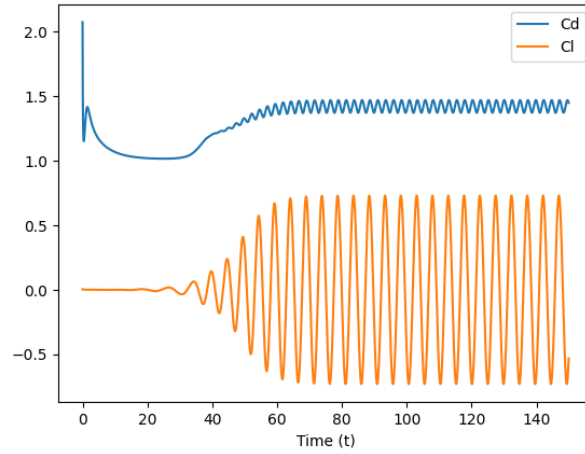
Figure 6.3: Drag coefficient C_d and lift coefficient C_l of flow past a cylinder.
