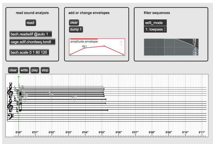
Figure 4.7: Max/MSP example patch of additive resynthesis of sound analysis using Koryphaïos .
