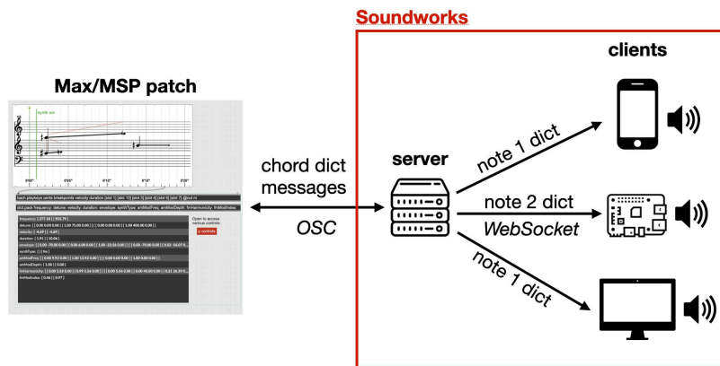
Figure 4.2: Diagram of the communication between the different parts of Koryphaïos .
