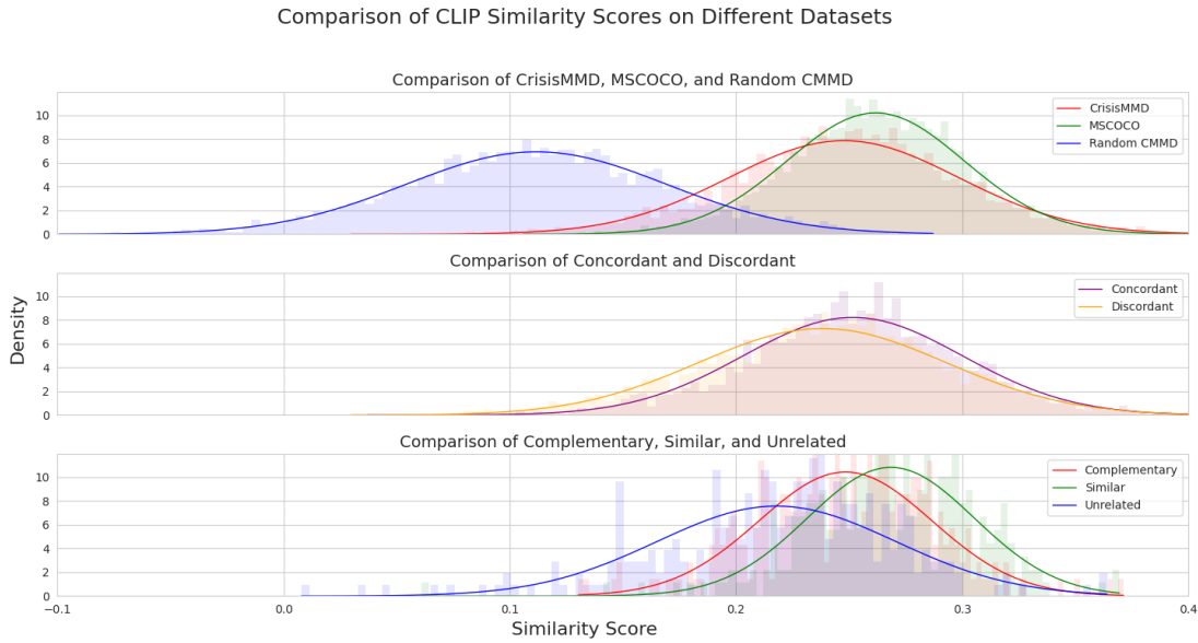
Figure 3.8: Comparison of CLIP Similarity Scores across different datasets and pair types.
