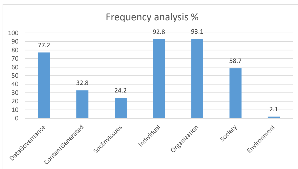
Figure 25: Incidents distribution
