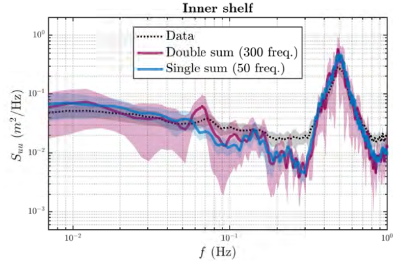
Figure III.9 Longshore-average power spectra of the cross-shore velocity ( S_{uu} ) as a function of frequency ( f ) for station located in the innershell (left, x = 26.6 m, -10 < y < 10 m). The spectrum from experimental data is shown as black dots, while those from simulations with the double-sum (300 freq.) and single-sum (50 freq.) wavemakers are shown as pink and blue lines, respectively. The longshore standard deviations of the model and data spectra are represented by shaded areas.
