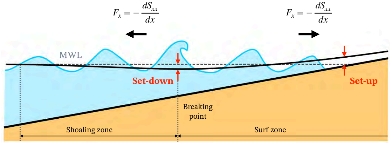
Figure I.8 Descriptive sketch of set-down and set-up caused by waves (re-adapted from geo.libretexts.org )
