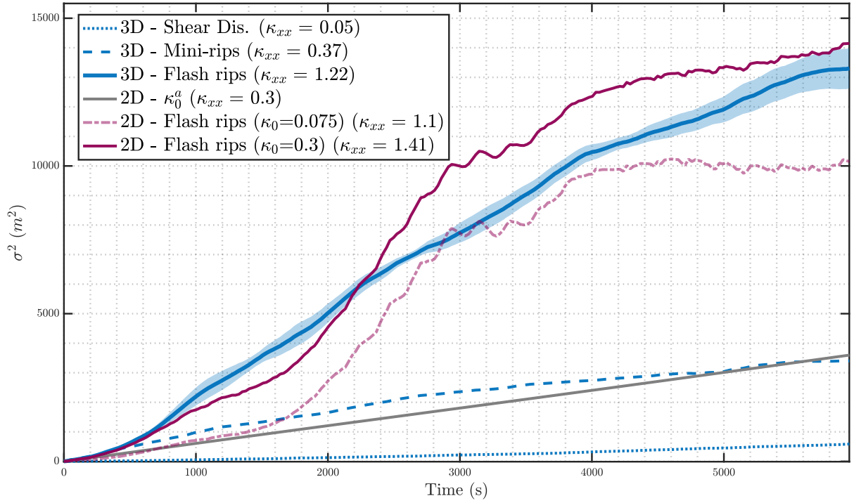
Figure IV.15 Cross-shore variance \sigma^2 of tracer concentration as a function of time for the idealized IB09 simulations described in Table IV.2. The shaded area represents the standard error of the ensemble simulations of 3D-FlashR ( \sigma/\sqrt{N} with N the number of simulations performed).
