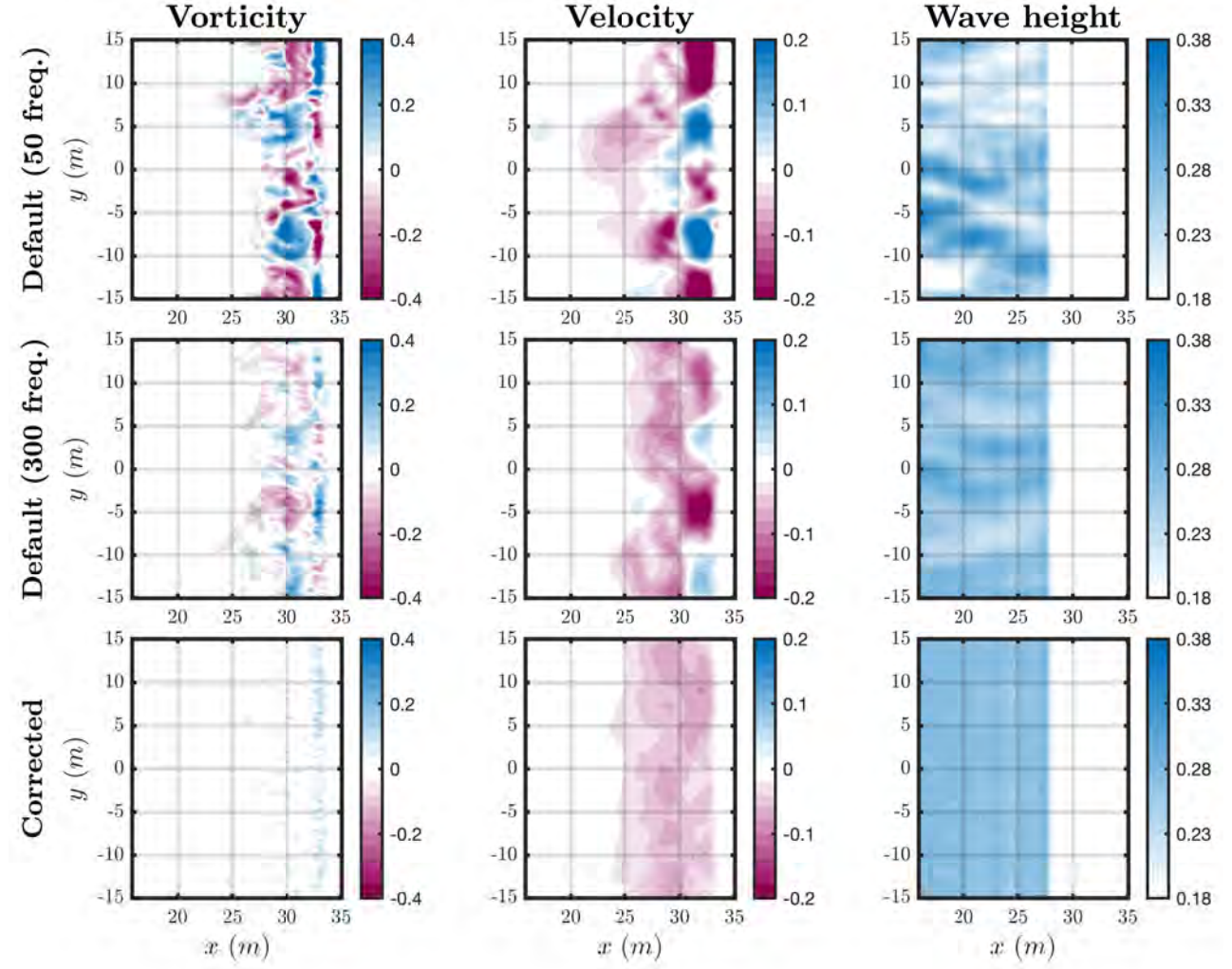
Figure III.5 Time-averaged ( t = 10 - 30 min) surface vertical vorticity \omega_z (s -1 , left), alongshore velocity v (m.s -1 , middle) and significant wave height H_s (m, right) for the double-sum (top: N = 50 freq., middle: N = 300 freq.) and single-sum (bottom: N = 50 freq.) wavemakers in the G1d case ( \sigma_\theta = 26.1^\circ ).
