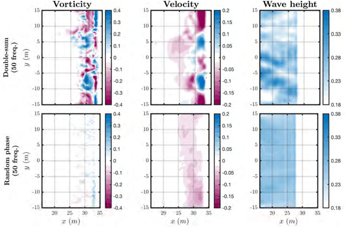
Figure III.11 Time-averaged ( t = 10 - 30 min) surface vertical vorticity \omega_z ( \text{s}^{-1} , left), alongshore velocity v ( \text{m.s}^{-1} , middle) and significant wave height H_s (m, right) for the default double-sum wavemaker (top) and the modified double-sum wavemaker with random phase (bottom), using N = 50 freq in the G1d case ( \sigma_\theta = 26.1^\circ ).
