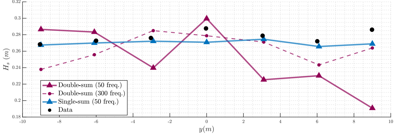
Figure III.6 Significant wave height H_s (m) for G1d ( \sigma_\theta = 26.1^\circ ) at all offshore stations along the coast ( x = 19.0 m, -9 < y < 9 m). The data (black circles) is from wave gauges and the model values from the double-sum (pink triangles for N = 50 freq. and pink dots for N = 300 freq.) and single-sum (blue triangles) wavemaker simulations computed at the same locations.
