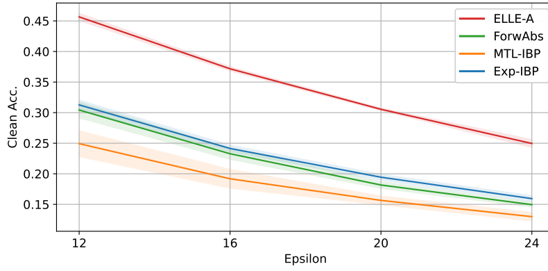
(b) CIFAR-100.
