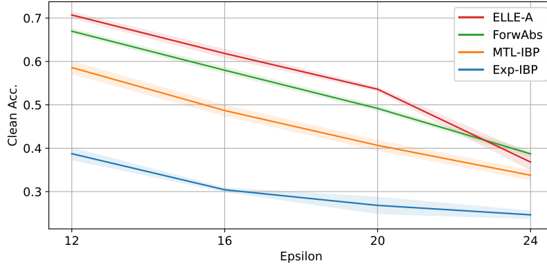
(a) CIFAR10.
