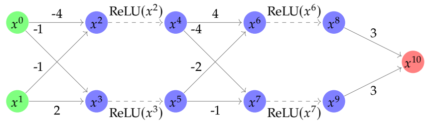
Figure 2.4: A simple neural network with 2 hidden layers, input of dimension 2 and a single output. Following the notations of Example 2.1.1, the weight matrices are: \left\{ \begin{pmatrix} -4 & -1 \\ -1 & 2 \end{pmatrix}, \begin{pmatrix} 4 & -2 \\ -4 & -1 \end{pmatrix}, (3 \quad 3) \right\} , the biases are omitted for clarity. The input is represented in green, the hidden layers in blue and the output in red. We decouple the application of the linear function from the activation function, deviating from the common graph representation to better illustrate how non-linearities are handled when approximating the reachable space of a network. The nodes immediately before the activation functions are called Pre-Activation nodes (or Pre-ReLU in the case of ReLU activations).
