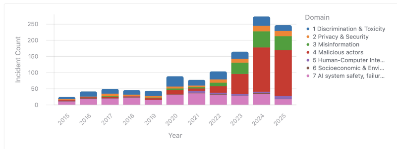
Figure 1.1: Incidents involving AI systems since 2015. The chart comes from https://airisk.mit.edu/ai-incident-tracker/timeline-risk-classification , the data from https://incidentdatabase.ai/ . Completing the legend: 5: Human-Computer Interaction, 6: Socioeconomic and Environmental, 7: AI system safety, failures and limitations.
