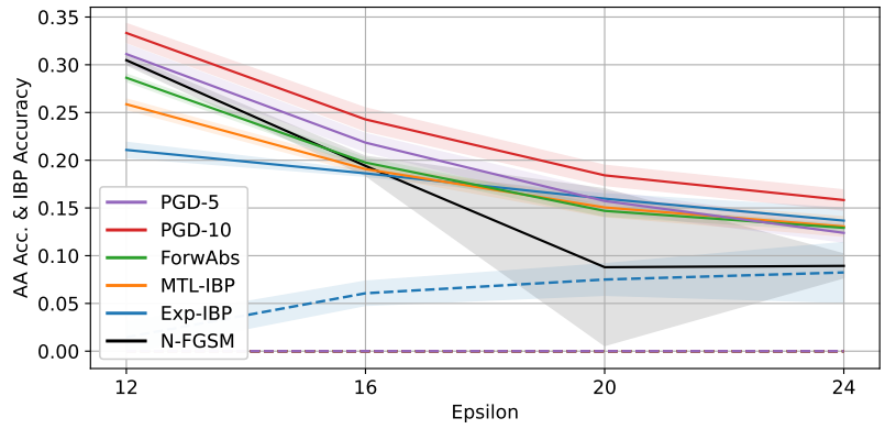
(a) AA (solid lines) and IBP (dashed) accuracies. Means over 5 repetitions and their 95% CIs.
