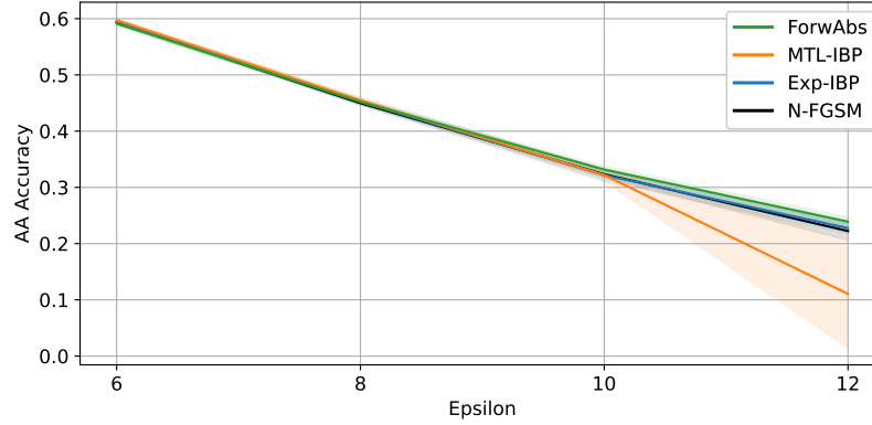
(b) SVHN
