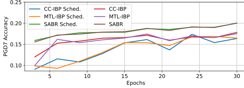
(a) Empirical accuracy under PGD7 attacks.
