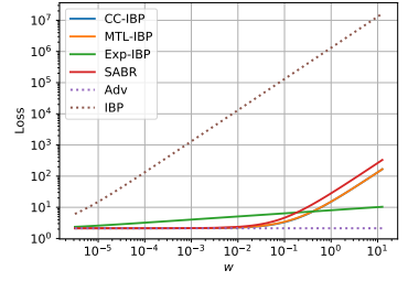
(a) 18 layers; \alpha = 10^{-5} for CC-IBP, MTL-IBP and SABR.
