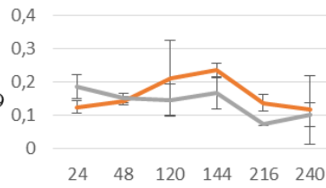
Unknown 19
