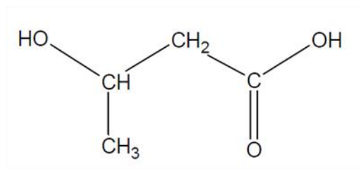
Figure 14. Acide 3-Hydroxybutyrique
