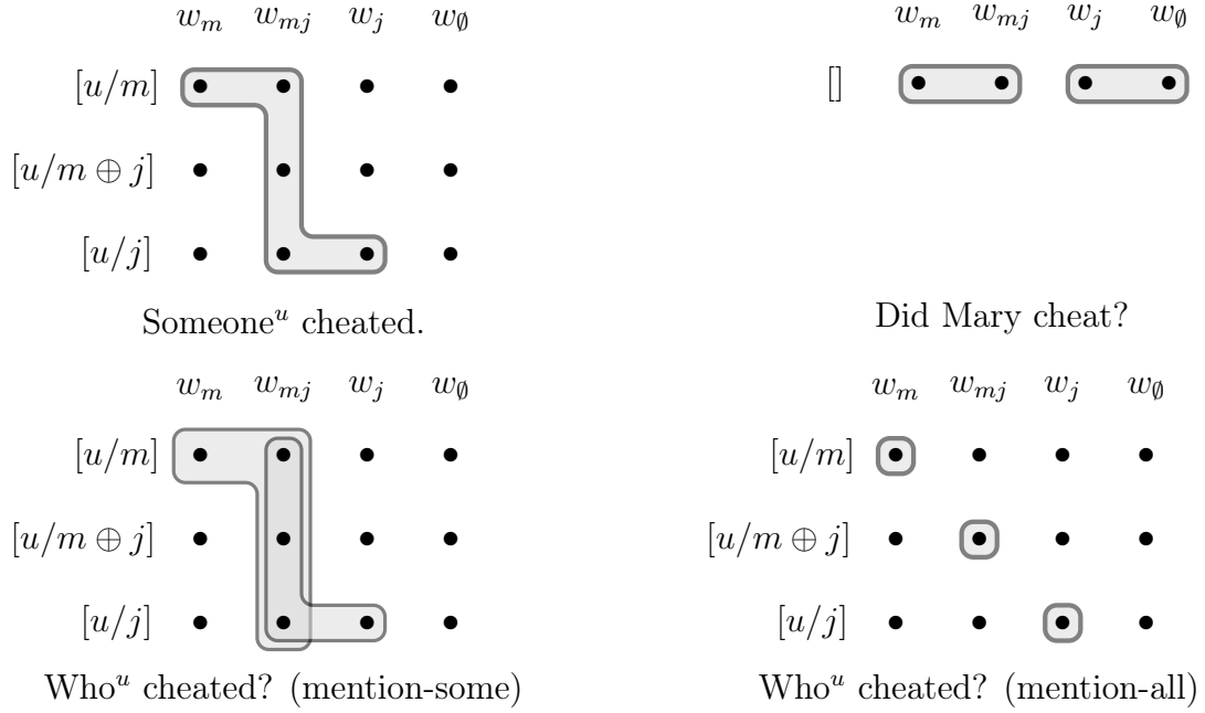
Figure 3.2 – Example sentences and their denotation in DInq.
