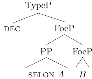
Figure 6.3 – Logical form of an assertive adjunct dependence utterance \text{selon}(A, B) .
