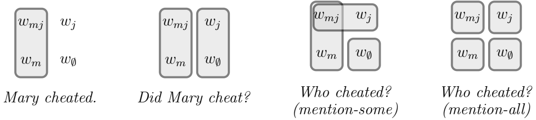
Figure 3.1 – Example sentences and their denotation in inquisitive semantics.
