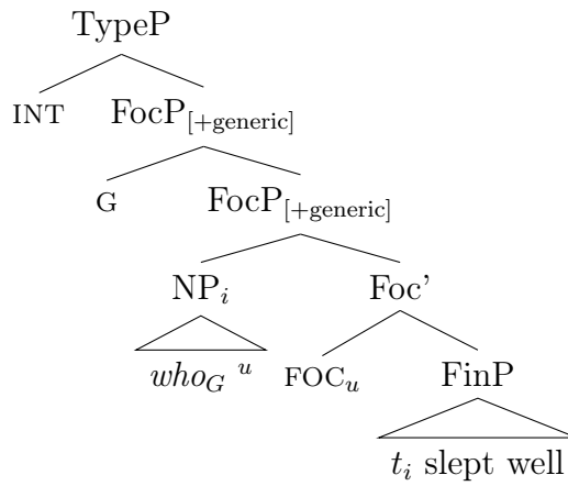
Figure 5.1 – Logical form of (29) before reconstruction.
