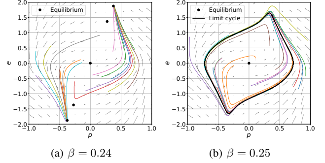
Fig. 2: Phase portraits for two value of \beta and \gamma = 0.2 . The system passes from 5 equilibria for \beta = 0.24 to 1 equilibrium with a stable limit cycle for \beta = 0.25 .
