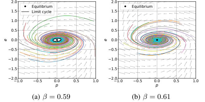
Fig. 3: Phase portraits for two value of \beta and \gamma = 0.2 . The stable limit cycle for \beta = 0.59 collapses into an equilibrium at \beta = 0.61 illustrating the Hopf bifurcation of Figure 1.
