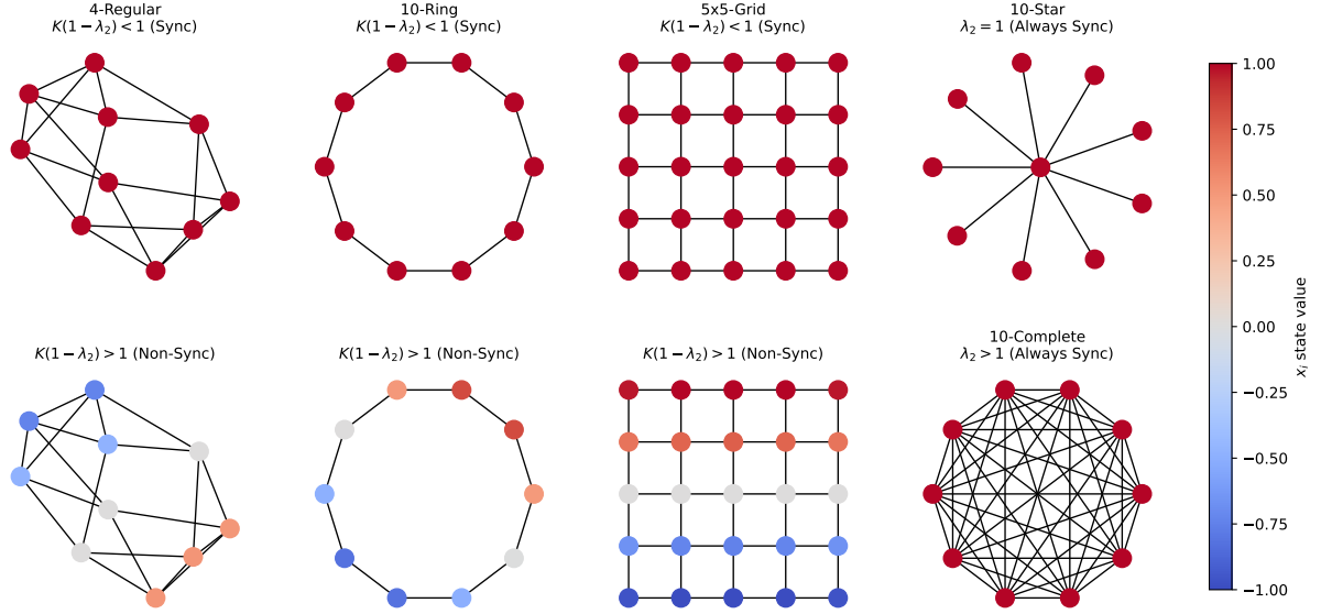
Figure 4.4: Asymptotic behavior of (COSA) on various graph topologies under different conditions for the synchronization parameter K(1 - \lambda_2) . Node colors represent the agent state x_i \in [-1, 1] , as indicated by the color bar. For each graph topology in columns 1-3, the top panel shows the final state when K(1 - \lambda_2) < 1 , resulting in global synchronization (Theorem 4.5.1). The bottom panel shows the final state for the same graph topology when K(1 - \lambda_2) > 1 , using a signal function s(x) that facilitates non-synchronized equilibria (Theorem 4.4.1), leading to persistent disagreement patterns. (Column 1) 4-Regular graph ( N = 10 , \lambda_2 \approx 0.42 ): (Top) K_1 = 2.6 . (Bottom) K_2 = 2.7 . (Column 2) 10-Ring graph ( N = 10 , \lambda_2 \approx 0.19 ): (Top) K_1 = 1.1 . (Bottom) K_2 = 1.3 . (Column 3) 5x5-Grid graph ( N = 25 , \lambda_2 \approx 0.11 ): (Top) K_1 = 1.1 . (Bottom) K_2 = 1.4 . (Column 4) Graphs with strong synchronizing properties: (Top) 10-Star graph ( N = 10 , \lambda_2 = 1 ), always synchronizes. (Bottom) 10-Complete graph ( N = 10 , \lambda_2 = N/(N - 1) > 1 ), always synchronizes due to high connectivity. Both are shown for parameters K = 50 still ensuring non fully synchronized equilibria. The signal function for both top and bottom panels is s(x) = \max(-1, \min(1, Kx)) . Initial condition are the same for both top and bottom panels and chosen to ensure non fully synchronized equilibria, and all simulations run until reaching a steady state.
