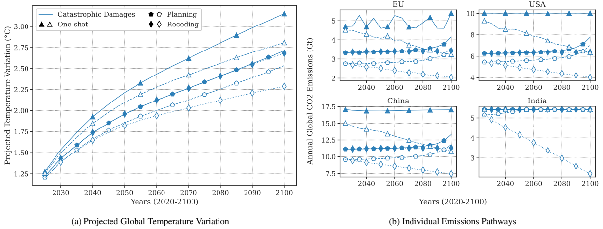
Figure 6: The Perils of Myopia and the Superiority of an Adaptive Policy Framework. All simulations are conducted under the Catastrophic damage function. (A) Projected global temperature variation for non-cooperative (NE, filled markers) and socially optimal (SO, open markers) equilibria under the three policy concepts. (B) The corresponding individual emissions pathways for four key players/blocs. The disastrous temperature outcomes of the One-shot concept are driven by the myopic, high-emission strategies of players like the USA and India. The Receding Horizon framework consistently yields the best environmental outcomes.
