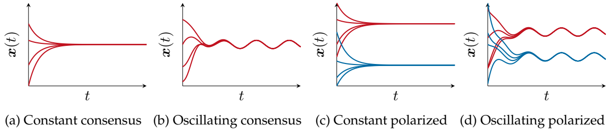
Figure 1.3: Initial observed dynamic behaviors of the coupled system.
