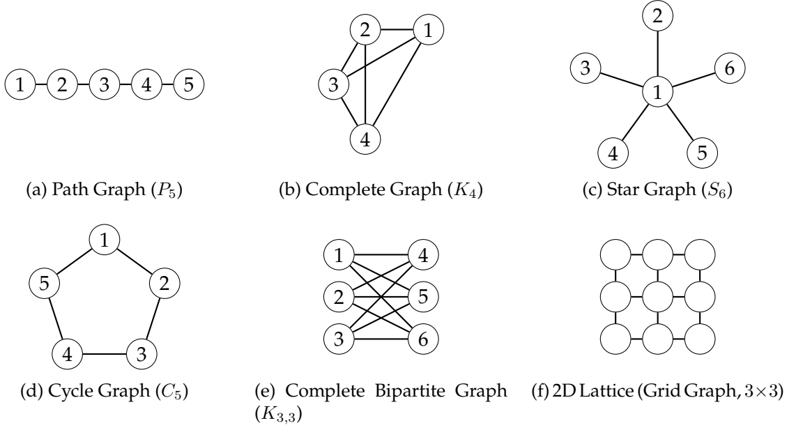
Figure 2.3: Illustrations of Canonical Graph Structures.
