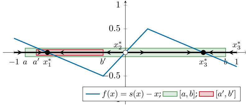
Figure 3.2: Illustration of the scalar dynamics \dot{x} = s(x) - x for the signal function s(x) = 0.7 \max(-1, \min(5x, 1)) . Equilibria are at the intersections (x_1^*, x_2^*, x_3^*) . The vector field f(x) = s(x) - x (indicated by arrows on the horizontal axis) shows the direction of movement. We present some invariant intervals of the dynamics to illustrate Proposition 3.5.5.
