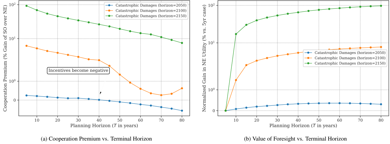
Figure 5: Economic Incentives are Exponentially Sensitive to the Terminal Time Horizon. Both panels plot outcomes in the Catastrophic Damages world for games ending in 2050, 2100, and 2150. Note the logarithmic scale on the y-axis. (a) The Cooperation Premium (percentage gain of SO over NE) is negligible for a 2050 horizon, significant for 2100, and an order of magnitude larger for 2150. (b) Similarly, the private economic value of long-term planning (normalized gain in NE utility) is close to zero for a 2050 horizon but becomes immense when the horizon is extended to 2150.
