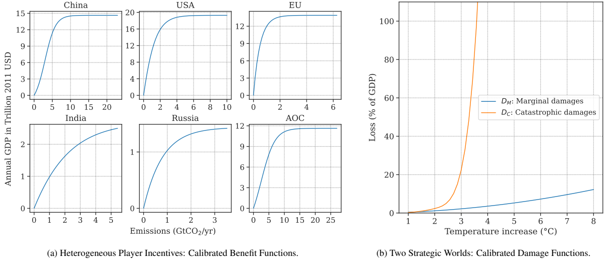
Figure 1: Core components of the game-theoretic model. (a) The calibrated benefit functions for the six players/regions, based on (11). The diverse shapes, from the sharply concave, post-industrial profiles of the USA and EU to the extended growth profile of India, represent the heterogeneous economic incentives and development stages that drive strategic behavior. (b) The two archetypal damage functions that define the strategic worlds of the analysis. The Marginal Damages function (12) models a conventional world of smoothly increasing costs, while the Catastrophic damage function (13) models a world with a Tipping point dynamic, creating fundamentally different strategic scenarios.
