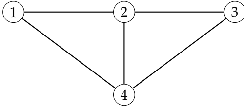
(a) A simple undirected, unweighted graph \mathcal{G}_1 with edges set \mathcal{E} = \{\{1, 2\}, \{2, 3\}, \{1, 4\}, \{2, 4\}, \{3, 4\}\} .
