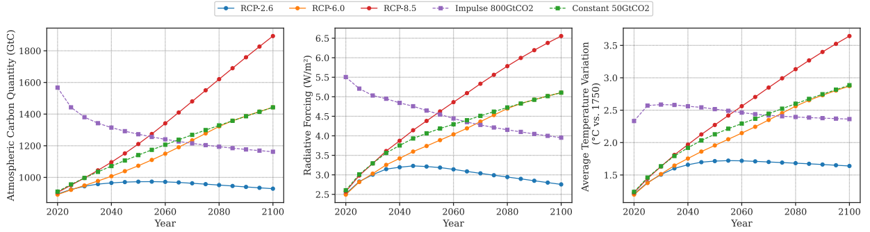
Figure 2: Validation of the SCM against standard climate scenarios. The three panels show the calibrated SCM’s response under standard emissions trajectories, including the IPCC’s Representative Concentration Pathway (RCP). The model correctly reproduces the key dynamic relationships between atmospheric carbon concentration (left), radiative forcing (middle), and global mean temperature anomaly (right). The consistency of these projections with established climate science benchmarks validates the SCM as a credible physical foundation for the strategic analysis.
