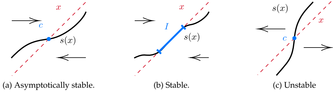
Figure 4.2: Illustration of the local stability conditions for synchronization equilibria as described in Theorem 4.3.1. The red dashed line represents the identity function y = x , and the blue curve represents the signal function s(x) . Fixed points (intersections) are marked with blue circles. Arrows on the x -axis indicate the direction of change in the scalar dynamics \dot{x} = s(x) - x .
