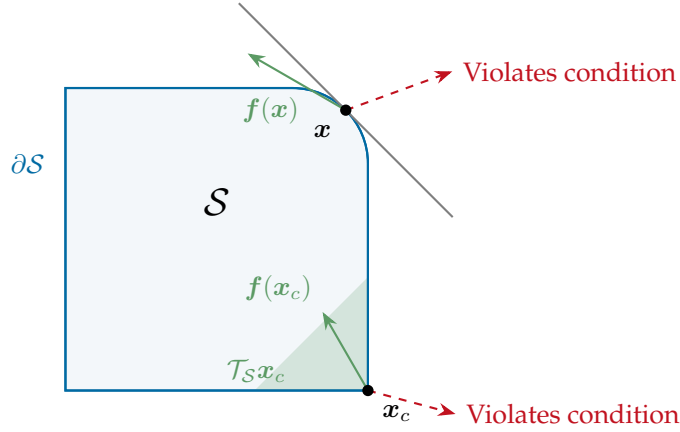
Figure 2.7: Illustration of Nagumo's condition for a set \mathcal{S} \subseteq \mathcal{X} with a smooth boundary and a sharp corner. For invariance, the vector field f(x) must belong to the tangent cone \mathcal{T}_S x at every boundary point x \in \partial\mathcal{S} . The red dashed vector are examples of vectors that violates the condition.i.e., a dynamical system with a vector field that is not in the tangent cone at a boundary point will not make the set forward invariant.
