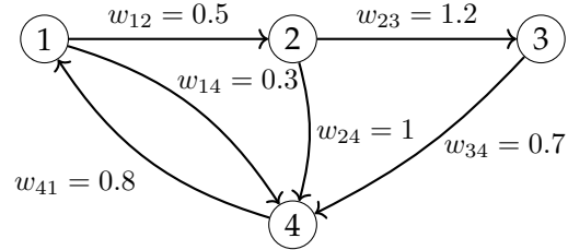
(b) A simple weighted directed graph (digraph) \mathcal{G}_2 with edges set \mathcal{E} = \{(1, 2), (2, 3), (1, 4), (2, 4), (3, 4), (4, 1)\} and weights w_{ij} .
