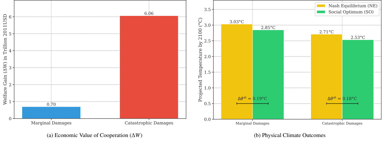
Figure 3: The Cooperation Dividend is Endogenous to Perceived Climate Damage. All simulations use the Planning framework to isolate the effect of the damage function. (a) The global welfare gain ( \Delta W ) realized by moving from the NE to the SO. The benefit of transitioning from non-cooperative (NE) to social-optimum (SO) behavior is most pronounced in a high-risk scenario, where the welfare dividend is nearly an order of magnitude greater. (b) The absolute temperature outcomes by 2100, showing that perceived climate damage induces greater unilateral abatement even in the non-cooperative equilibrium.
