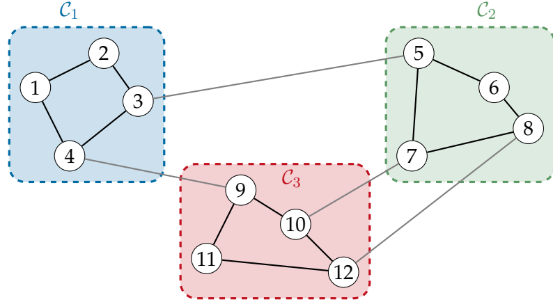
Figure 2.5: Illustration of a graph partition. A graph \mathcal{G} is partitioned into three disjoint cells \mathcal{C}_1 = \{1, 2, 3, 4\} , \mathcal{C}_2 = \{5, 6, 7, 8\} , and \mathcal{C}_3 = \{9, 10, 11, 12\} . Edges within cells are internal edges in black, while those connecting different cells are external edges in gray.
