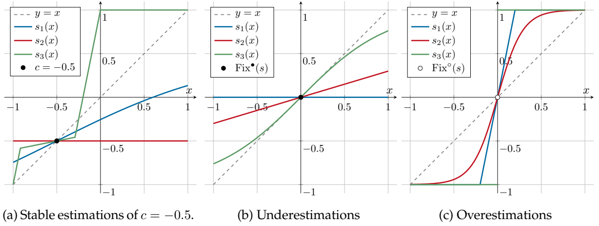
Figure 3.1: Examples of different signal functions s(x) classified as stable estimations, underestimations, and overestimations. An underestimation can be transformed into a stable estimation by translating and shifting the function s(x) by c . i.e., the function \tilde{s}(x) = s(x - c) - c for c to be a stable estimation of c .
