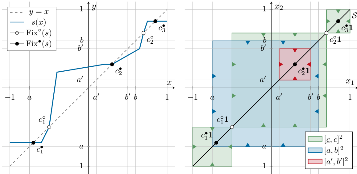
(a) A piecewise linear signal function s(x) with two unstable fixed points c_1^o and c_2^o and three stable fixed points c_1^* , c_2^* , and c_3^* . The shape of s hints the shape of the induced invariant hypercubes.
