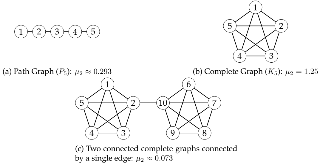
Figure 2.4: Examples illustrating varying algebraic connectivity. The P_5 graph is weakly connected, resulting in a small \lambda_2 . The K_5 graph is maximally connected, leading to a large \lambda_2 . The two connected complete graphs are connected by a single edge leading to the presence of a bottleneck and thus a really small \lambda_2 .
