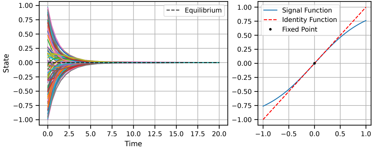
Figure 4.3: State evolution for agents with global underestimation signal over a connected graph (Erdős-Rényi with N = 100 and p = 0.1 ) with random uniform initial conditions and s(x) = \tanh(x) .
