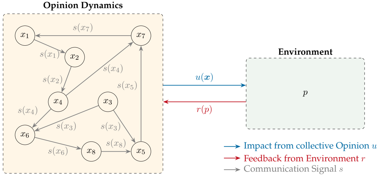
Figure 1.4: Diagram of the coupled dynamics. The opinion state of each agent is represented by the scalar x_i(t) and the environmental state is represented by the scalar p(t) . The opinion state of each agent is influenced by the environmental state through the function r(p(t)) and the environmental state is influenced by the opinion state of each agent through the function u(x(t)) .
