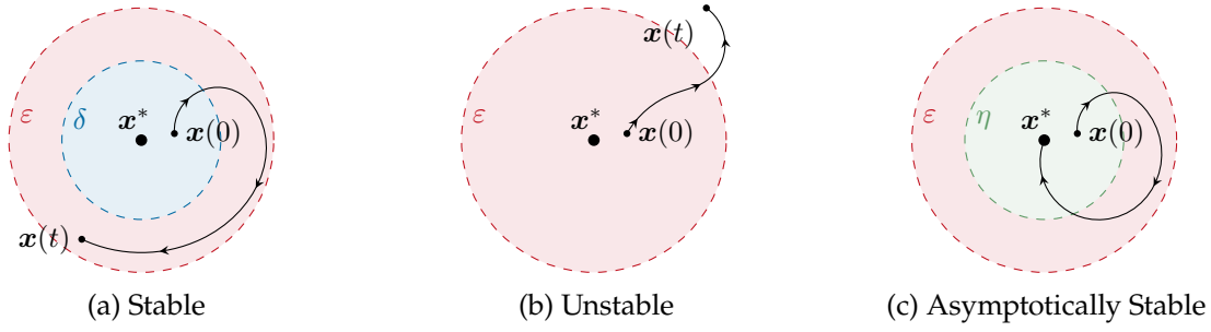
Figure 2.9: Visual representation of stability notions for an equilibrium point x^* . (a) A stable system: all the trajectories starting within \delta remain within \varepsilon . (b) An unstable system: trajectories starting within \varepsilon eventually leave \varepsilon . (c) An asymptotically stable system: trajectories starting within \eta converge to x^* .
