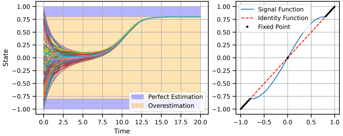
Figure 4.5: State evolution for agents with a globally overestimating signal under the same conditions as in Figure 4.3, s(x) = 0.8 \sin(2x) / \sin(1.6) for x \in [-0.8, 0.8] and s(x) = x otherwise.
