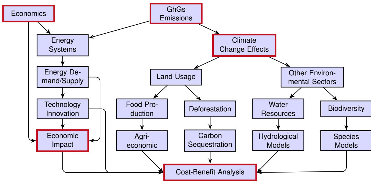
Figure 1.2: A schematic representation of an IAM possible structure illustrating their complexity and non-tractable nature.
