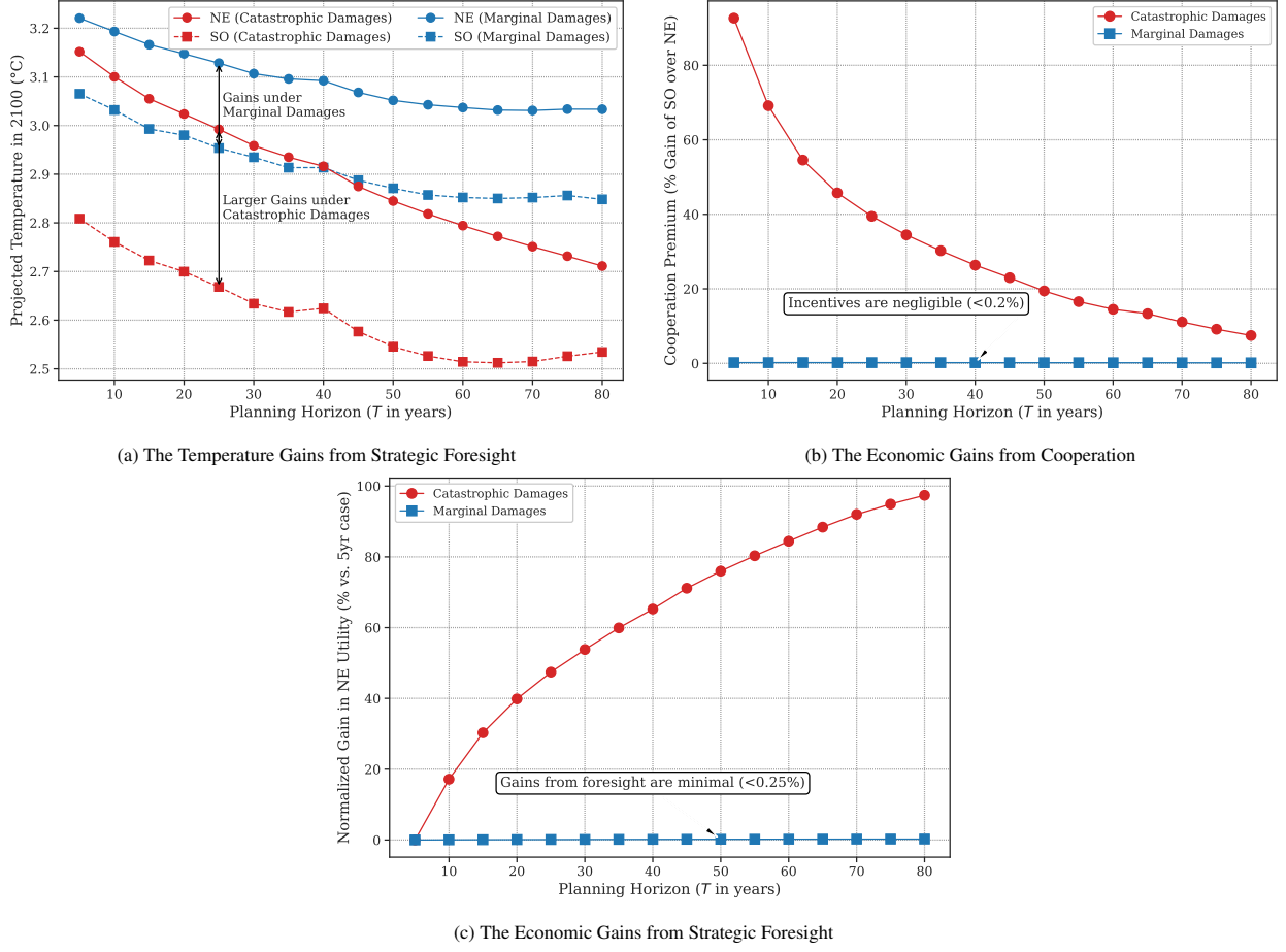
Figure 4: The Impact of Strategic Foresight ( T ) and Perceived Damage. All simulations use the Planning framework with a 2100 horizon. (a) Projected 2100 temperature for non-cooperative (NE, solid lines) and cooperative (SO, dashed lines) outcomes. (b) The “Cooperation Premium,” measured as the percentage gain in global welfare from achieving the SO over the NE. (c) The economic value of foresight, measured as the percentage gain in NE utility for a given horizon compared to a myopic one-stage ( T = 1 , i.e., 5-year) case. The plots demonstrate that perceived damage creates significant, non-negligible incentives for both foresight and cooperation. Specifically, governments have a strong incentive to adopt a long-term horizon (large T ) rather than relying on a sequence of successive short-term plans (small T ).
