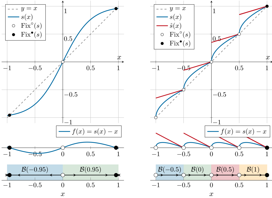
(a) Case s(x) = \tanh(2x) .
