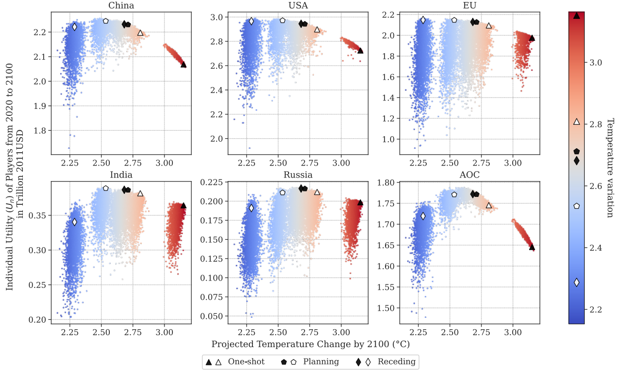
Figure 7: Individual Player Trade-offs Between Utility and Climate Outcomes. Each panel plots the total utility for a single player (y-axis) against the projected 2100 temperature (x-axis) under the Catastrophic damage scenario. The scatter plot shows the space of possible outcomes, with the color indicating the temperature. The six key equilibrium concepts are overlaid: NE (filled markers) and SO (open markers) for the One-shot (triangle), Planning (pentagon), and Receding Horizon (diamond) frameworks. The figure reveals the heterogeneous nature of the Free-Rider Problem , as the utility cost of achieving better climate outcomes varies significantly across players.
