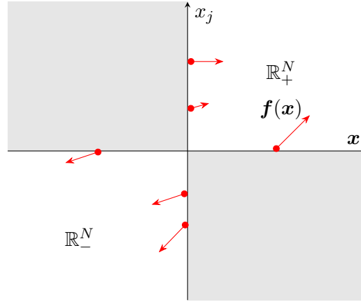
Figure 2.8: A cooperative system with a monotone flow. The red arrows represent the vector field of the system. The shaded regions represent the unordered orthant.
