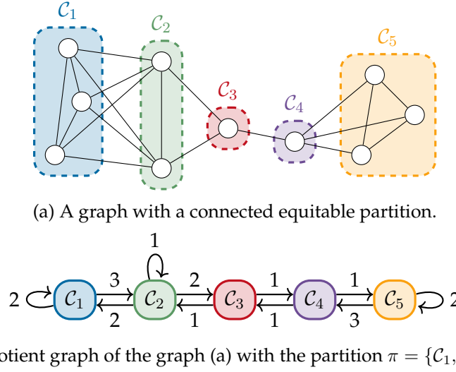
Figure 5.2: Example of a graph with equitable partition and its quotient graph.
