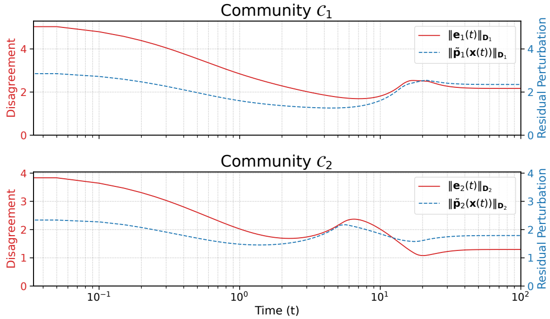
(b) ISS analysis for each community. For k \in \{1, 2\} , the internal disagreement \|e_k(t)\|_{D_k} (the ISS "state", in red) decays exponentially from its initial condition and converges to a non-zero ultimate bound. This bound is sustained by the persistent residual perturbation \|\tilde{p}_k(x(t))\|_{D_k} from the opposing cluster (the ISS "input," in blue), precisely as predicted by Theorem 5.4.1.
