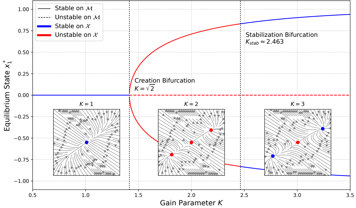
Figure 3.5: Bifurcation diagram for the N = 5 line graph, illustrating the distinction between stability on the invariant manifold \mathcal{M} and stability in the full state space \mathcal{X} . The plot shows the equilibrium state x_1^* as a function of the gain parameter K . Stability on \mathcal{M} (lines) : The FSE at x_1^* = 0 loses stability at K = \sqrt{2} (dashed line), creating two branches of NFSE that are stable on the manifold (solid lines). Stability in \mathcal{X} (red/blue colors) : The FSE becomes unstable in the full space at K = \sqrt{2} (red dashed line). Crucially, the new NFSE branches are also born unstable in \mathcal{X} (solid red lines), despite their stability on \mathcal{M} . They only become stable in the full space (solid blue lines) after the transversal stabilization bifurcation at K_{\text{stab}} \approx 2.463 . The inset phase portraits visualize the dynamics (3.11) on \mathcal{M} at three representative values of K .
