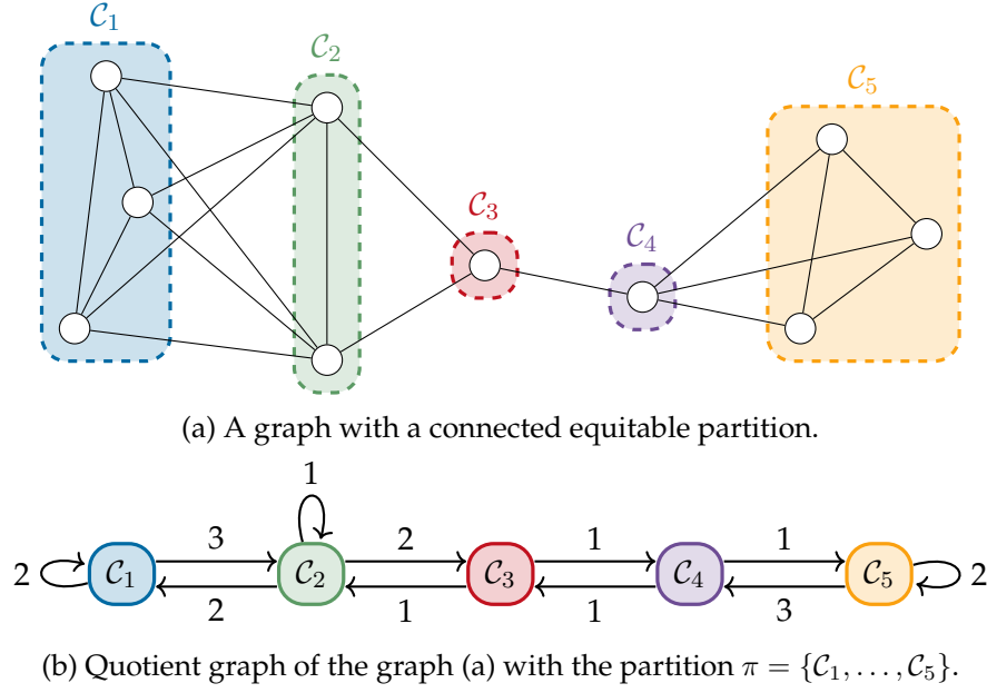
Figure 2.6: Example of a graph with equitable partition and its quotient graph.
