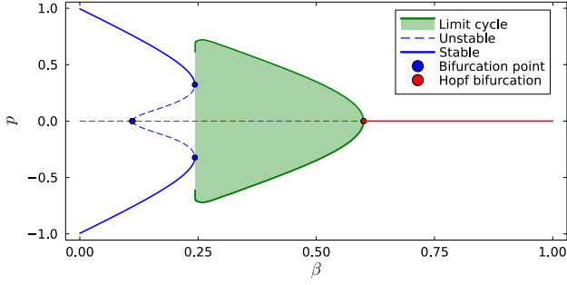
Fig. 1: Bifurcation diagram for the FSO dynamics (4a) with \gamma = 0.2 . Solid lines denote stable equilibria, dashed lines denote unstable equilibria, dots mark bifurcation points, and the green region shows the amplitude of the stable limit cycle emerging from the Hopf bifurcation.
