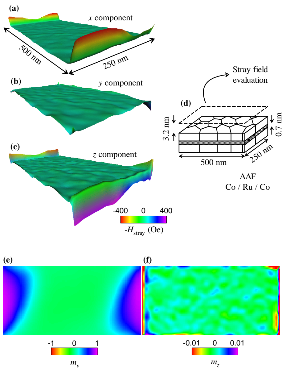
Figure 5.6: (Colour) Surface mapping of the AAF's stray field. (a)–(c) Field components. Both the colour code and the three-dimensional surface mapping correspond to the indicated component. (d) Stack schematics. (e)–(f) Remanent free Permalloy configuration. Note the highly expanded scale used for the m_z snapshot.
