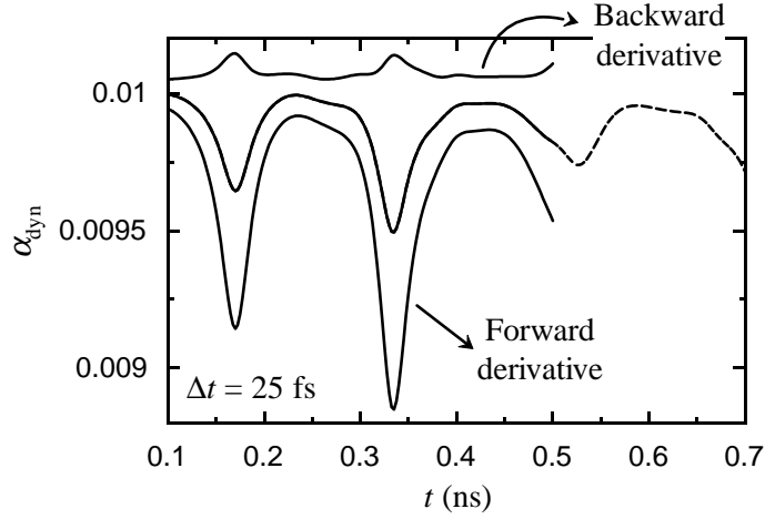
Figure A.6: First-order backward and forward \alpha_{dyn} values together with their average (dashed curve) and the second-order formula value (solid curve on top of the dashed one).
